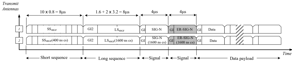
Figure 013 – MIMO-OFDM Training structure for N_{Tx} = 2 , 40 MHz, greenfield operation. The shaded field indicates the optional duplicate SIG-N for extended range communication.
