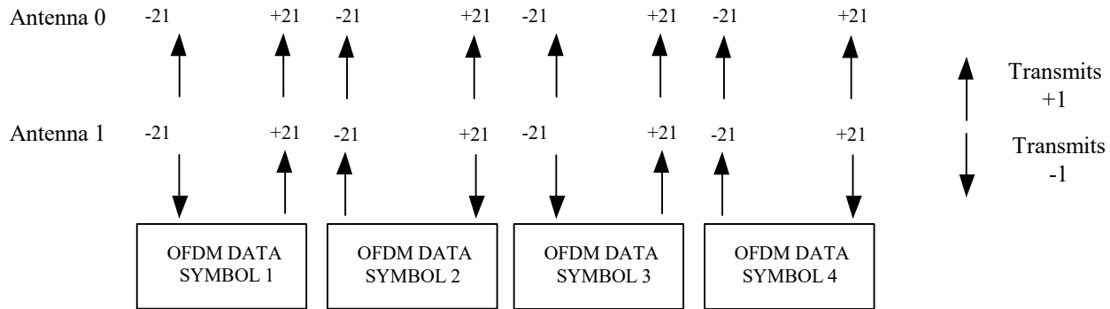
Figure 022 – An illustration of the relative polarity of pilot signals in the 20 MHz 2TX-SDM mode. “-21” and “+21” indicate the subcarrier indices on which pilot signals are sent
