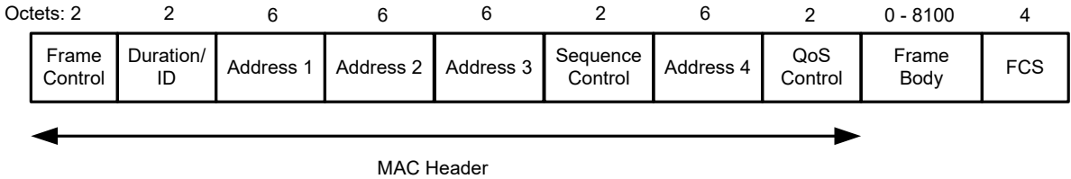
Figure 22 – Data frame
