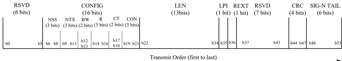
Figure 017 – SIG-N field bit assignment
