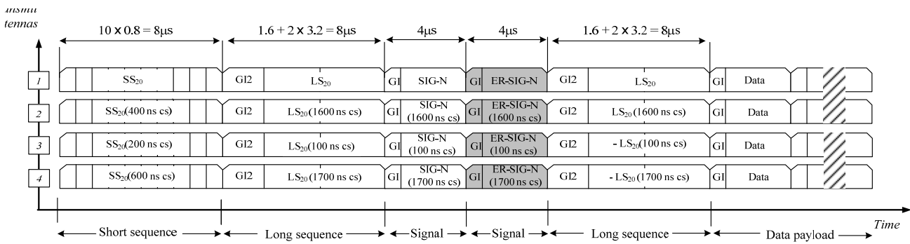
Figure 009 – MIMO-OFDM Training structure for N_{TX} = 3 and 4, 20 MHz, greenfield operation. The shaded field indicates the optional duplicate SIG-N for extended range communication.
