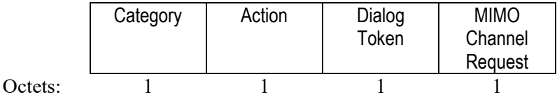
Figure 000n3- MIMO Channel Request frame format
