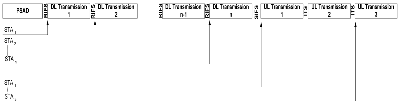
Figure 003n – HTP Burst transmission with Power Efficiency and ULT scheduling
