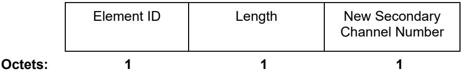
Figure 46u—New Secondary Number element format
