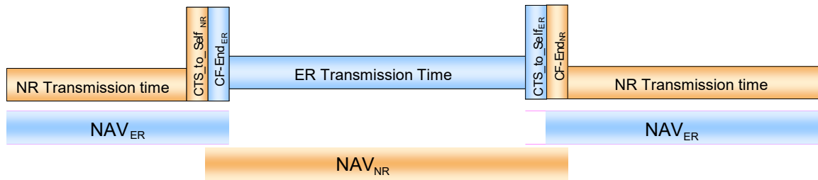
Figure xyz: Alternate ER/NR protection mechanism managed by AP
