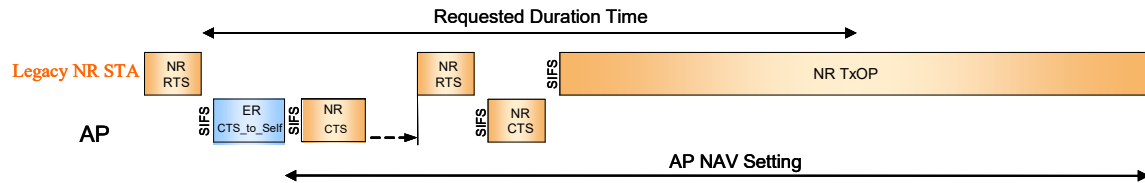
Figure xxyz5: Protection of an EDCA NR TxOP initiated by a non-AP legacy STA
