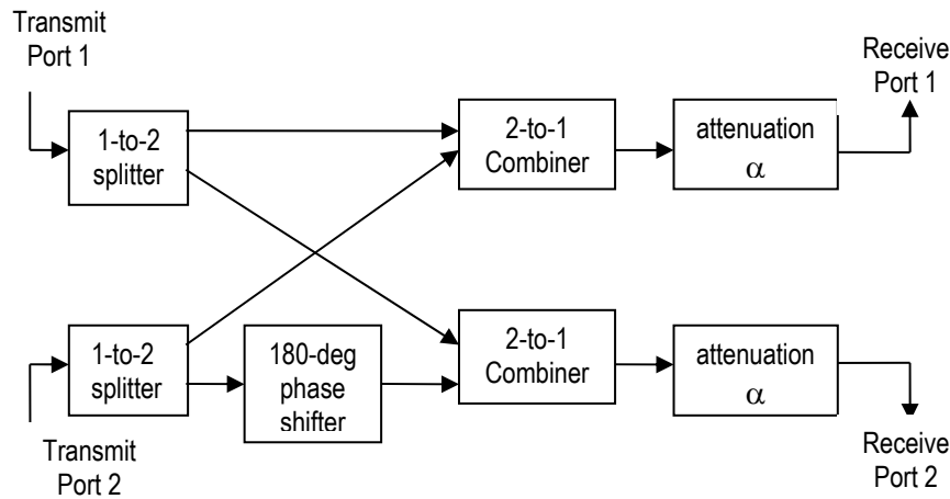
Figure 026 –EVM test setup
