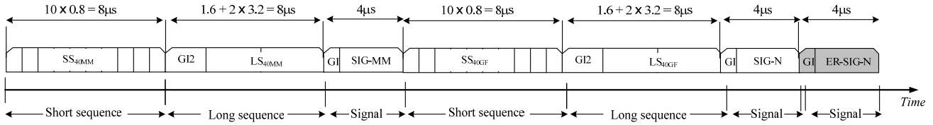
Figure 012 – MIMO-OFDM Training structure for N_{Tx}=1 , 40 MHz, mixed-mode operation. The shaded field indicates the optional duplicate SIG-N for extended range communication.
