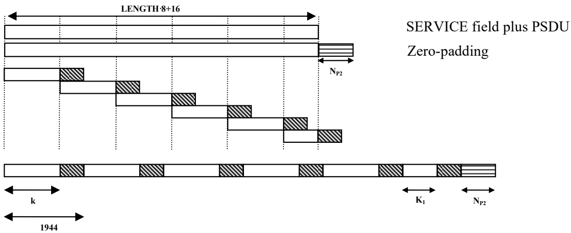
Figure 020 – LDPC PDU encoding.
