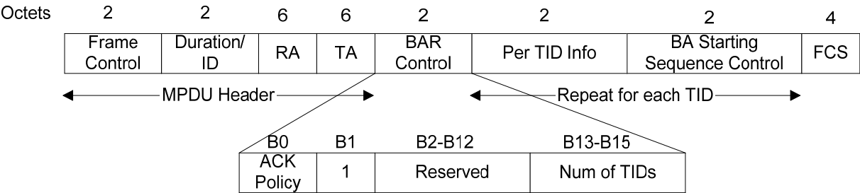
Figure x.y1 – HT Block ACK Request Frame Format
