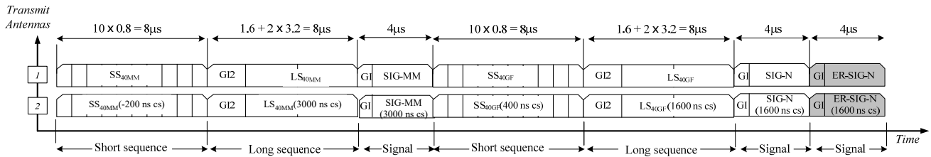
Figure 014 – MIMO-OFDM Training structure for N_{Tx} = 2 , 40 MHz, mixed-mode operation. The shaded field indicates the optional duplicate SIG-N for extended range communication.
