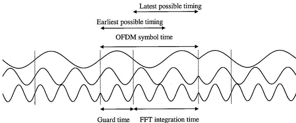
Figure 4.5 Example of an OFDM signal with three subcarriers, showing the earliest and latest possible symbol timing instants that do not cause ISI or ICI.
