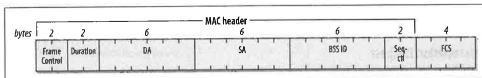
Figure 4-42. ATIM frame
