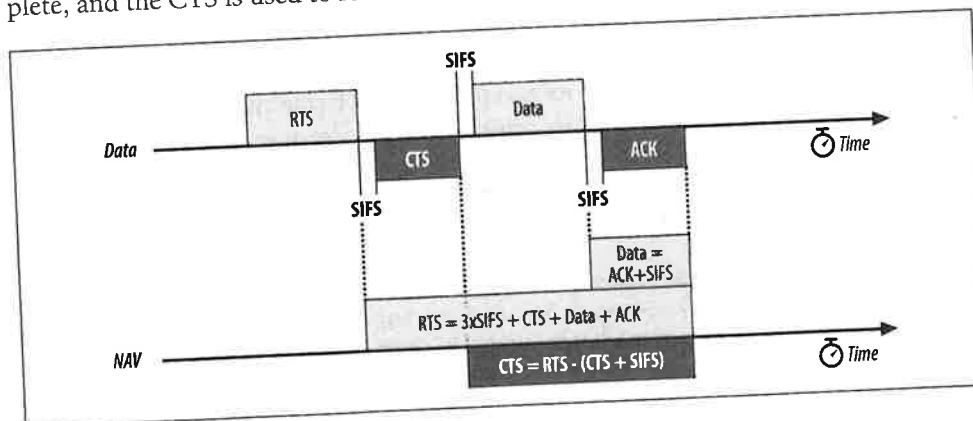
Figure 3-17. RTS/CTS lockout
