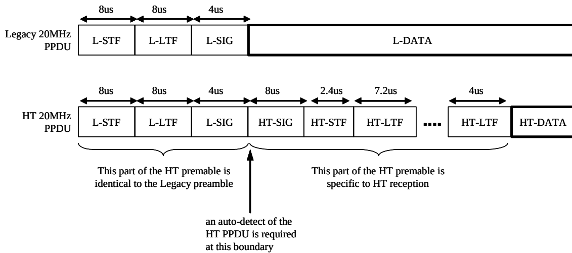
Figure 28: HT Preamble format
