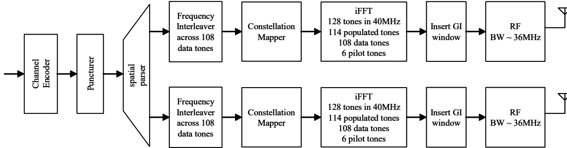
Figure 46: Transmitter datapath for 2-antenna MIMO in 40MHz 12
