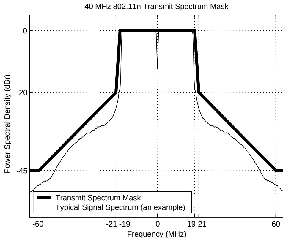
Figure 46: Transmit spectrum mask for 40MHz channelization
