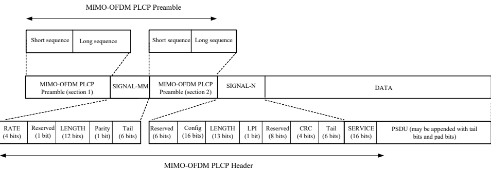
Figure 003 – PPDU frame format: Mixed-modeMixed-mode access in the 1TX (40 MHz) and 2TX (20 and 40 MHz) modes
