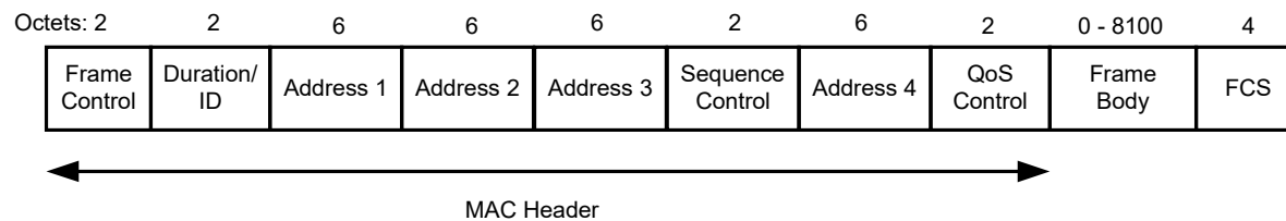
Figure 22 – Data frame
