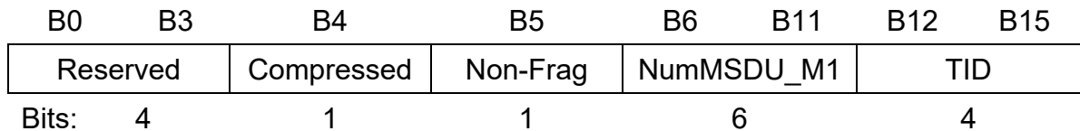
Figure 7 - BA Control field
