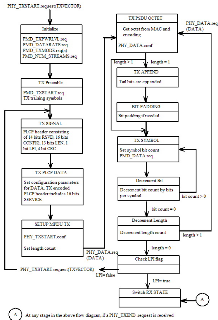
Figure 027 –PLCP transmit state machine
