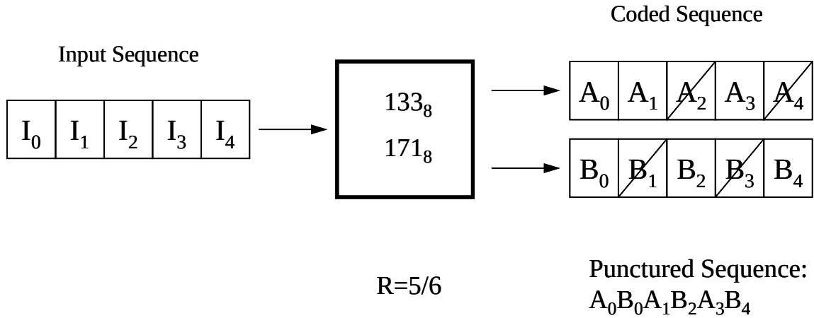
Figure 41: Puncturing pattern for code rate = 5/6
