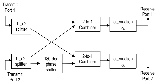
Figure 026 –EVM test setup
