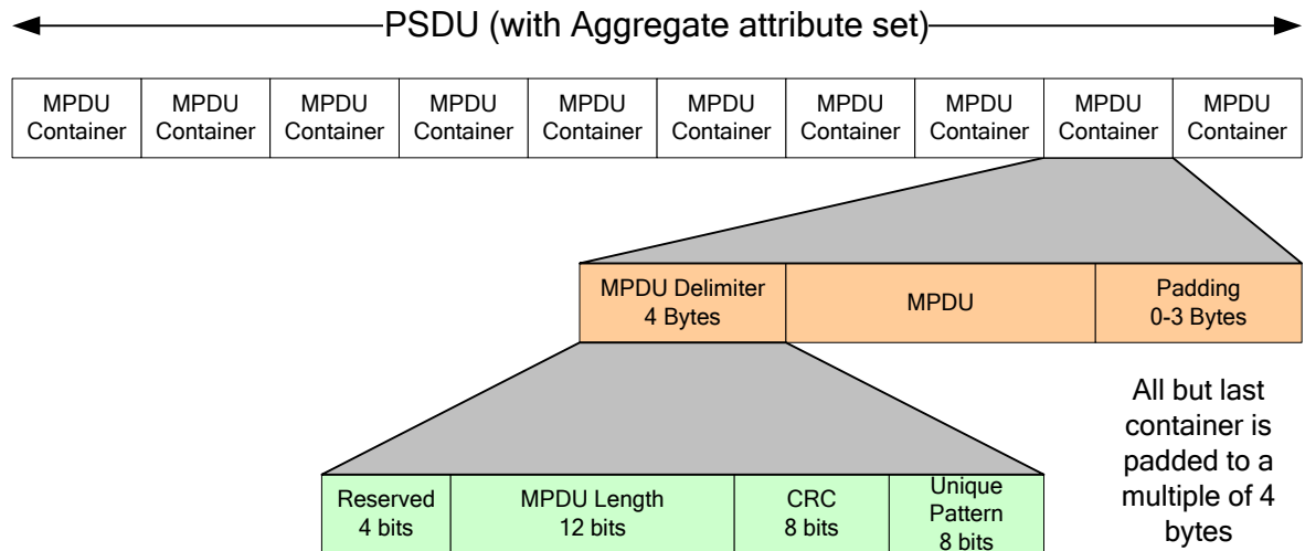
Figure 11 – A-MPDU format
