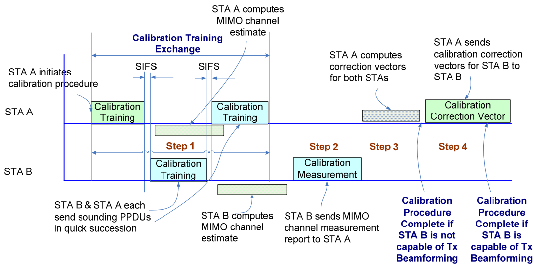
Figure 37 - Calibration Procedure
