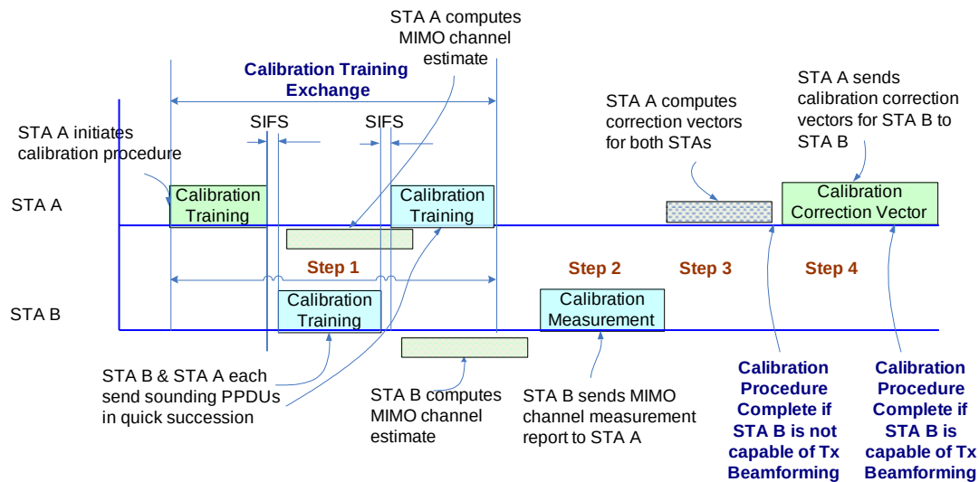
Figure 17: Calibration Procedure
