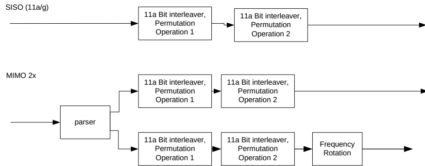
Figure 42: Structure of interleaver
