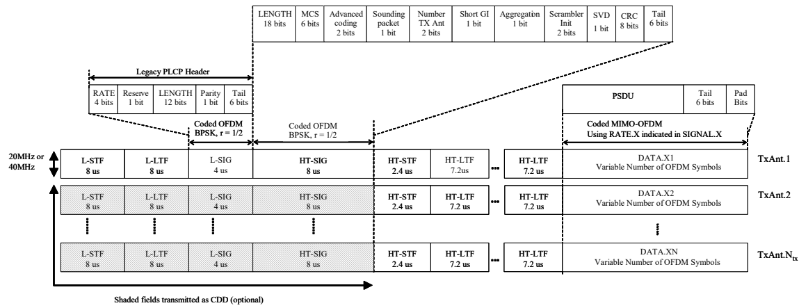
Figure 56: PPDUs format leveraging CDD transmission
