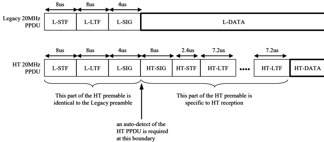
Figure 50: HT Preamble format
