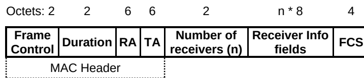
Figure 2 – MMP MPDU
