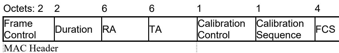
Figure 8 – Calibration Training MPDU
