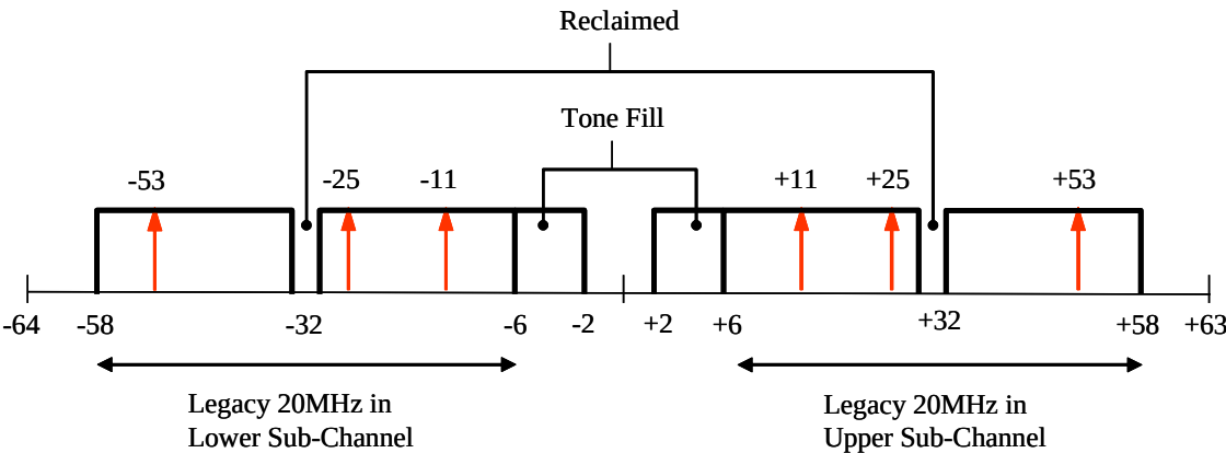
Figure 43: Tone Format for 40MHz channelization
