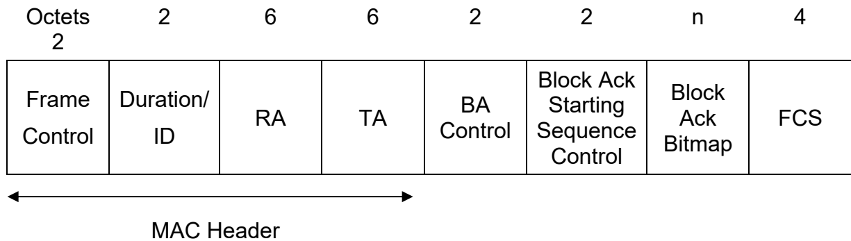
Figure 6 - Compressed BA MPDU
