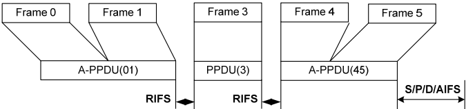
Figure 003n – HTP Burst transmission
