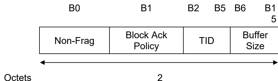
Figure 16 - Block Ack Parameter Set fixed field
