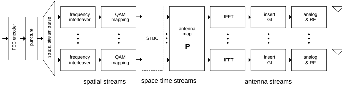
Figure 20: MIMO data path.
