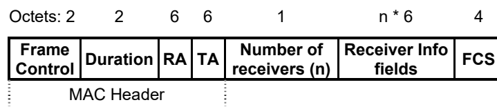
Figure 3 – MRAD MPDU
