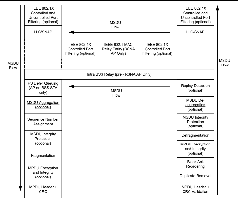
Figure 11g – MAC data plane architecture
