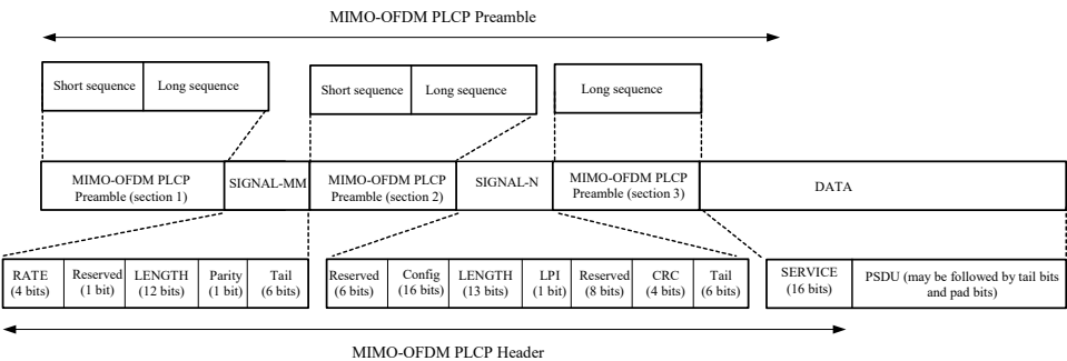
Figure 005– PPDU frame format: Mixed-modeMixed-mode access in the 3TX and 4TX modes (40 MHz)
