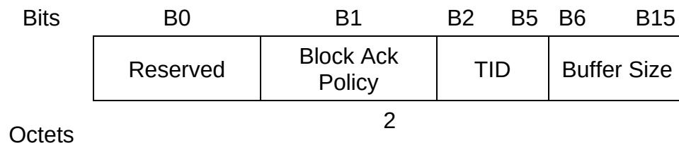
Figure 10 - Block Ack Parameter Set fixed field
