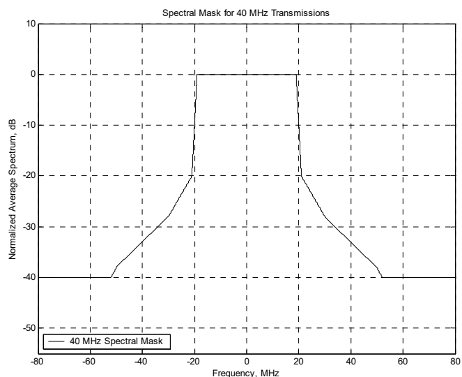
Figure 025 –Transmit spectrum mask for 40 MHz transmissions
