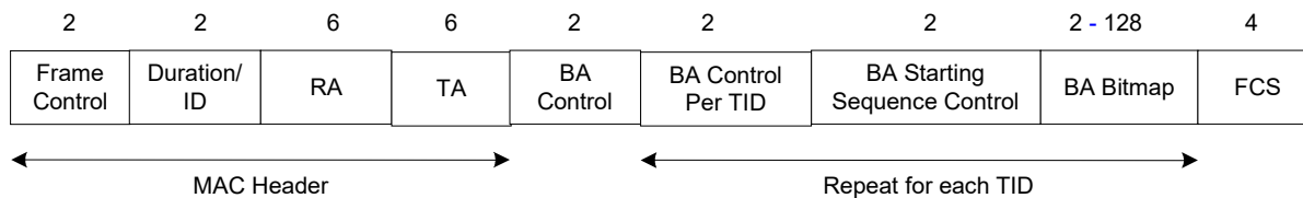
Figure x.y3 – HT Block ACK Frame Format
