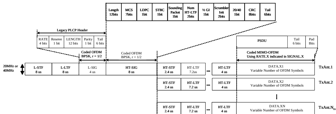
Figure 31: PPDU Format for N_{Tx} antennas
