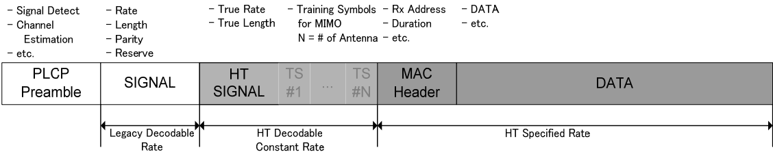
Figure 40 – PPDU Format with Legacy Protection
