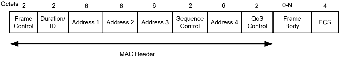
18 19 Figure 12 – MAC frame format
