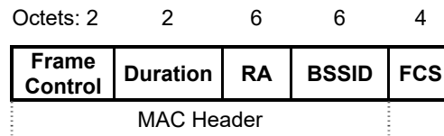
Figure 5 – DCB MPDU
