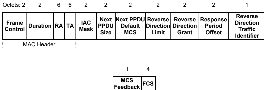
Figure 1 – IAC MPDU
