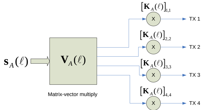
Figure 48: Application of calibration correction vector on Tx
