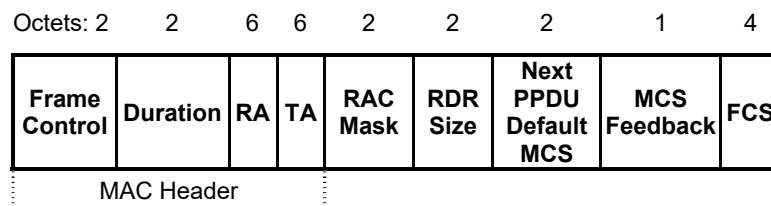
Figure 2 – RAC MPDU
