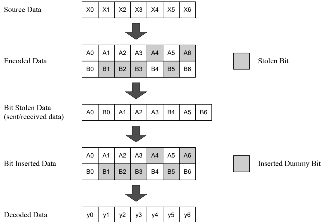
Figure 64: Puncturing pattern for code rate = 7/8
