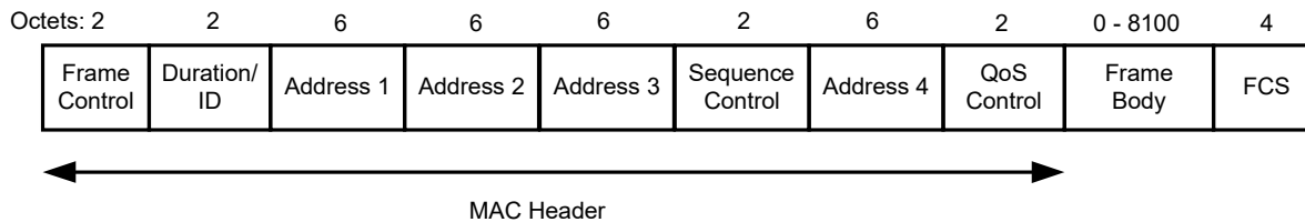
Figure 22 – Data frame
