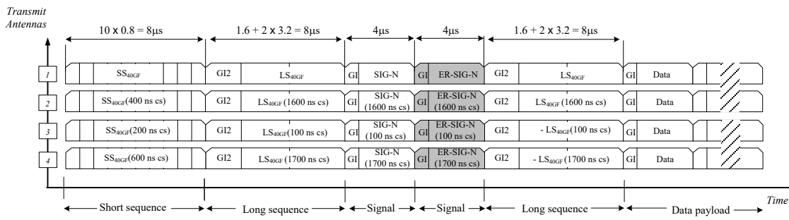
Figure 015 – MIMO-OFDM Training structure for N_{TX} = 3 and 4, 40 MHz, greenfield operation. The shaded field indicates the optional duplicate SIG-N for extended range communication.
