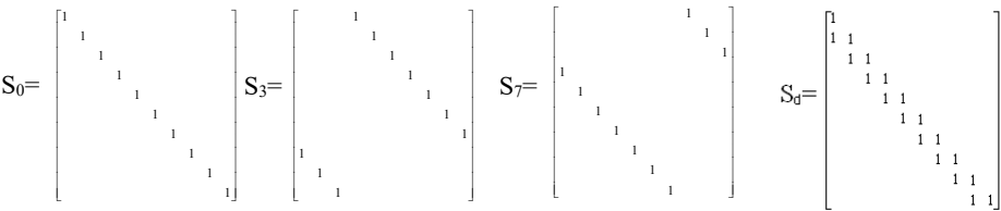
Figure 022 — Structure of the cyclic permutations of the identity matrix. Matrix S_i is produced by cyclically shifting the columns of the identity matrix to the right i places.
