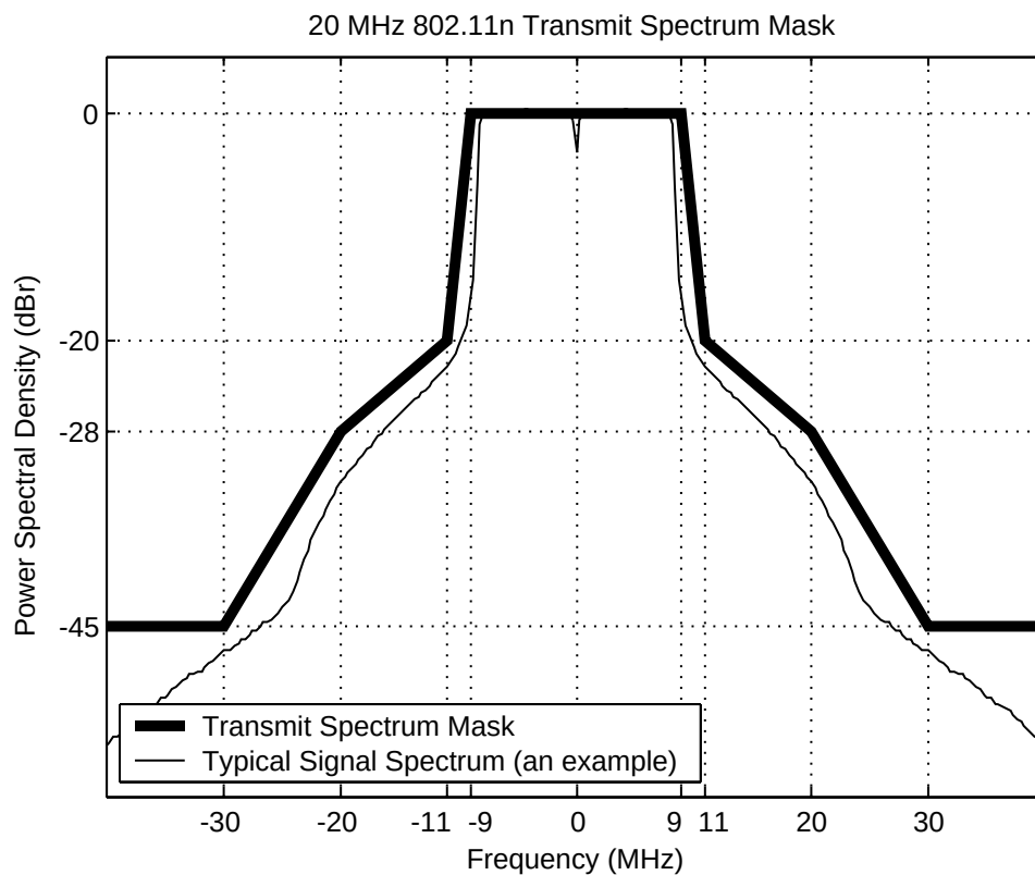
Figure 45: Transmit Spectrum Mask for 20MHz channelization
