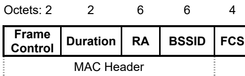
Figure 4 – ICB MPDU
