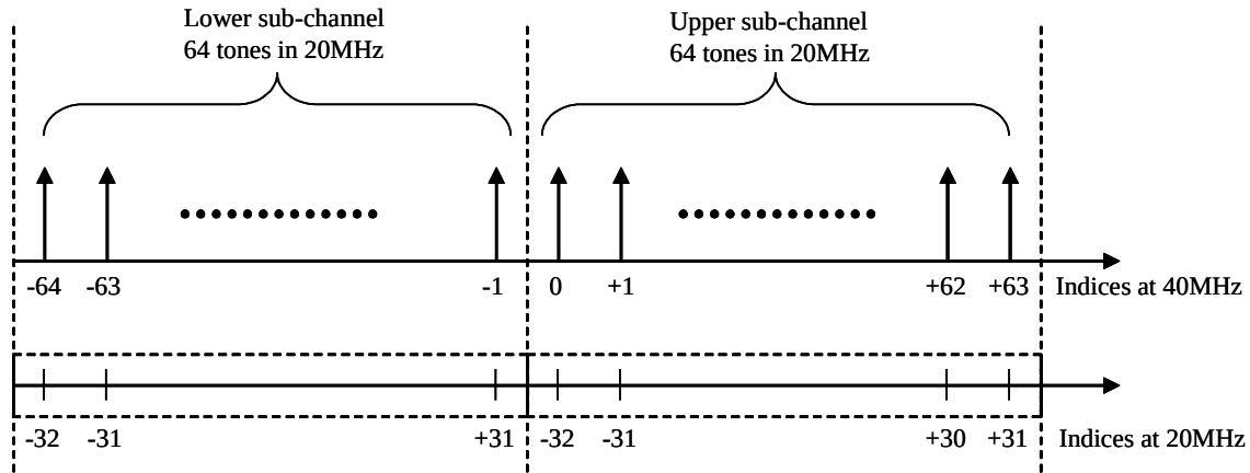
Figure 26: Upper and Lower sub-channel specification in 40MHz
