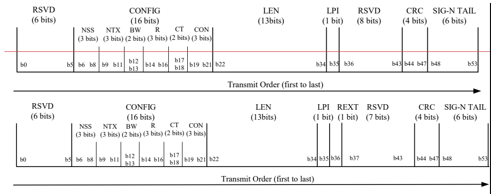
Figure 017 – SIG-N field bit assignment
