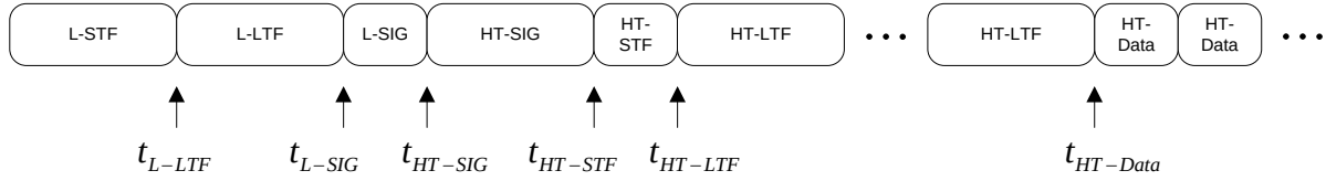
Figure 33: Timing boundaries for PPDU Fields
