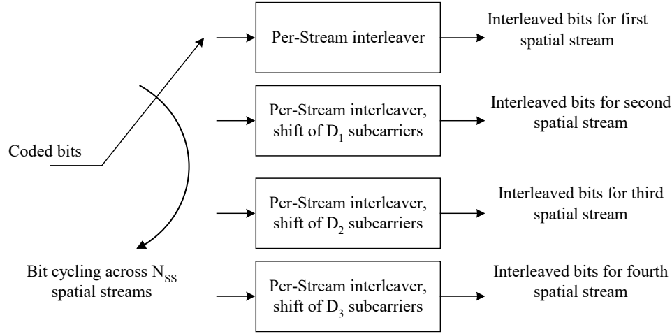
Figure 019 – Illustration of the interleaver function
