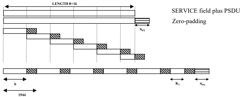
Figure 020 – LDPC PPDU encoding.
