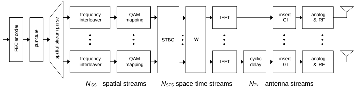
Figure 24: STBC with spatial spreading
