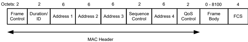
Figure 22 – Data frame
