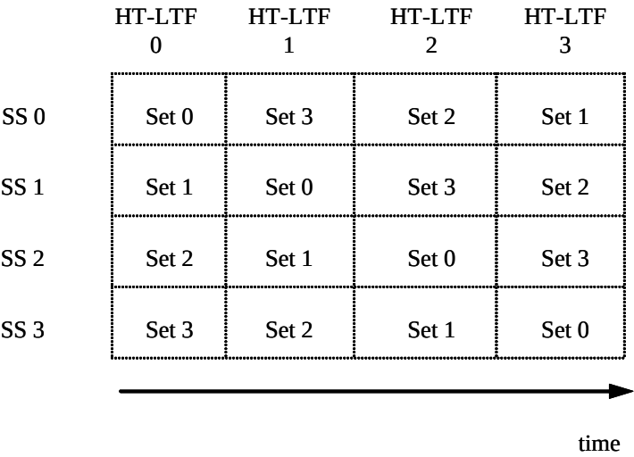
Figure 35: HT-LTF tone interleaving across 4 spatial streams
