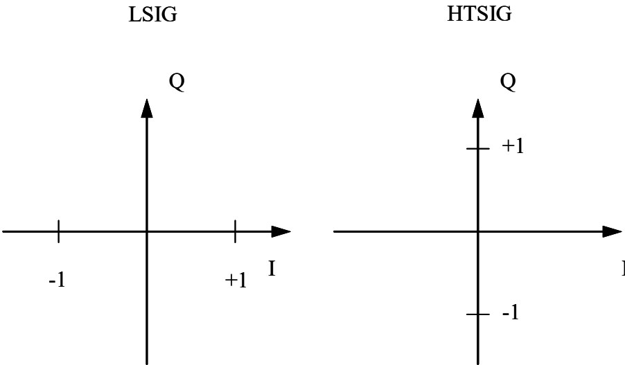
Figure 60: Constellation specification for LSIG and HTSIG
