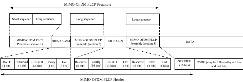
Figure 004– PPDU frame format: Mixed-modeMixed-mode access in the 3TX and 4TX modes (20 MHz)
