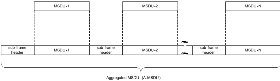
Figure 001n – Formation of an A-MSDU
