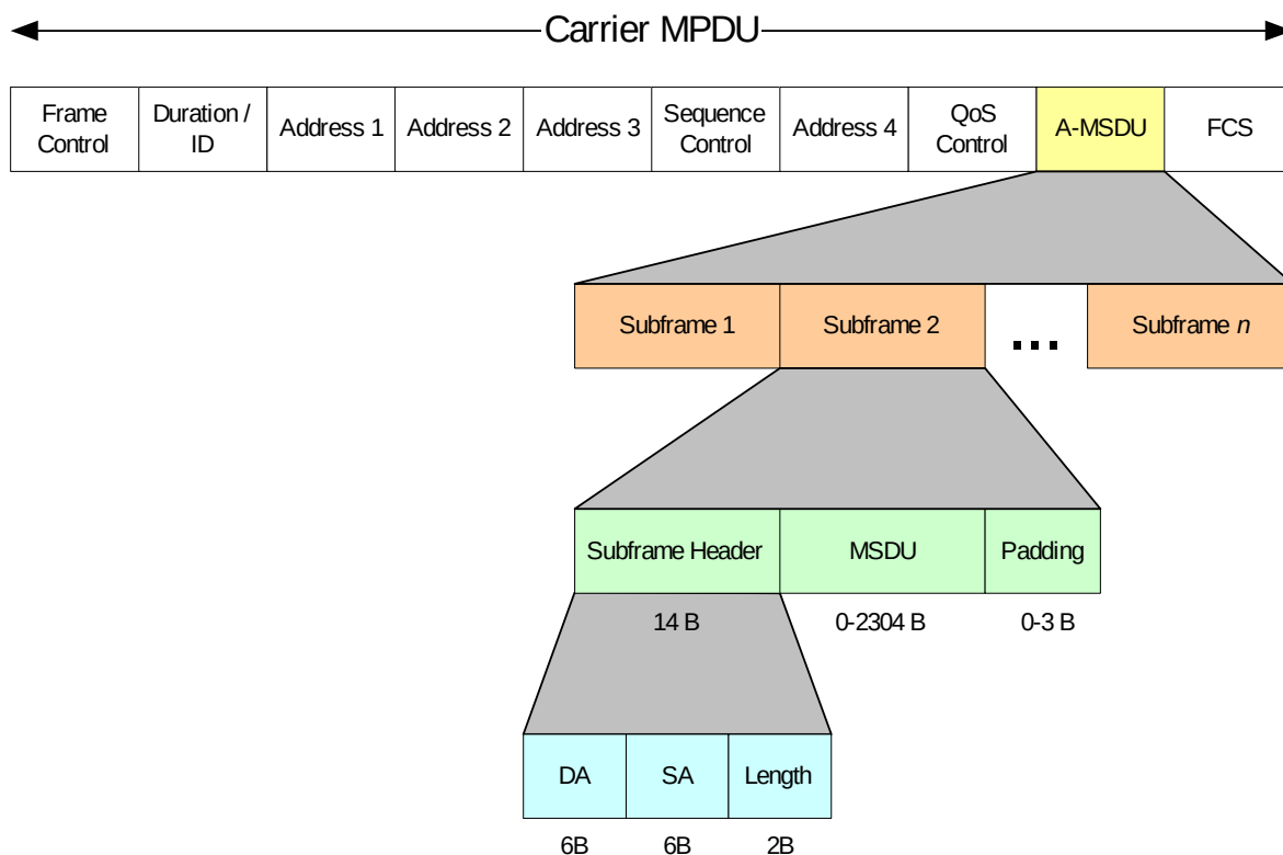
Figure 12: A-MSDU Strcuture
