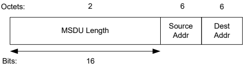
Figure 002n – Sub-Frame Header
