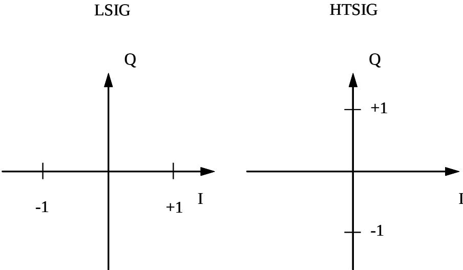
9 10 Figure 37: Constellation specification for LSIG and HTSIG
