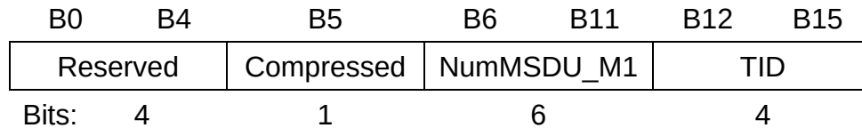
Figure 4 – BA Control field
