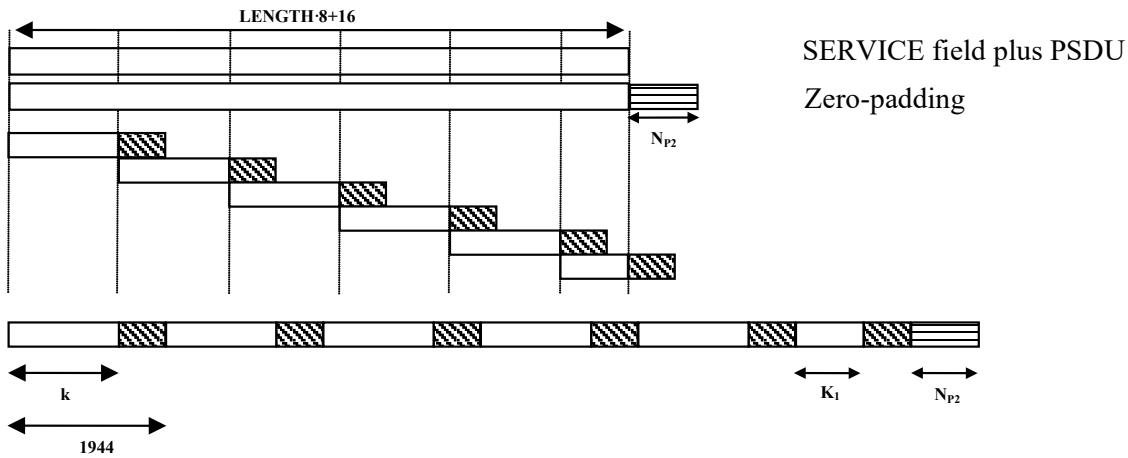
Figure 020 – LDPC PPDU encoding.
