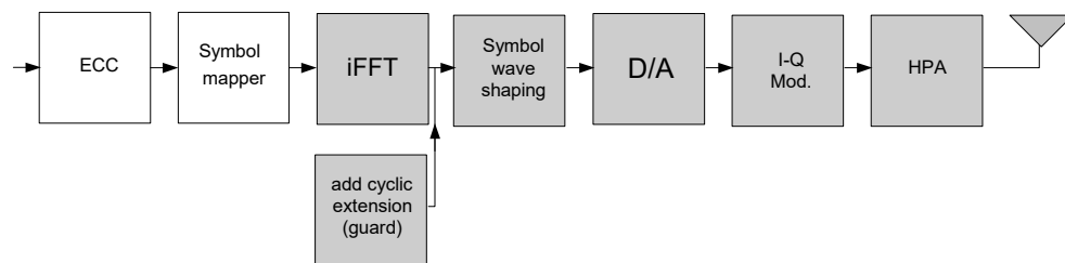
Figure 024 – Transmitter block diagram for the MIMO-OFDM PHY
