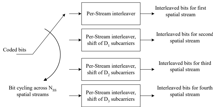
Figure 019 – Illustration of the interleaver function
