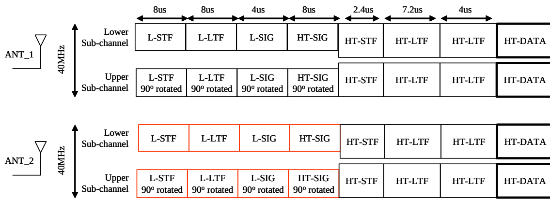
Figure 27: PPDU Format for 2x40 Basic MIMO Transmission 10
