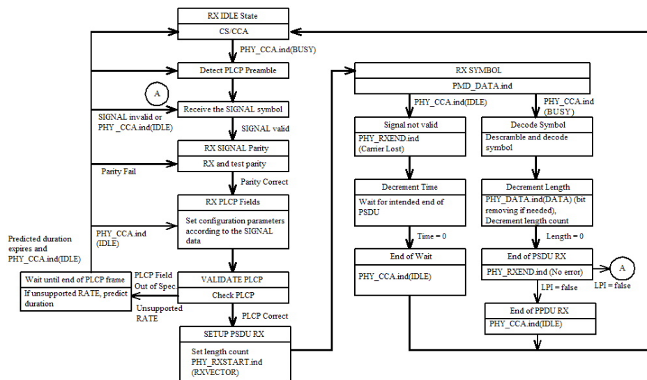
Figure 028 – PLCP receive state machine
