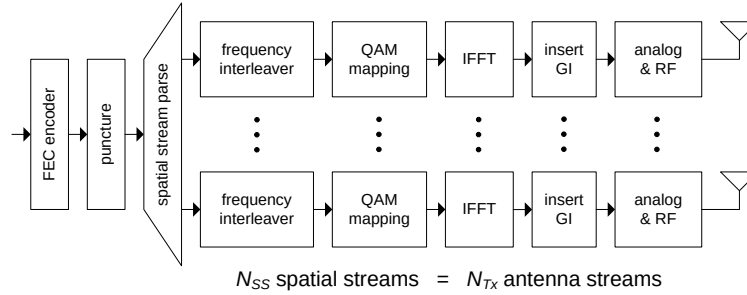
Figure 21: Direct Map MIMO.
