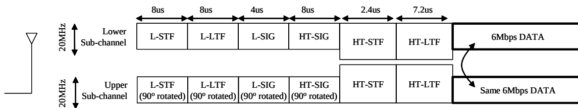
Figure 30: PPDU format for 6Mbps duplicate mode
