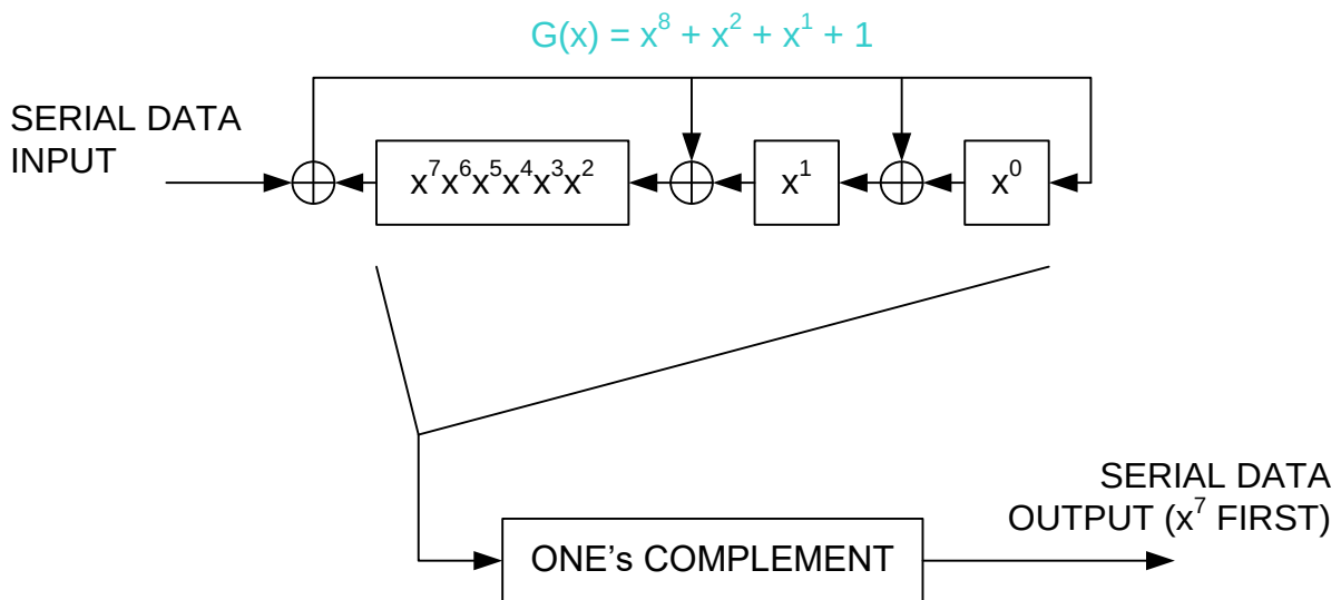
Figure 40: CRC8 implementation
