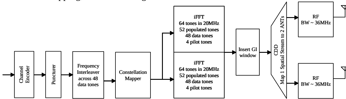
Figure 29: Transmitter configuration for 6Mbps in 40MHz 11
