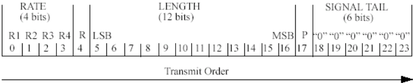
14 15 Figure 38: SIGNAL field bit assignment
