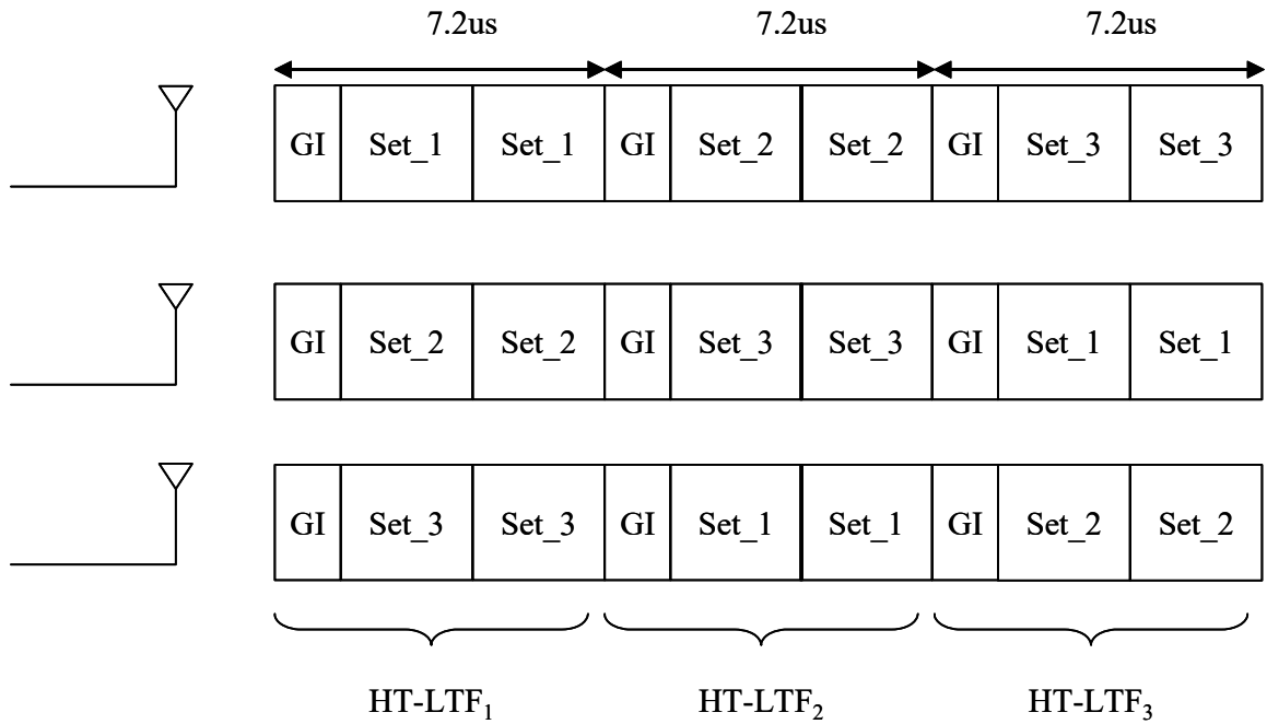
Figure 58: HT-LTF pattern for 3 antennas (3 spatial streams)
