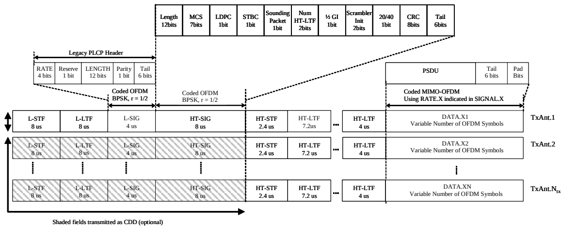
Figure 32: PPDU format leveraging CDD transmission
