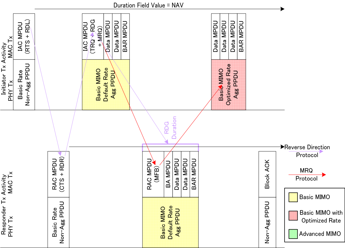
Figure 27 – LongNAV Bi-Directional Example
