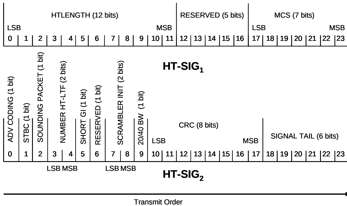
Figure 39: HT-SIG field bit assignments
