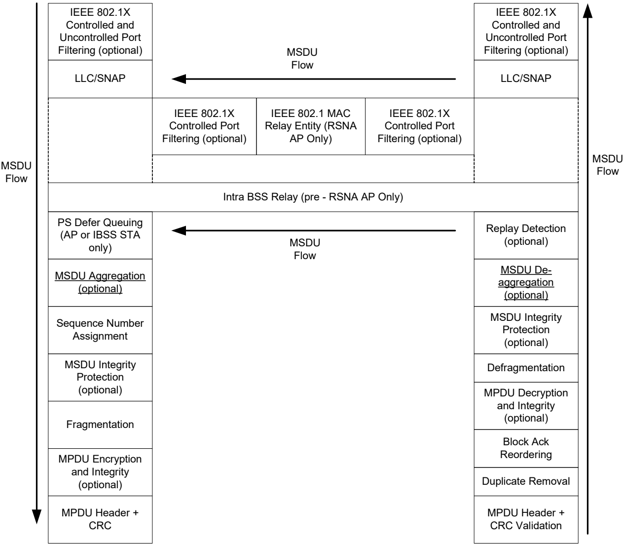
Figure 11g – MAC data plane architecture
