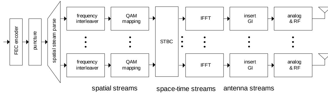
Figure 23: STBC with direct map MIMO
