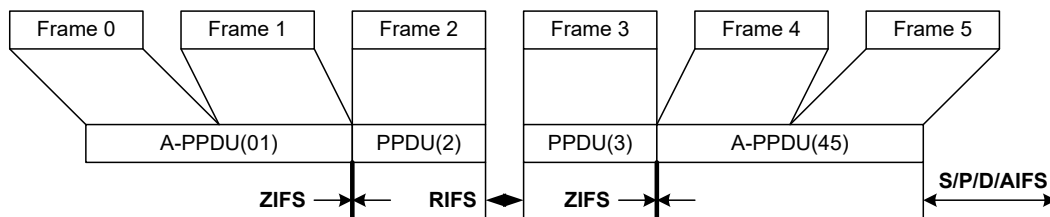
Figure 003n – HTP Burst transmission
