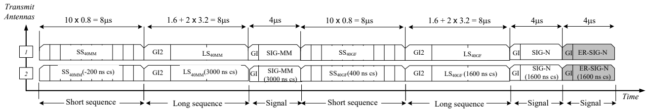
Figure 014 – MIMO-OFDM Training structure for N_{TX} = 2 , 40 MHz, mixed-mode operation. The shaded field indicates the optional duplicate SIG-N for extended range communication.
