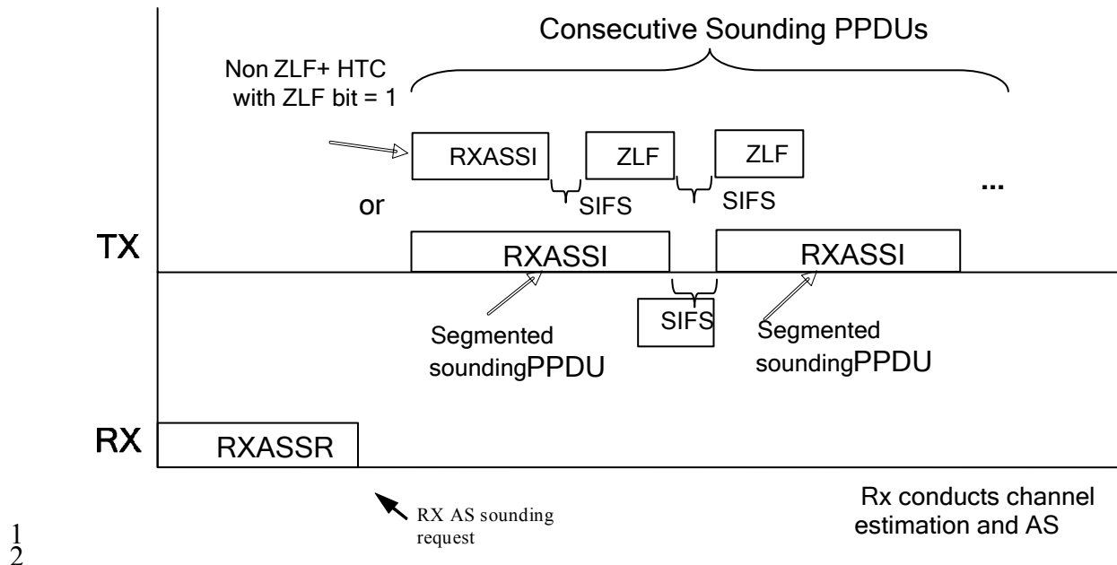
Figure n47 – Frame Exchange Sequence of Receive Antenna Selection
