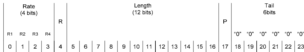
Figure n52 - The signal field
