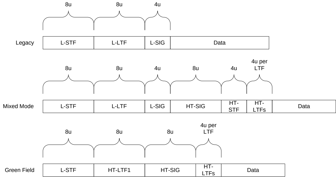
Figure n49- PLCP packet format
