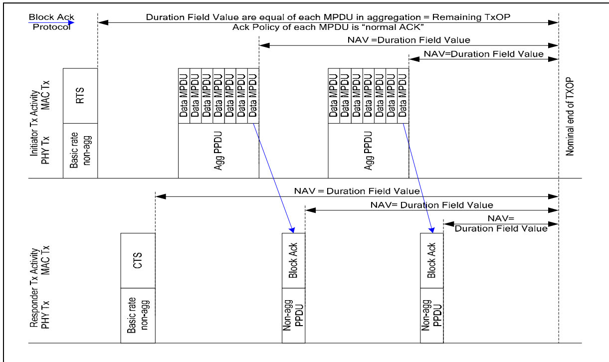
Figure n35 – Example of LongNAV Operation
