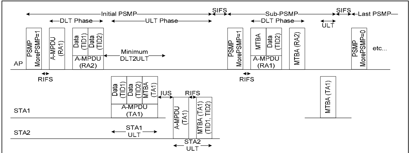
Figure n38 – PSMP sequence
