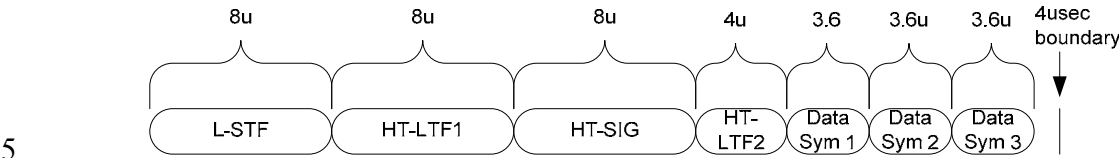
Figure n65 - Packet alignment example - GF packet with short GI
