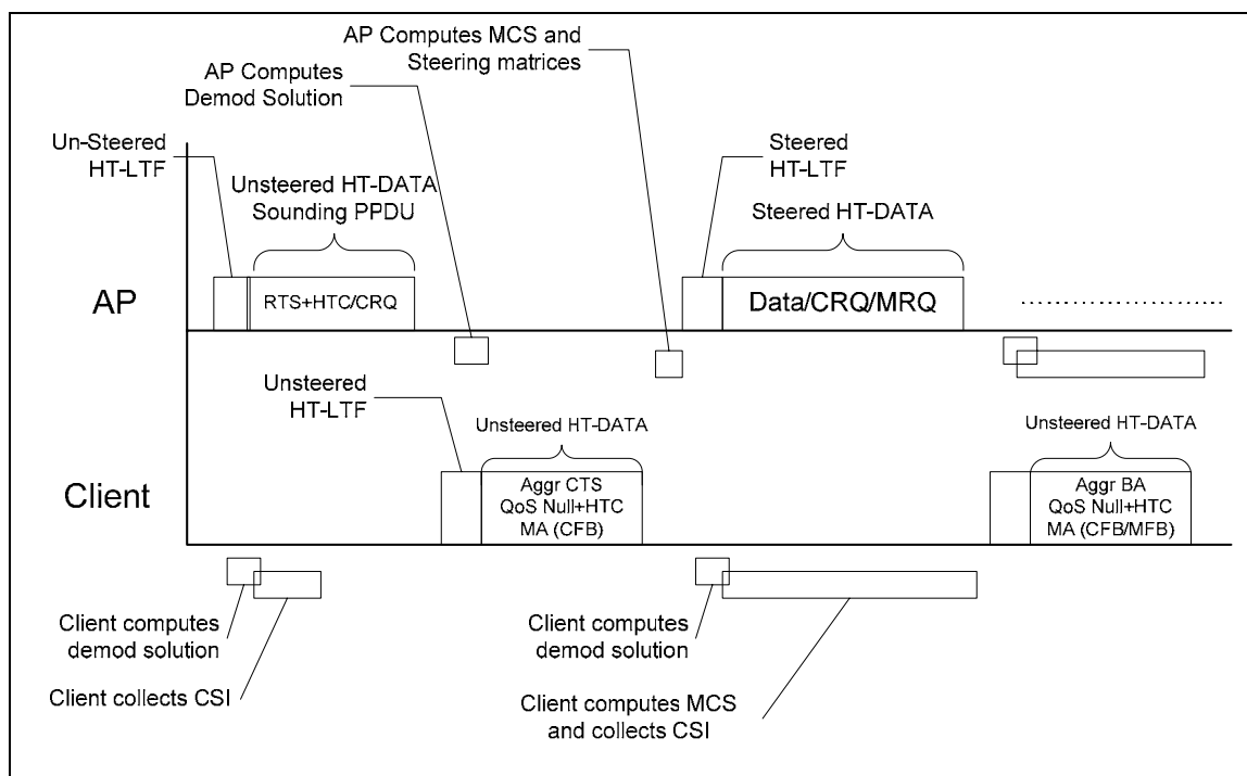
Figure n45 – Frame exchange for transmit beamforming with explicit feedback
