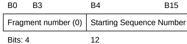
Figure n4 – Block Ack Starting Sequence Control field
