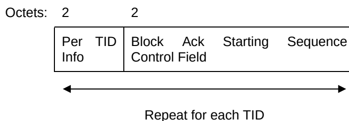
Figure n5 – MTBAR Block Ack Request Information field format
