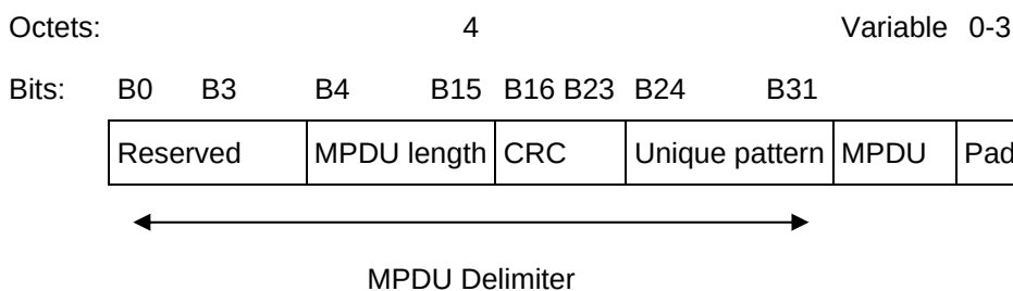
Figure n32 - A-MPDU sub-frame format
