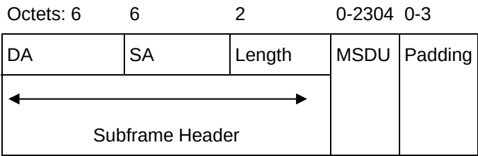
Figure n10 - A-MSDU subframe structure
