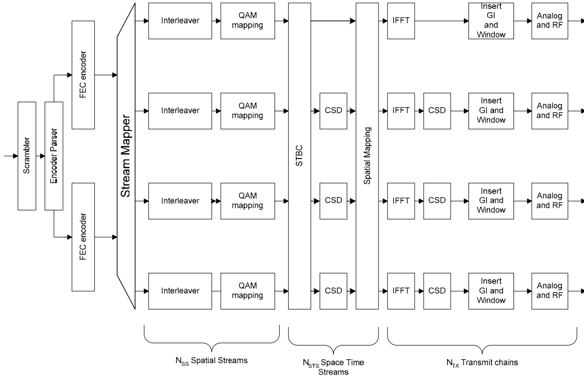
Figure n50 - Transmitter block diagram
