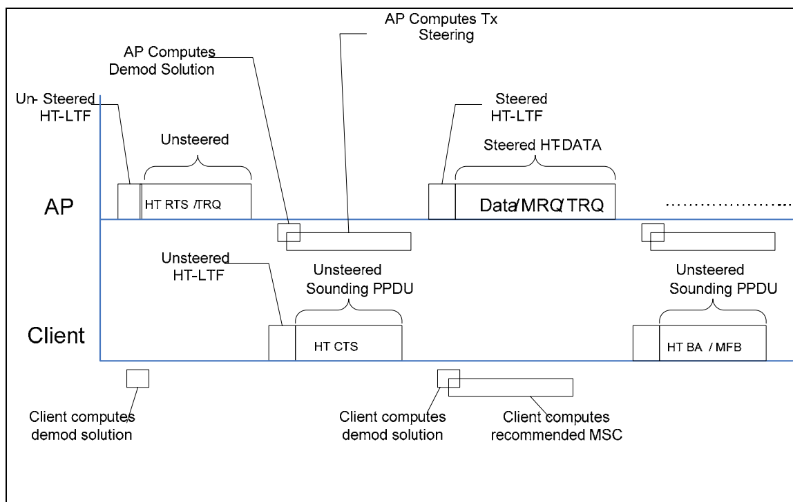
Figure n43 – Frame Exchange Sequence for Transmit Beamforming with Implicit Feedback
