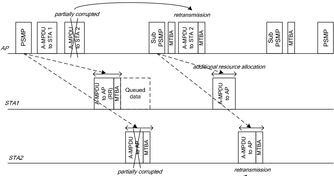
9 Figure n41 – Multi-phase PSMP showing additional resource allocation
