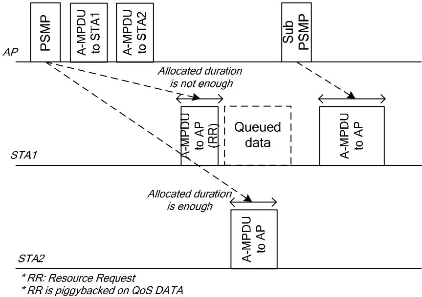
9 Figure n41 – Multi-phase PSMP showing additional resource allocation
