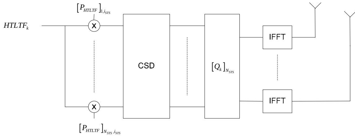
Figure n56 - Generation of data HT-LTFs
