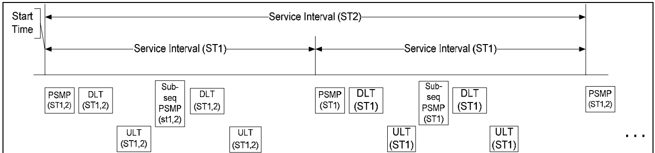
Figure n38 – PSMP sequence
