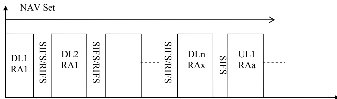
Figure n40 – Multiple RA packet transmission with RIFS or SIFS
