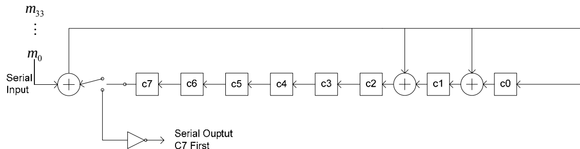
Figure n55 - HT-SIG CRC calculation
