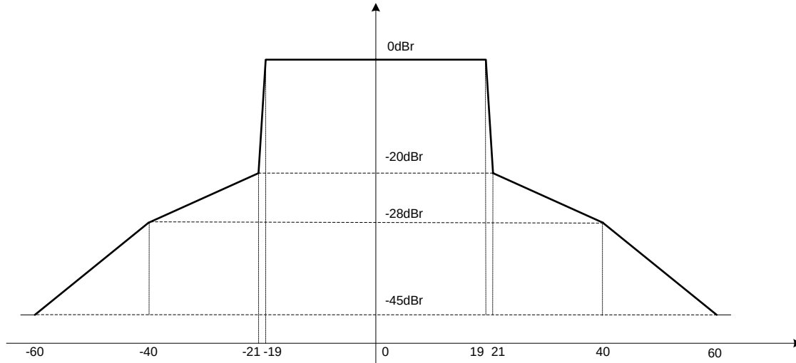
Figure n64 - Transmit spectral mask for a 40MHz channel
