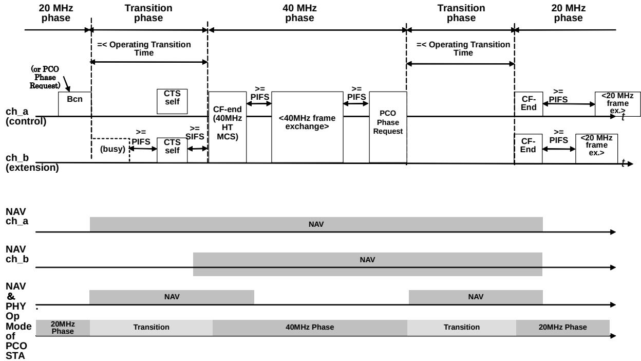
Figure n48 – Phased Coexistence Operations
