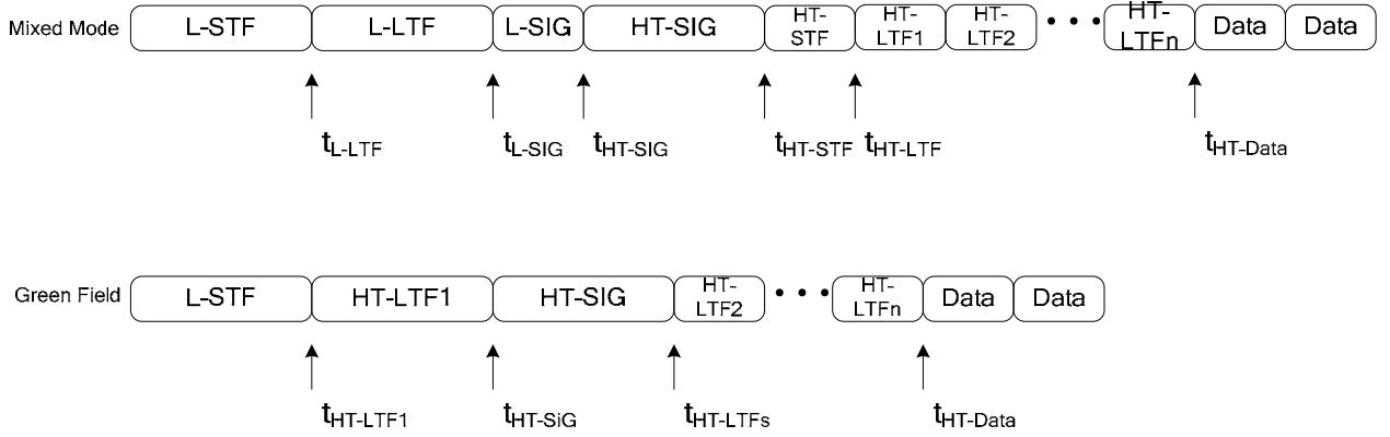
Figure n51: Timing boundaries for PPDU Fields
