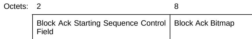
Figure n7 – Compressed Block Ack Information field format
