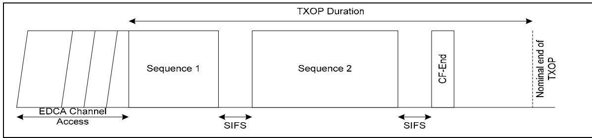
Figure n36 – Example of TXOP Truncation
