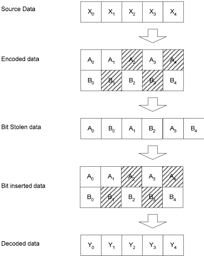
Figure n58 - Puncturing at rate 5/6
