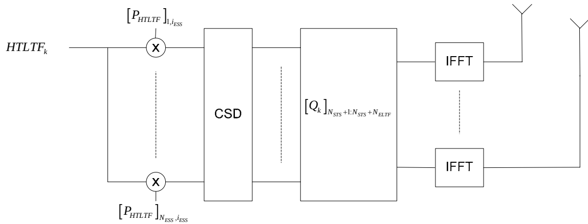
Figure n57 - Generation of the extension HT-LTFs
