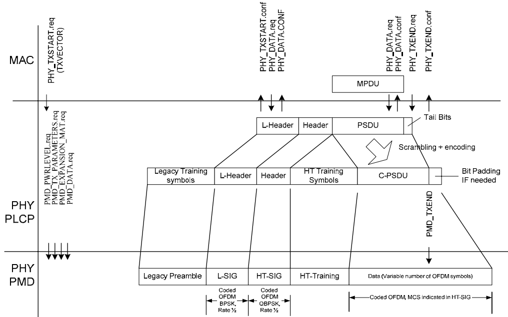
Figure n66 - PLCP Transmit Procedure – Mixed Mode Packet Format
