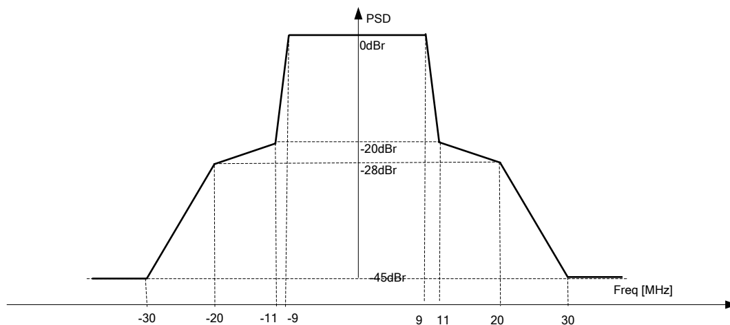
Figure n63 - Transmit spectral mask for 20MHz Transmission
