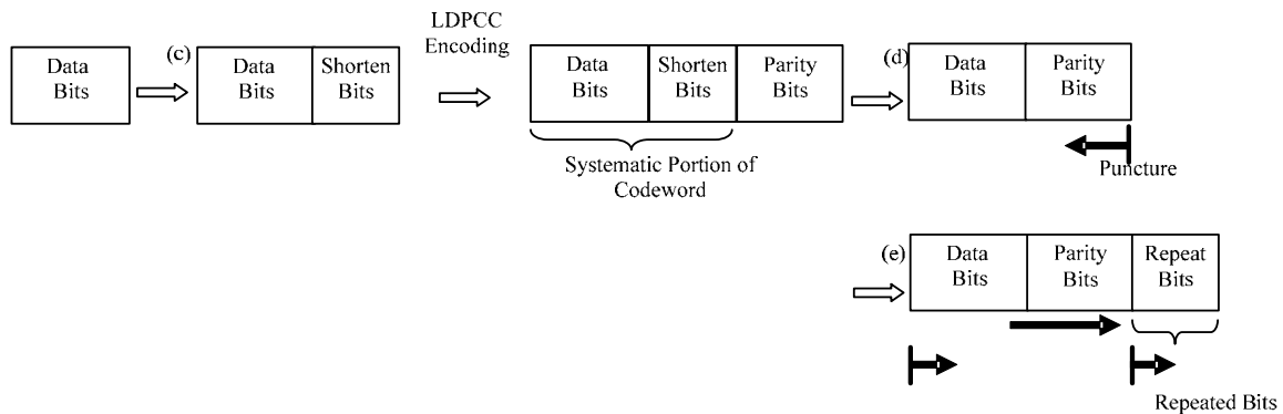
Figure n60 - LDPC PDU encoding padding and puncturing of a single codeword
