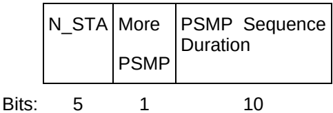
Figure n29 – PSMP Parameter Set format
