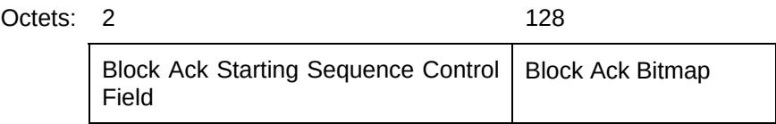
20 Figure n8 – Simple Block Ack Information field format
