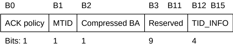
20 Figure 31 – BAR Control field
