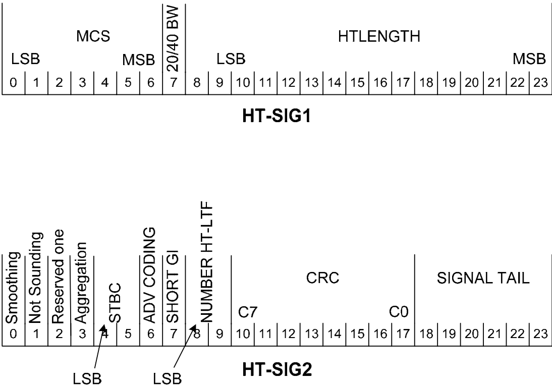
Figure n53 - HT SIG breakdown to HT-SIG1 and HT-SIG2
