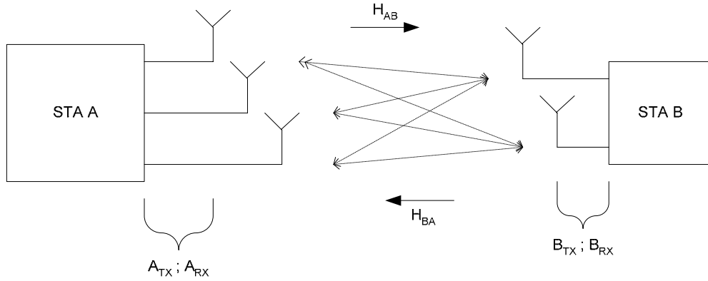
Figure n61 - The beamforming MIMO channel model
