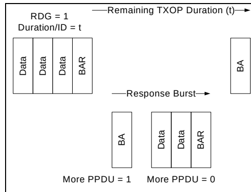
Figure n37 – Example of RD Operation showing response burst
