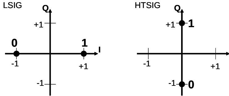
Figure n54 - constellation for the non-HT signal field and the HT signal field
