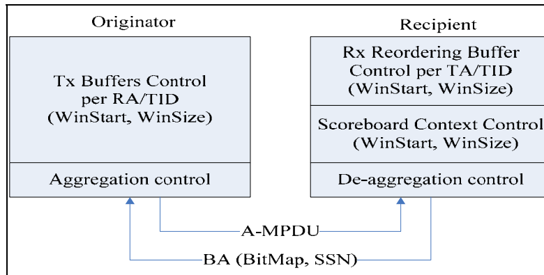
Figure n34 – Extended BlockAck Architecture
