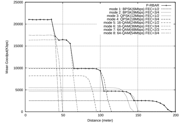
Fig. 6. Mean goodput of single CBR connection for P-RBAR
