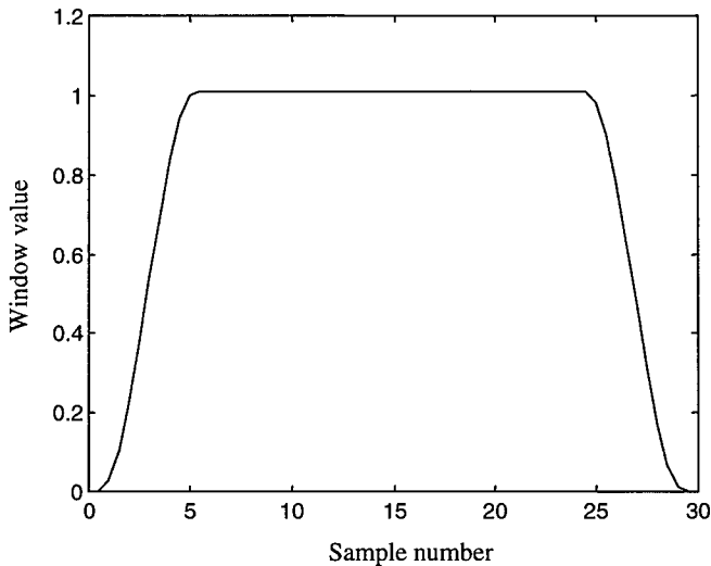
Figure 4.15 Raised cosine window.
