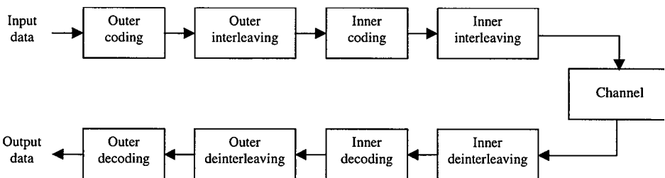
Figure 3.3 Concatenated coding/decoding.
