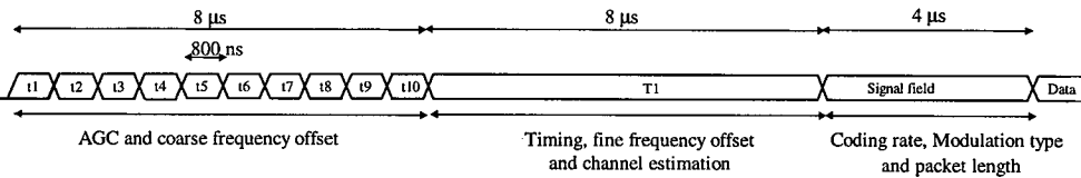
Figure 10.12 OFDM preamble.
