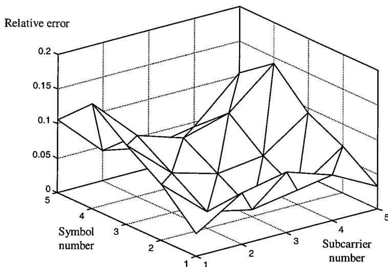
Figure 5.3 Example of relative channel estimation errors versus subcarrier number and symbol number.
