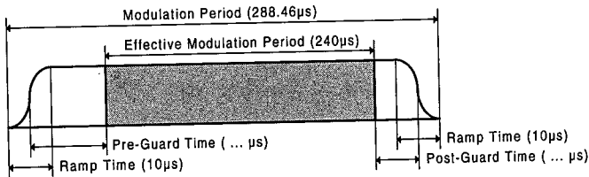
Figure 9.6 OFDM modulation burst.
