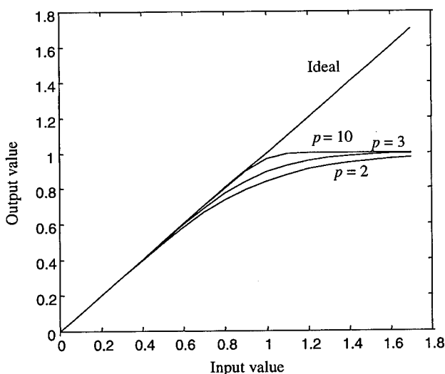
Figure 6.10 Rapp's model of AM/AM conversion.
