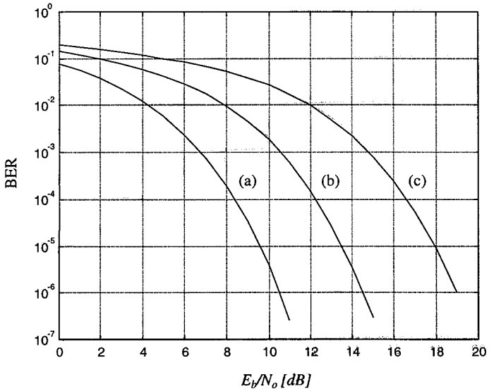
Figure 3.7 BER versus E_b/N_o for (a) BPSK/QPSK, (b) 16-QAM, (c) 64-QAM.
