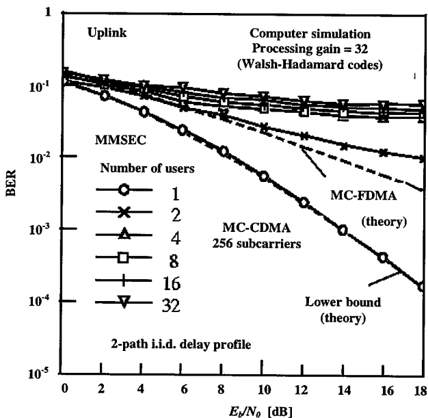
Figure 8.14 Uplink BER of MC-CDMA systems with MMSEC.
