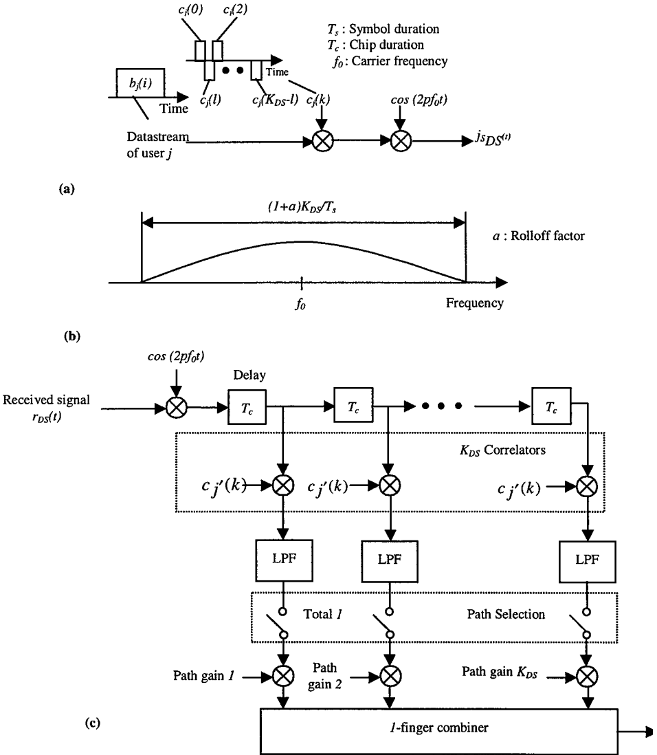
Figure 8.2 DS-CDMA system: (a) transmitter, (b) power spectrum of its transmitted signal, and (c) RAKE receiver.
