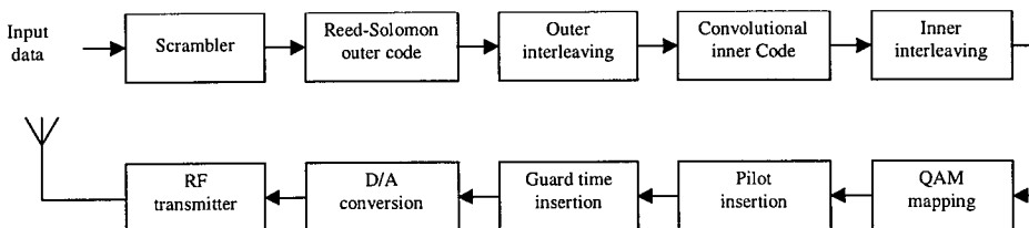
Figure 10.2 Block diagram of a DVB-T transmitter.
