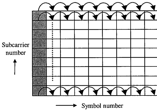
Figure 5.8 Differential detection in the time domain. Gray subcarriers are pilots that are needed for initial phase references.
