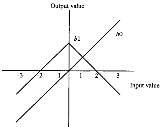
Figure 3.9 Demapping of 4 level PAM into 2 metrics.
