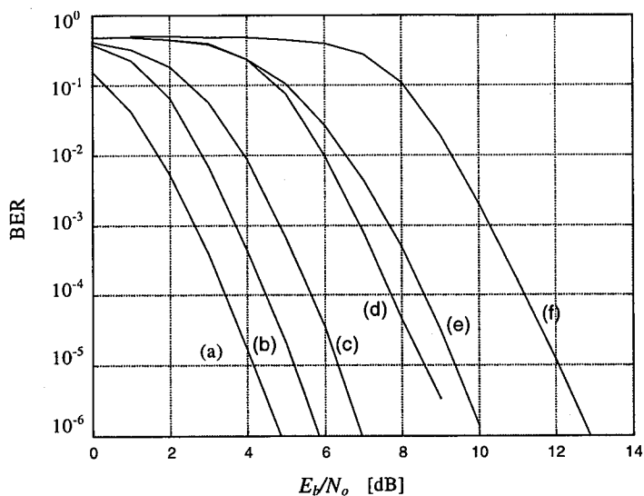
Figure 3.11 BERs versus E_b/N_0 in AWGN for a constraint length 7 convolutional code with (a) QPSK, rate \frac{1}{2} ; (b) QPSK, rate \frac{3}{4} ; (c) 16-QAM, rate \frac{1}{2} ; (d) 16-QAM, rate \frac{3}{4} ; (e) 64-QAM, rate \frac{1}{2} ; (f) 64-QAM, rate \frac{3}{4} .
