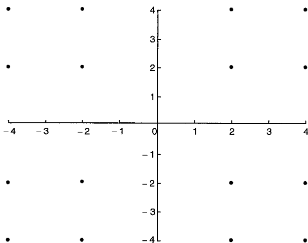
Figure 10.3 Hierarchical 16-QAM.
