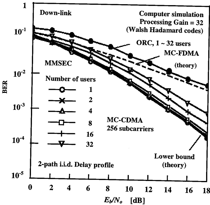
Figure 8.9 Downlink BER of MC-CDMA system with MMSEC.
