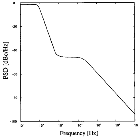
Figure 4.3 Example of a PLL phase noise spectrum.
