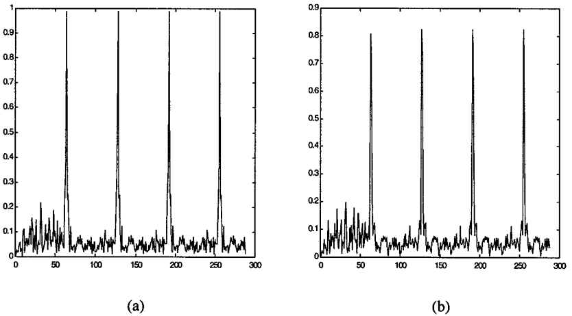
Figure 4.14 Matched filter output versus sample number with \{1, -1, 0\} values for in-phase and quadrature coefficients. (a) Zero fractional timing offset between input signals and matched filter coefficients, (b) worst case fractional offset of half a sample between input signal and reference pulse.
