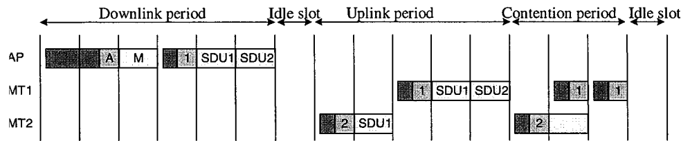
Figure 10.9 Magic WAND MAC frame.
