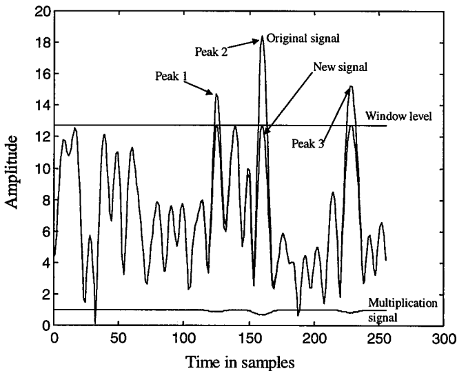
Figure 6.5 Windowing an OFDM time signal.
