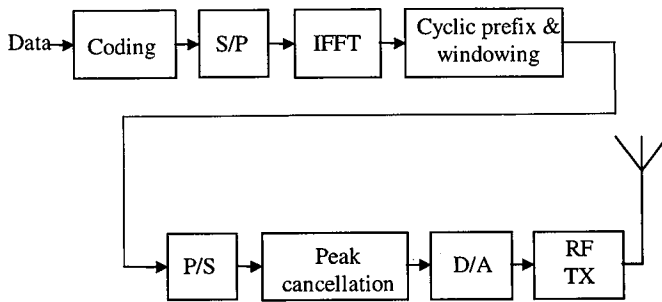
Figure 6.15 OFDM transmitter with peak cancellation.
