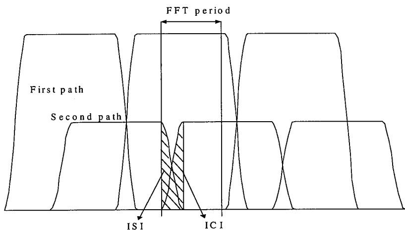
Figure 4.16 ISI/ICI caused by multipath signals.
