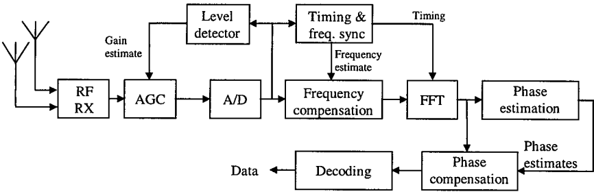
Figure 10.5 OFDM receiver.
