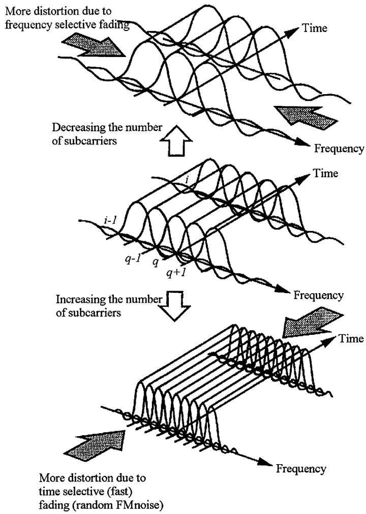
Figure 8.4 Optimum in the number of subcarriers.
