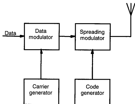
Figure 7.4 Block diagram of a DS-SS transmitter.
