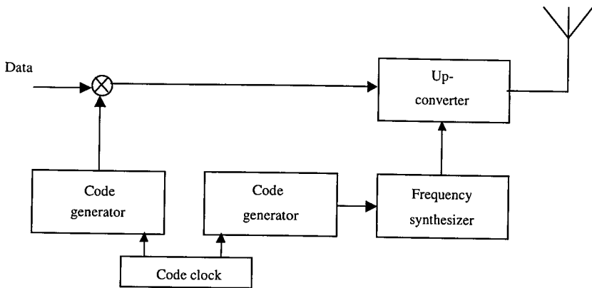
Figure 7.12 Hybrid DS-FH transmitter.
