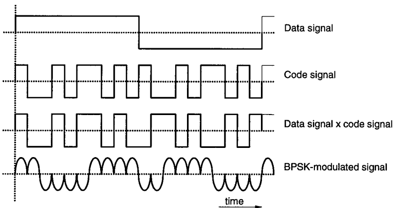
Figure 7.6 Generation of a BPSK-modulated spread-spectrum signal.
