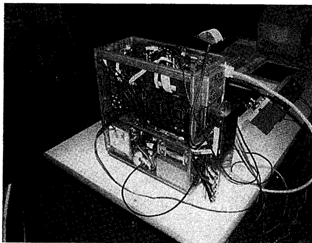
Figure 10.4 Magic WAND prototype 5-GHz modem.
