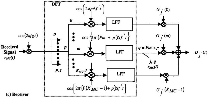
Figure 8.3 MC-CDMA system.
