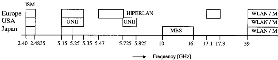
Figure 1.3 Frequency band for wireless broadband communications.
