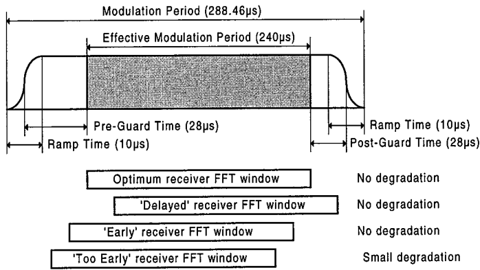
Figure 9.9 OFDMA burst and synchronization requirements.
