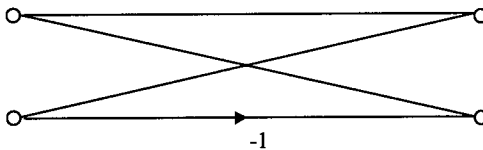
Figure 6.24 Butterfly of binary fast Walsh transform.
