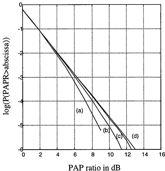
Figure 6.2 PAP distribution of an OFDM signal with (a) 12, (b) 24, (c) 48 and (d) an infinite number of subcarriers (pure Gaussian noise). Four times oversampling used in simulation, total number of simulated samples = 12 million.
