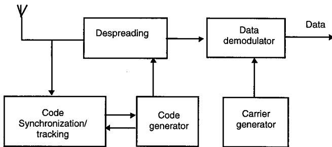
Figure 7.7 Receiver of a DS-SS signal.
