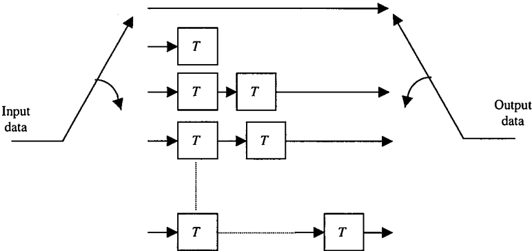
Figure 3.5 Convolutional interleaver.
