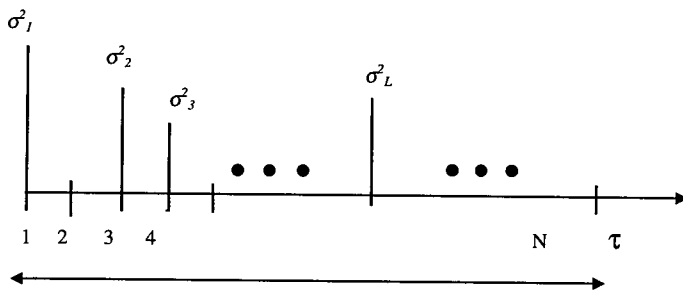
Figure 8.1 Multipath power delay profile.
