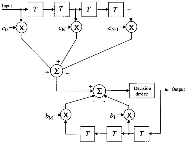
Figure 2.15 Decision-feedback equalizer.
