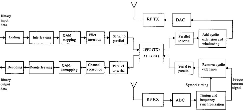
Figure 10.11 Block diagram of OFDM transceiver.
