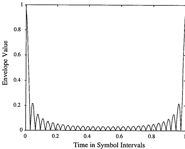
Figure 6.17 Envelope of cyclic reference function.
