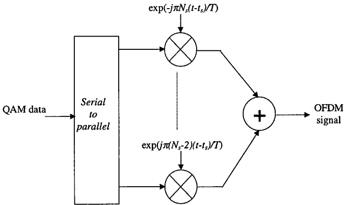
Figure 2.1 OFDM modulator.
