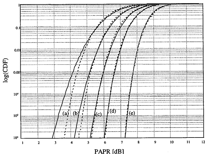
Figure 6.4 Cumulative distribution function of the PAPR for a number of subcarriers of (a) 32, (b) 64, (c) 128, (d) 256, and (e) 1,024. Solid lines are calculated; dotted lines are simulated.
