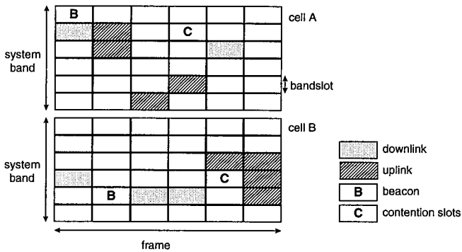
Figure 9.11 Example of frame layout.
