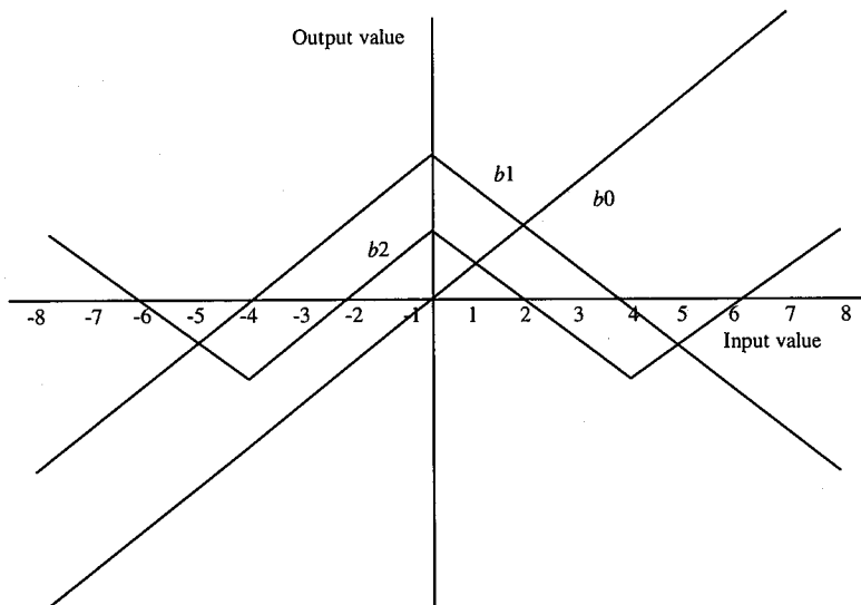
Figure 3.10 Demapping of 8 level PAM into 3 metrics.
