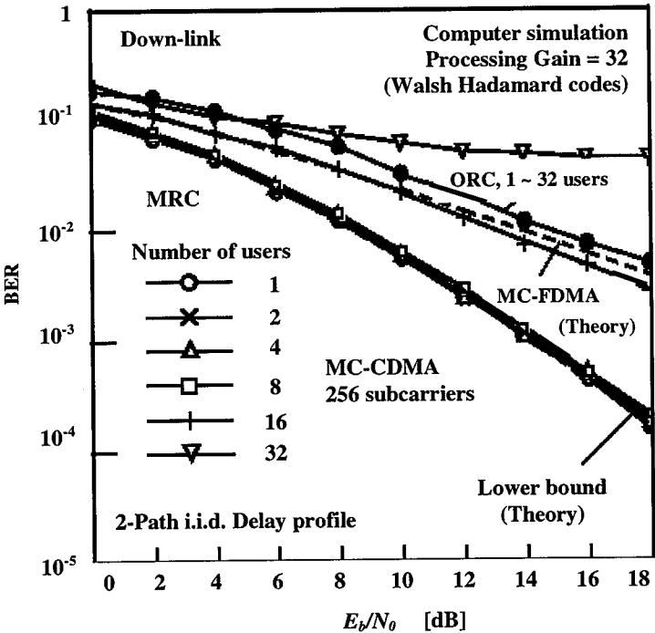
Figure 8.8 Downlink BER of MC-CDMA system with MRC.
