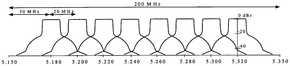
Figure 10.10 Channelization in lower and middle UNII band.
