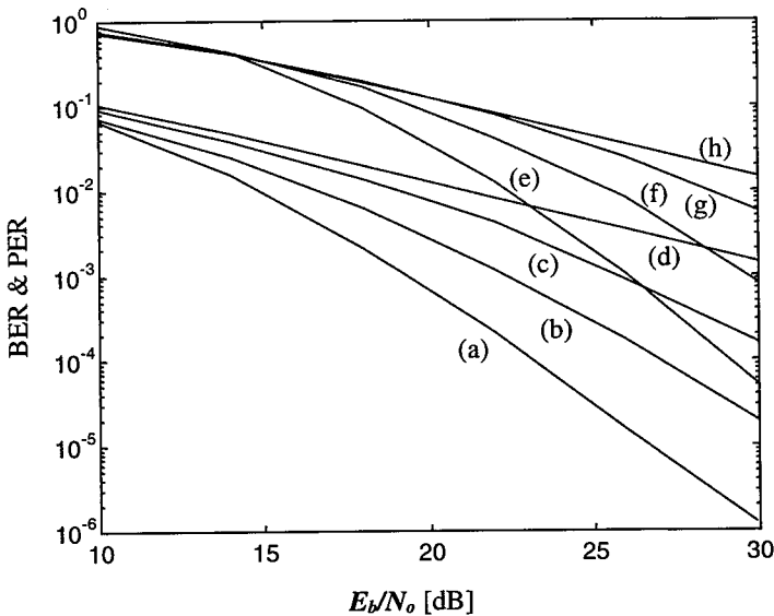
Figure 6.28 BER (a-d) and PER (e-h) versus mean E_b/N_o for delay spreads of (a) and (e) 50 ns, (b) and (f) 20 ns, (c) and (g) 10 ns, (d) and (h) 0.
