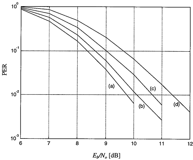
Figure 6.8 Packet error ratio versus E_b/N_o for 64 byte packets in AWGN. OFDM signal is clipped to a PAP ratio of (a) 16 (= no distortion), (b) 6, (c) 5, and (d) 4 dB.
