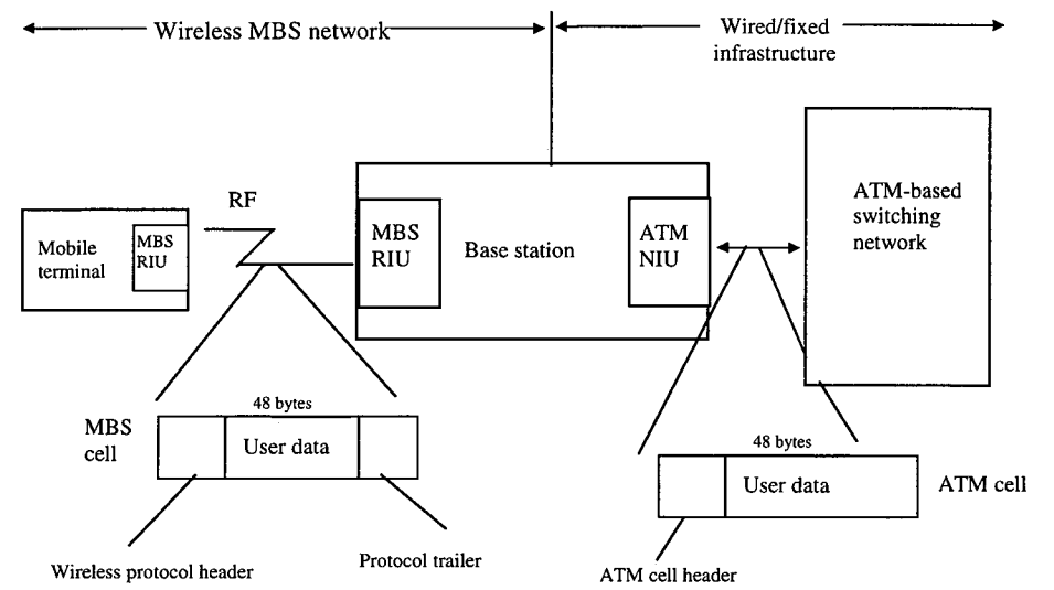
Figure 1.6 ATM-compatible MBS approach. Terms: radio interface unit (RIU); network interface unit (NIU).
