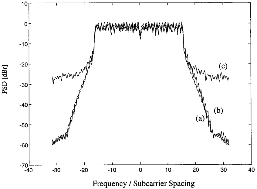
Figure 6.20 Power spectral density for (a) undistorted spectrum with 32 subcarriers, PAP = 15dB, (b) spectrum after peak cancellation to PAP = 4 dB, and (c) clipping to PAP = 4 dB. Referential cancellation function has a length equal to \frac{1}{4} of the length of an OFDM symbol.
