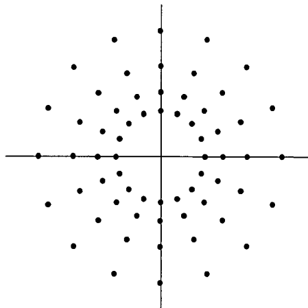
Figure 5.14 64-DAPSK constellation.
