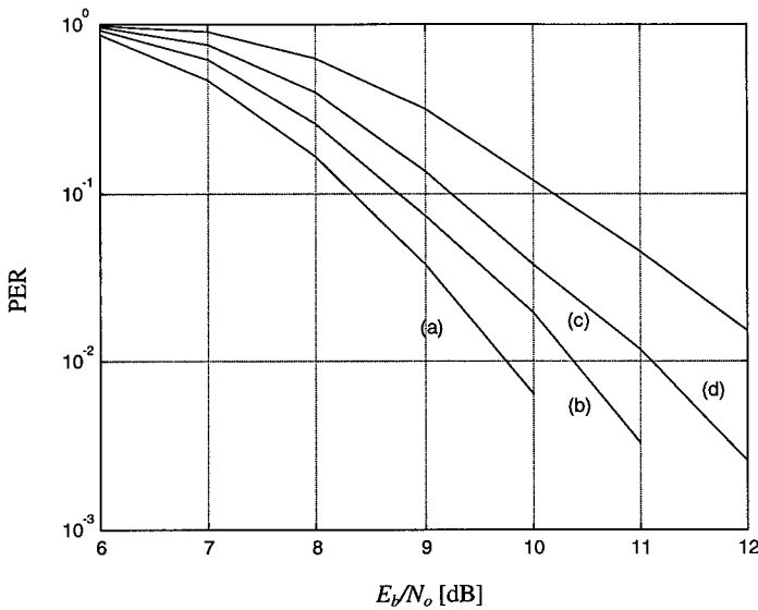
Figure 6.21 PER versus E_b/N_o for 64-byte packets in AWGN. Peak cancellation is applied to reduce the PAP ratio to (a) 16 (= no distortion), (b) 6, (c) 5, and (d) 4 dB.
