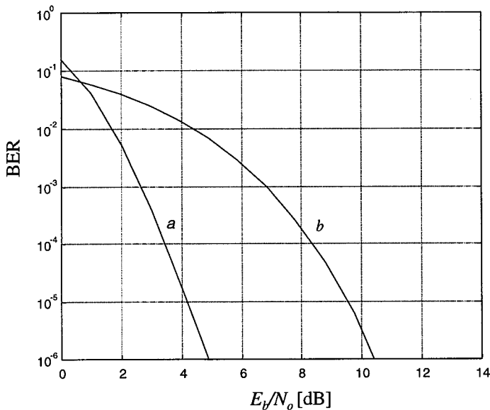
Figure 3.2 BER versus E_b/N_o for coded and uncoded QPSK in AWGN.
