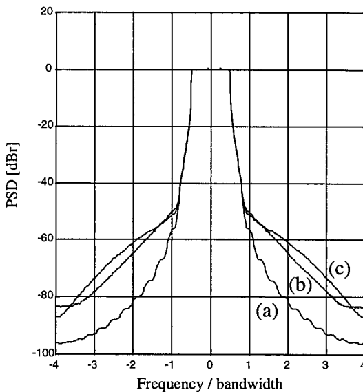
Figure 6.11 (a) Ideal OFDM spectrum for 64 subcarriers, (b) spectrum after highly linear amplifier (Rapp's parameter p = 10 ) with 8.7-dB backoff, (c) spectrum using peak windowing with 5.9-dB backoff.
