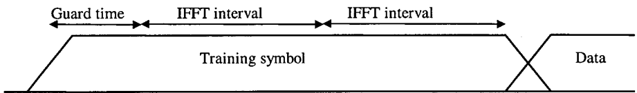
Figure 5.6 Extended training symbol for channel estimation with a single guard time and multiple IFFT intervals.
