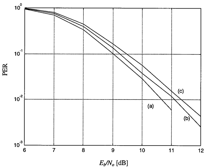
Figure 6.22 Packet error ratio versus E_b/N_o for 64-byte packets in AWGN. PAP ratio is reduced to 5 dB by (a) clipping, (b) peak cancellation, and (c) peak windowing.
