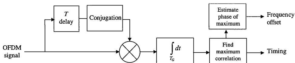
Figure 4.7 Synchronization using the cyclic prefix.
