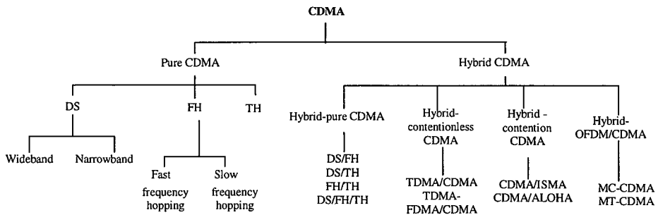
Figure 7.3 Classification of CDMA.
