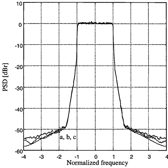
Figure 6.30 OFDM spectra for (a) no scrambling with a 8.5-dB backoff, (b) 1 scrambling code with 7.2 dB backoff and (c) 10 scrambling codes with a 6.5-dB backoff.
