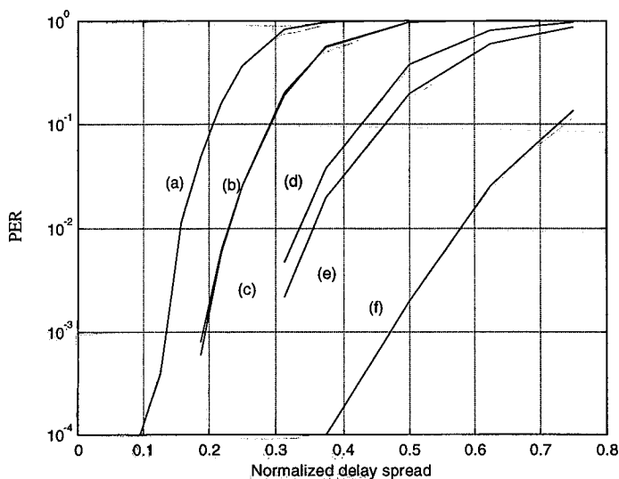
Figure 3.15 Irreducible packet error ratios versus normalized delay spread \tau_{ms}/T_G for 256 byte packets and (a) 64-QAM, rate \frac{3}{4} ; (b) 64-QAM, rate \frac{1}{2} ; (c) 16-QAM, rate \frac{3}{4} ; (d) 16-QAM, rate \frac{1}{2} ; (e) QPSK, rate \frac{3}{4} ; (f) QPSK, rate \frac{1}{2} .
