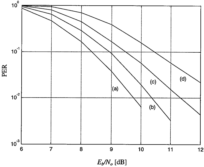
Figure 6.9 PER versus E_b/N_o for 64-byte packets in AWGN. Peak windowing is applied with a window width of 1/16 of the FFT duration. The PAP ratio is reduced to (a) 16 (= no distortion), (b) 6, (c) 5, and (d) 4 dB.
