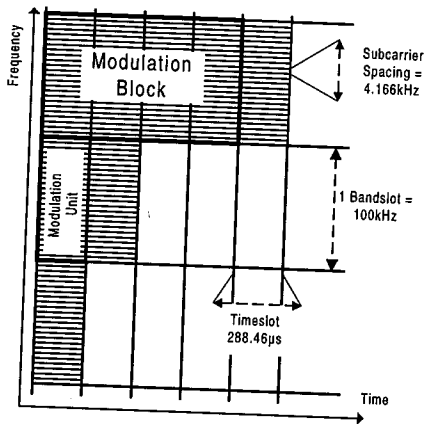
Figure 9.4 Time-frequency grid.
