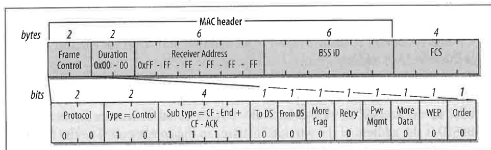
Figure 8-8. CF-End+CF-Ack frame
