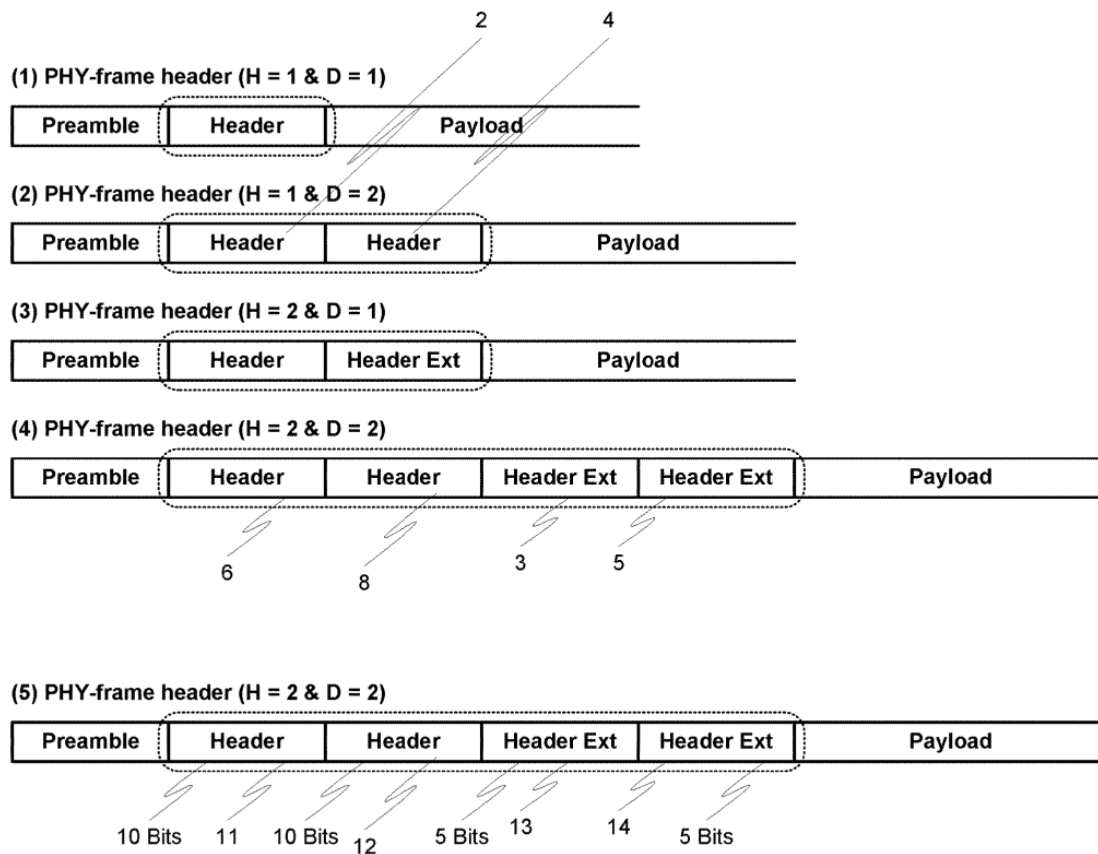
'272 Patent, Figure 1
