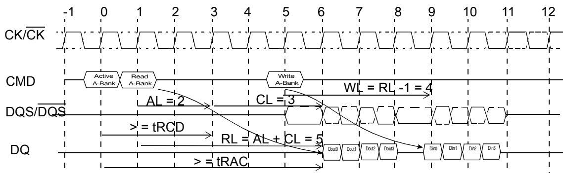
Figure 21 — Example 1: Read Followed by a Write to the Same Bank [AL = 2 and CL = 3, RL = (AL + CL) = 5, WL = (RL - 1) = 4, BL = 4]
