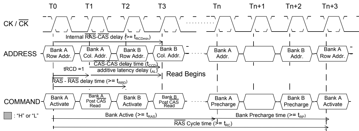
Figure 20 — Bank Activate Command Cycle: t_{\text{RCD}} = 3 , AL = 2 , t_{\text{RP}} = 3 , t_{\text{RRD}} = 2 , t_{\text{CCD}} = 2
