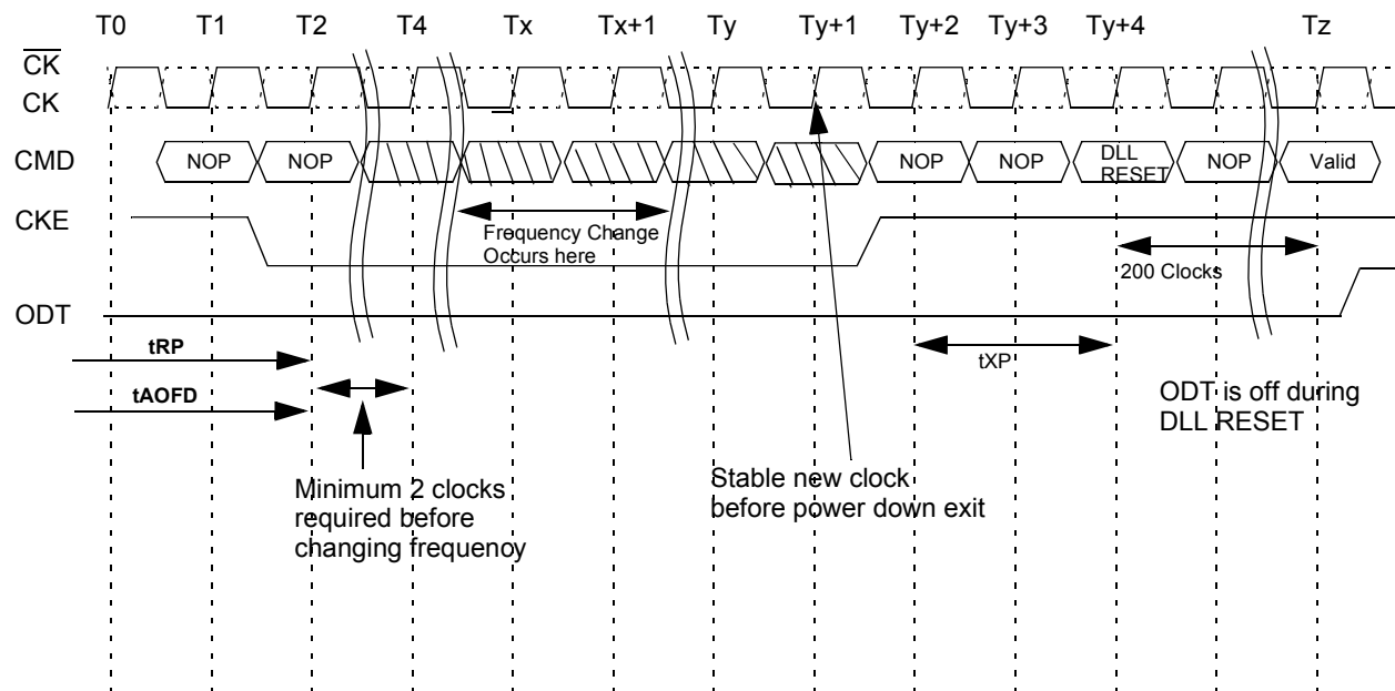
Figure 61 — Clock Frequency Change in Precharge Power
