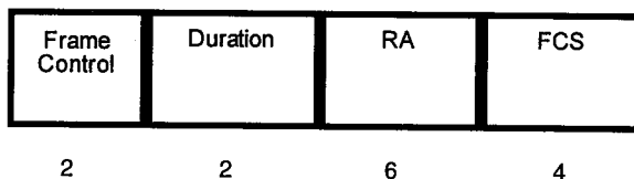
Figure 3-8—Clear to Send Frame
