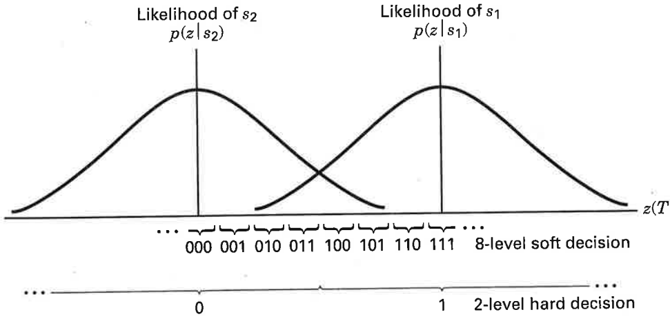
Figure 7.8 Hard and soft decoding decisions.
