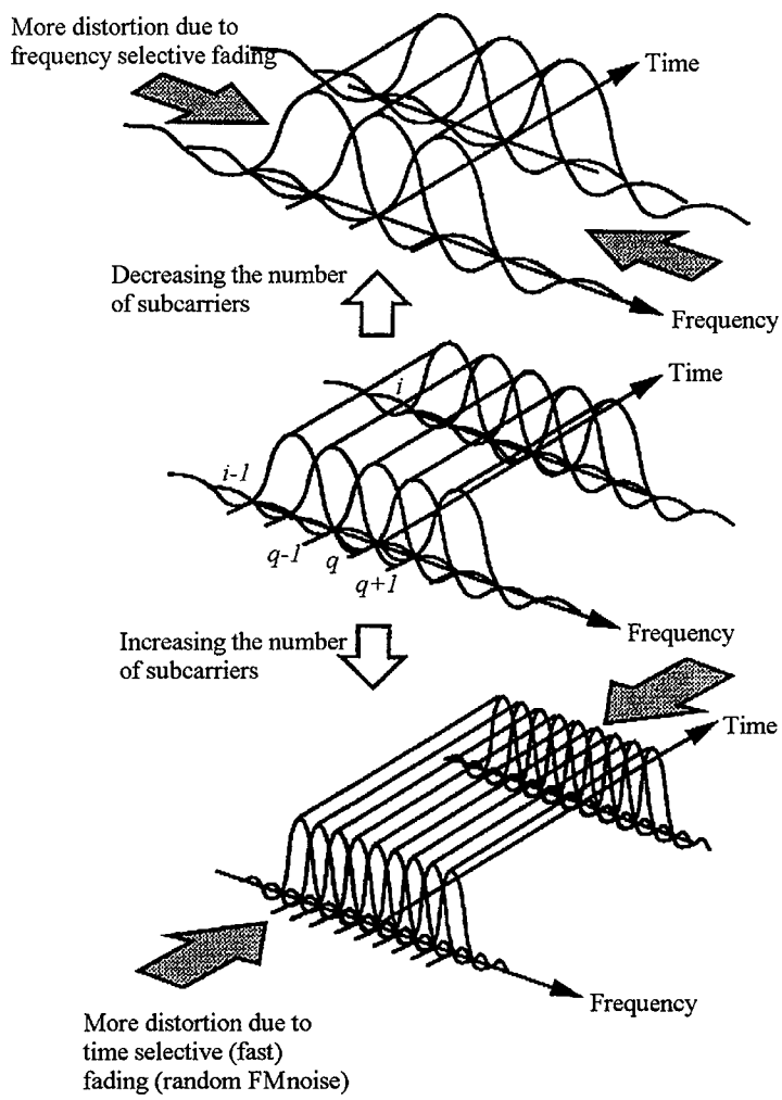
Figure 8.4 Optimum in the number of subcarriers.
