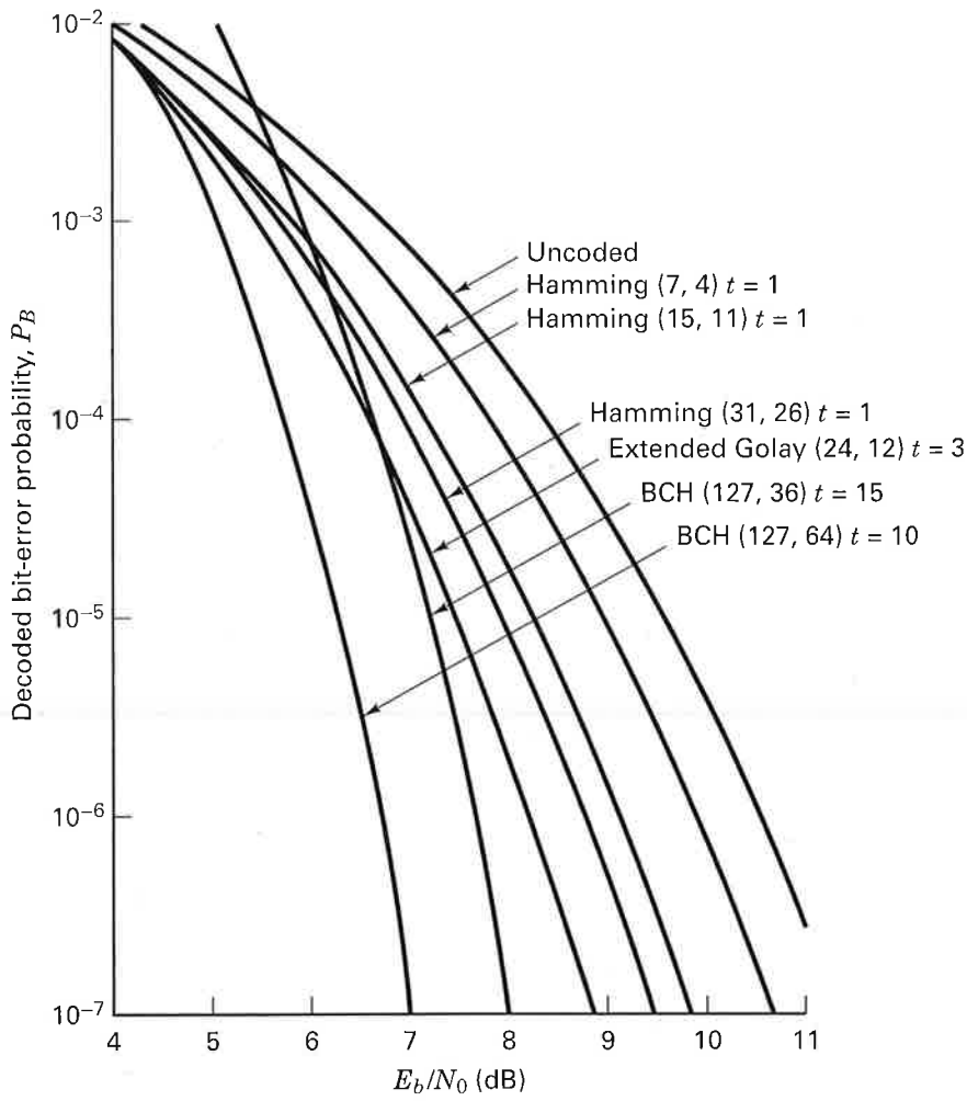
Figure 6.22 P_B versus E_b/N_0 for coherently demodulated BPSK over a Gaussian channel for several block codes.
