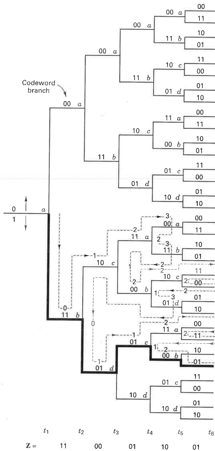
Figure 7.23 Sequential decoding example.
