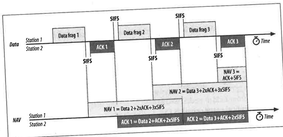
Figure 3-16. Fragmentation
