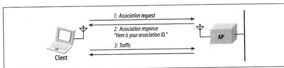
Figure 7-7. Association procedure
