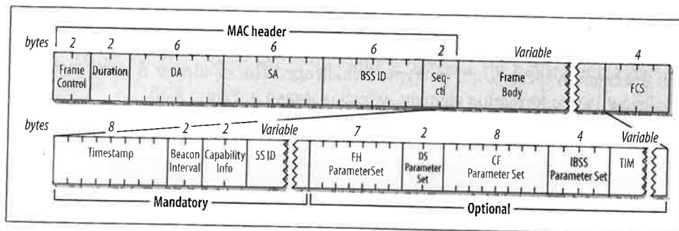
Figure 4-39. Beacon frame
