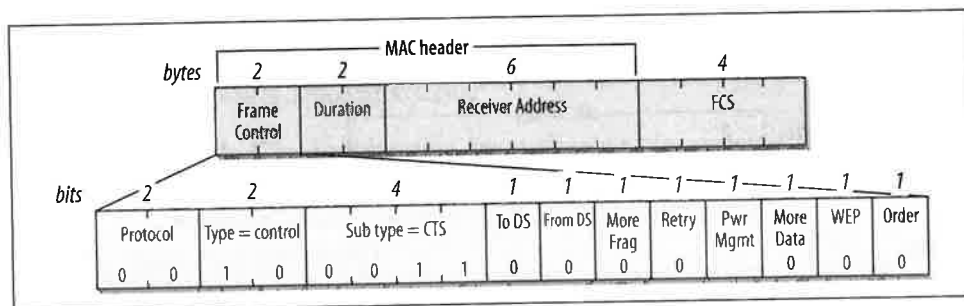
Figure 4-15. CTS frame
