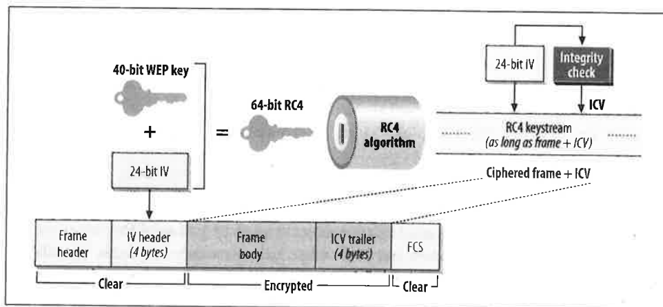
Figure 5-3. WEP operations
