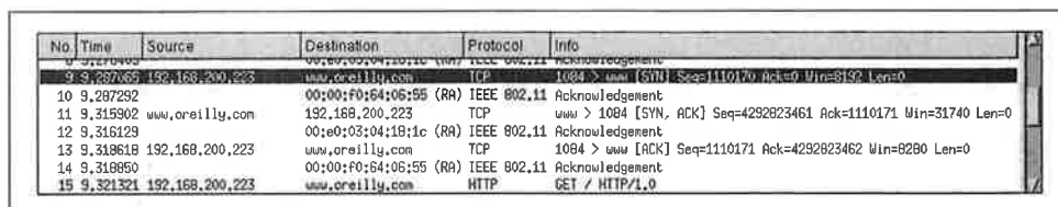
Figure 16-25. TCP three-way handshake
