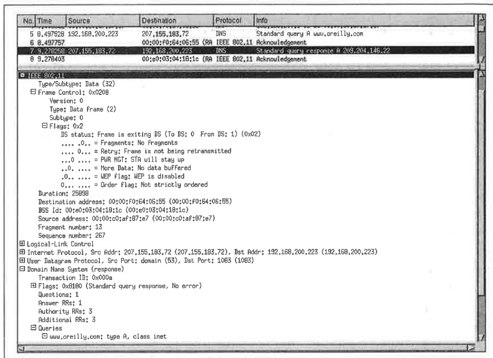
Figure 16-24. DNS reply
