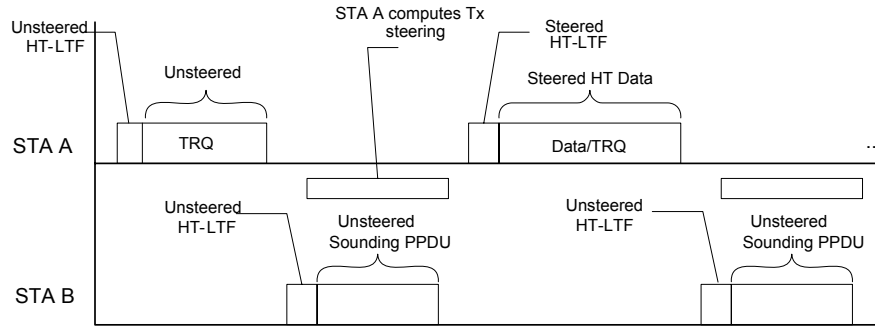
Figure 9-31—Example PPDU exchange for unidirectional implicit transmit beamforming
