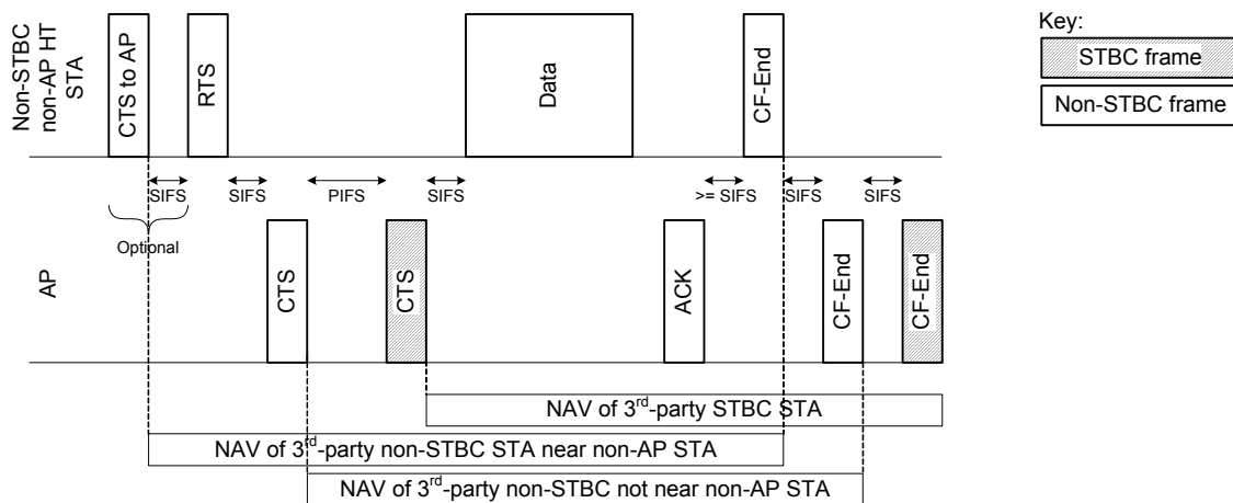
Figure 9-8b—Example of the dual CTS mechanism (non-STBC initiator)
