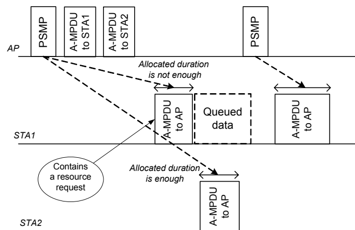
Figure 9-29—PSMP burst showing resource allocation
