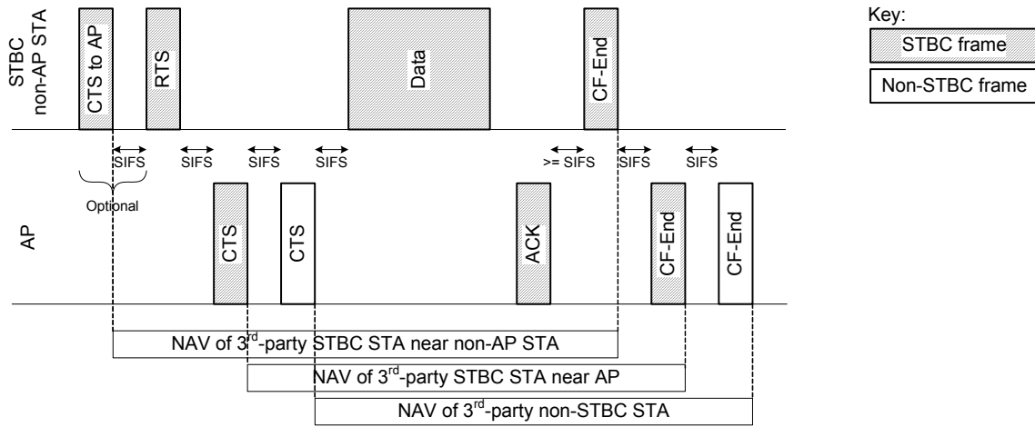
Figure 9-8a—Example of dual CTS mechanism (STBC initiator)
