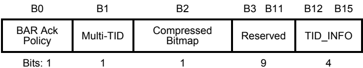
Figure 7-13—BAR Control field
