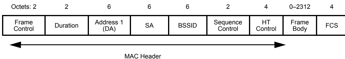
Figure 7-18—Management frame format
