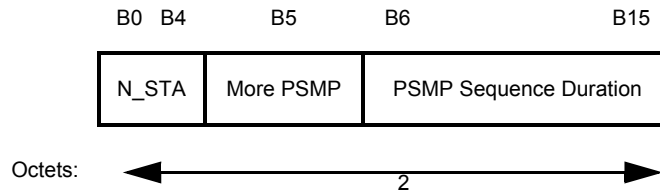
Figure 7-36g—PSMP Parameter Set fixed field
