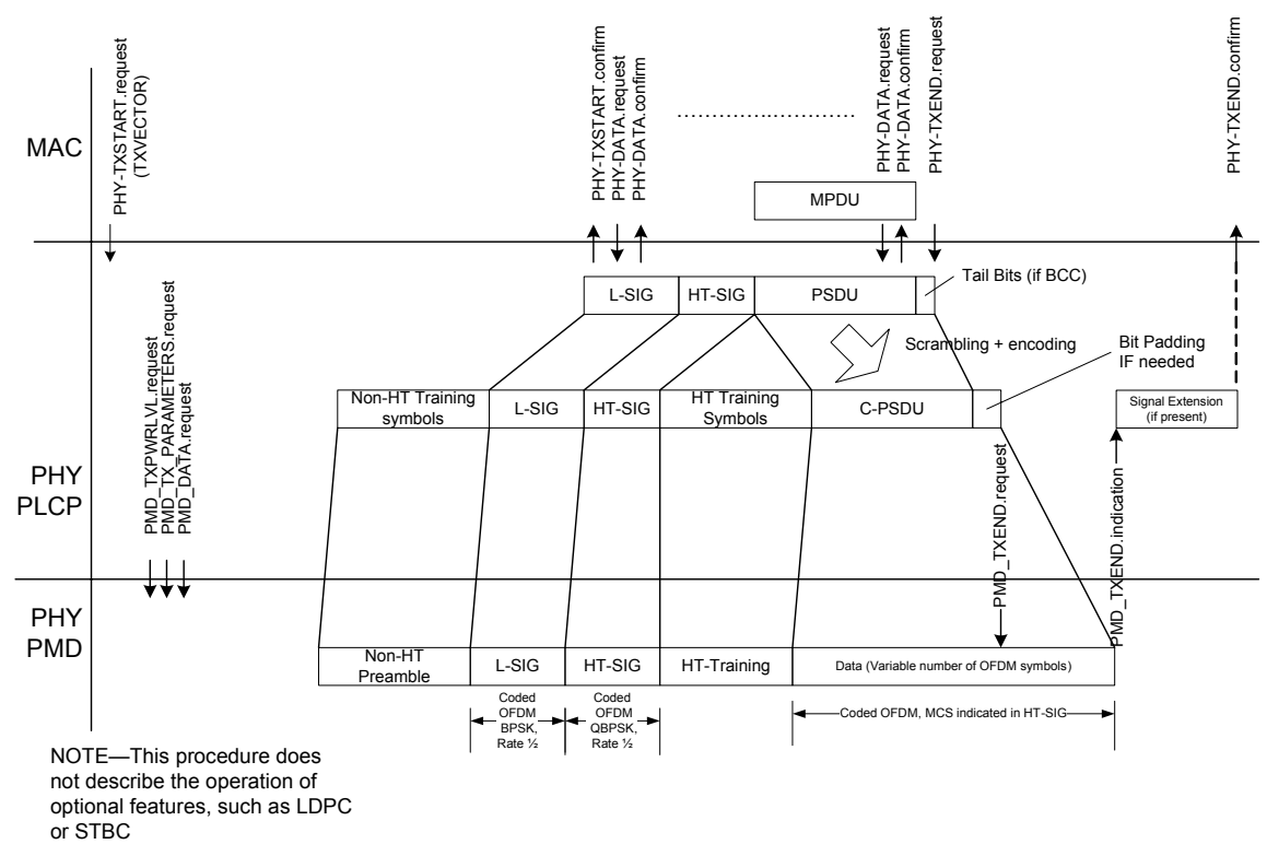
Figure 20-20—PLCP transmit procedure (HT-mixed format PPDU)
