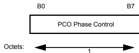
Figure 7-36f—PCO Phase Control fixed field
