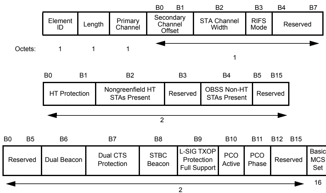
Figure 7-95o24—HT Operation element format
