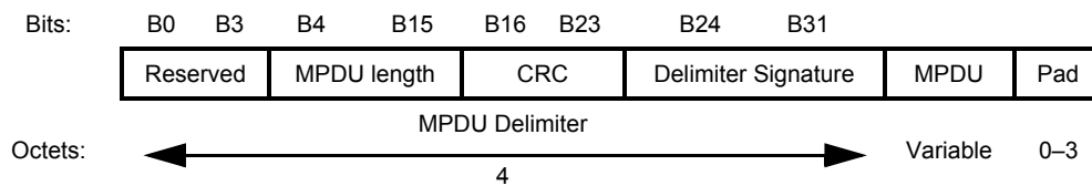
Figure 7-101p—A-MPDU subframe format
