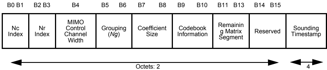
Figure 7-36j—MIMO Control field
