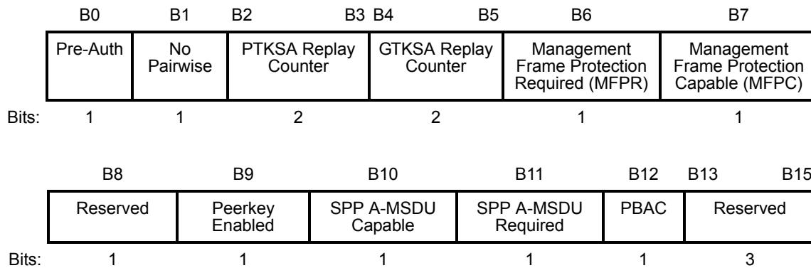
Figure 7-74—RSN Capabilities field format
