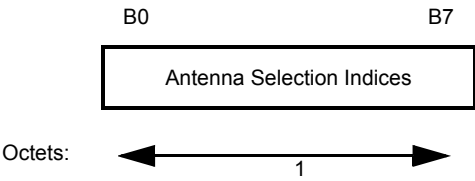
Figure 7-36o—Antenna Selection Indices fixed field
