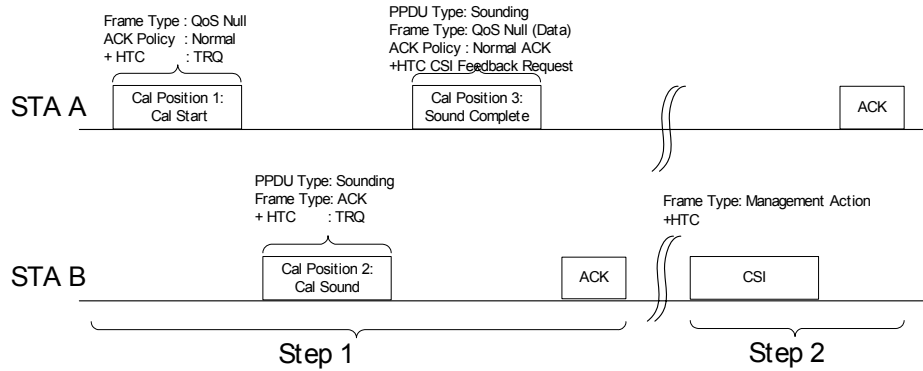
Figure 9-33—Calibration procedure with sounding PPDU containing an MPDU
