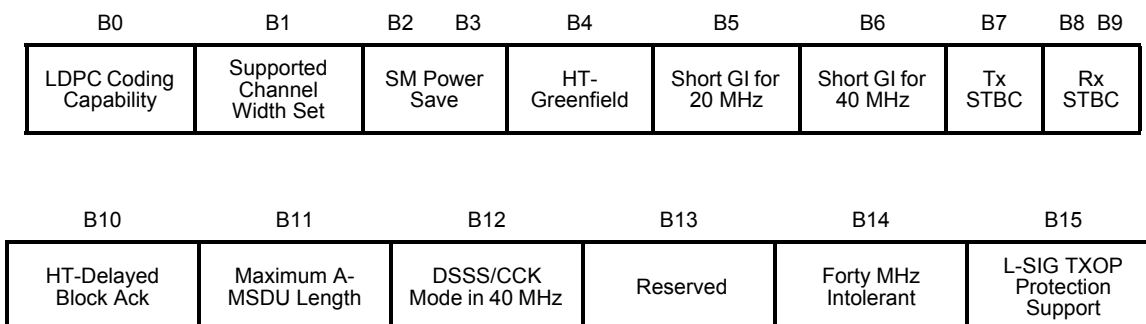
Figure 7-95o18—HT Capabilities Info field
