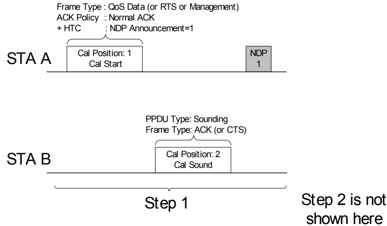
Figure 9-35—Calibration procedure with NDP when STA B supports transmitting sounding PPDU for which only one channel dimension can be estimated (i.e., a single column of the MIMO channel matrix)
