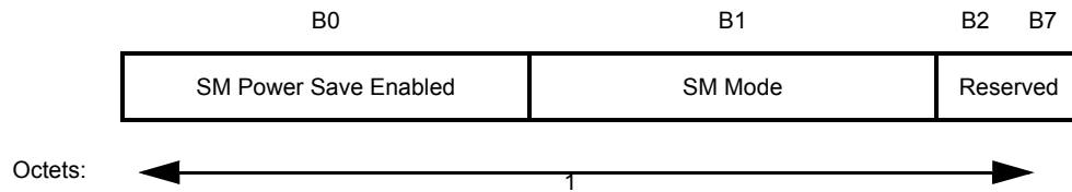
Figure 7-36e—SM Power Control fixed field
