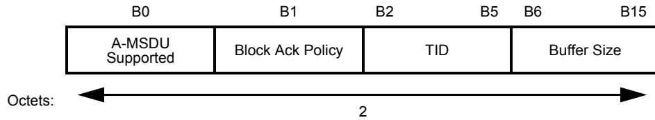
Figure 7-32—Block Ack Parameter Set fixed field
