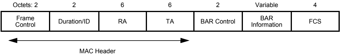
Figure 7-12—BlockAckReq frame
