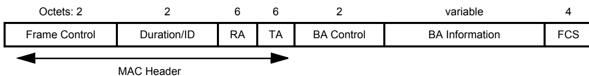
Figure 7-15—BlockAck frame
