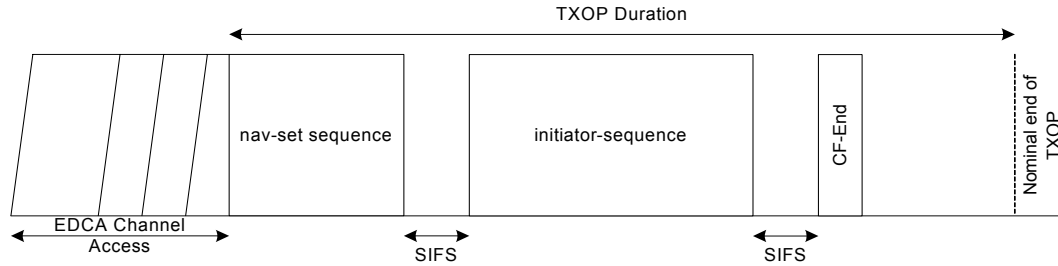
Figure 9-18a—Example of TXOP truncation
