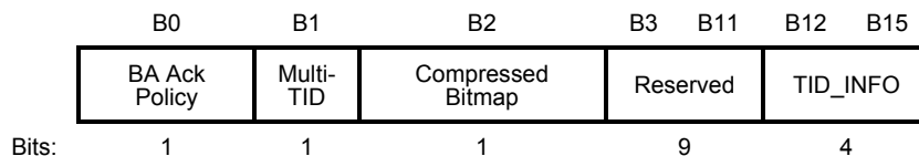
Figure 7-16—BA Control field
