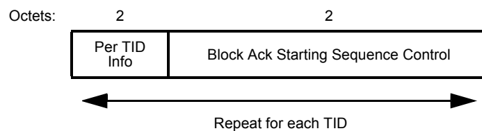
Figure 7-14a—BAR Information field (Multi-TID BlockAckReq)
