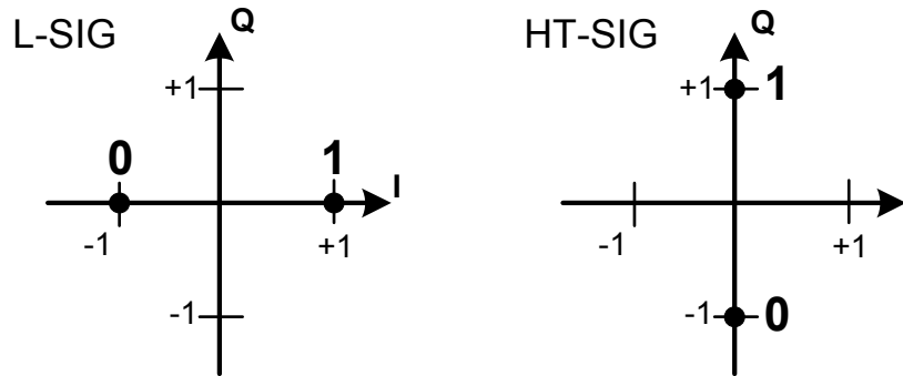
Figure 20-7—Data tone constellations in an HT-mixed format PPDUs
