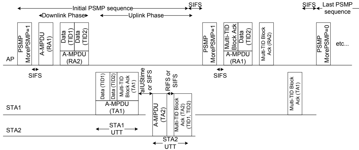
Figure 9-28—PSMP burst
