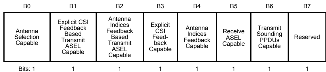
Figure 7-95o23—ASEL Capability field
