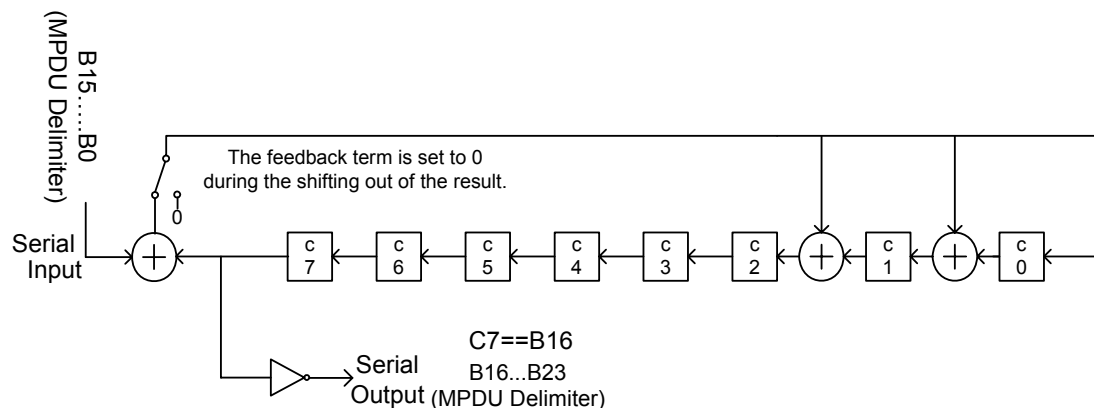
Figure 7-101q—MPDU delimiter CRC calculation
