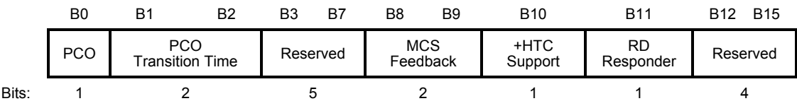
Figure 7-95o21—HT Extended Capabilities field
