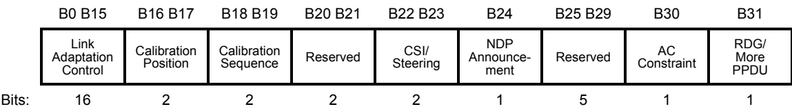
Figure 7-4a—HT Control field
