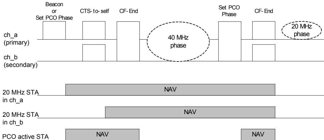
Figure 11-20—Phased coexistence operation (PCO)
