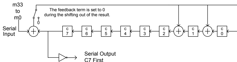
Figure 20-8—HT-SIG CRC calculation
