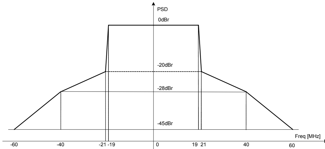
Figure 20-18—Transmit spectral mask for a 40 MHz channel
