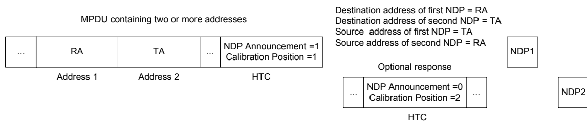
Figure T.4—Determination of NDP source and destination for bidirectional NDP sequence
