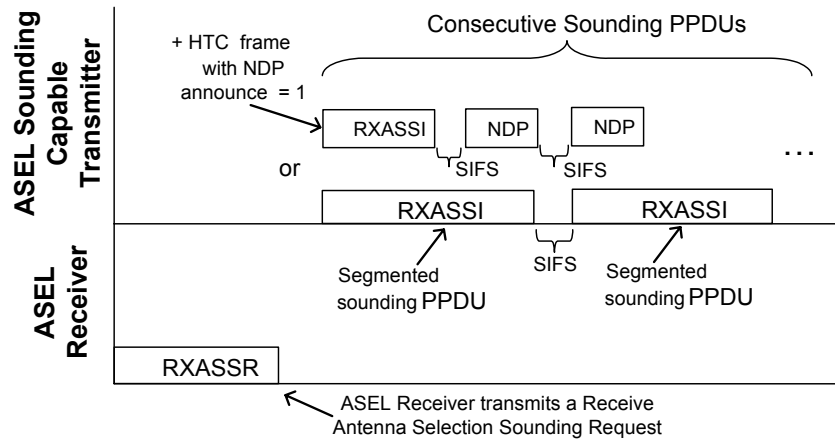
Figure 9-37—Receive ASEL
