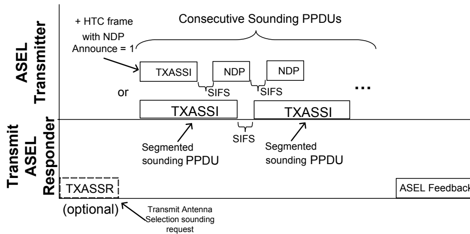
Figure 9-36—Transmit ASEL
