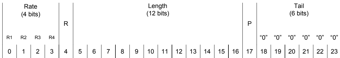
Figure 20-5—L-SIG structure
