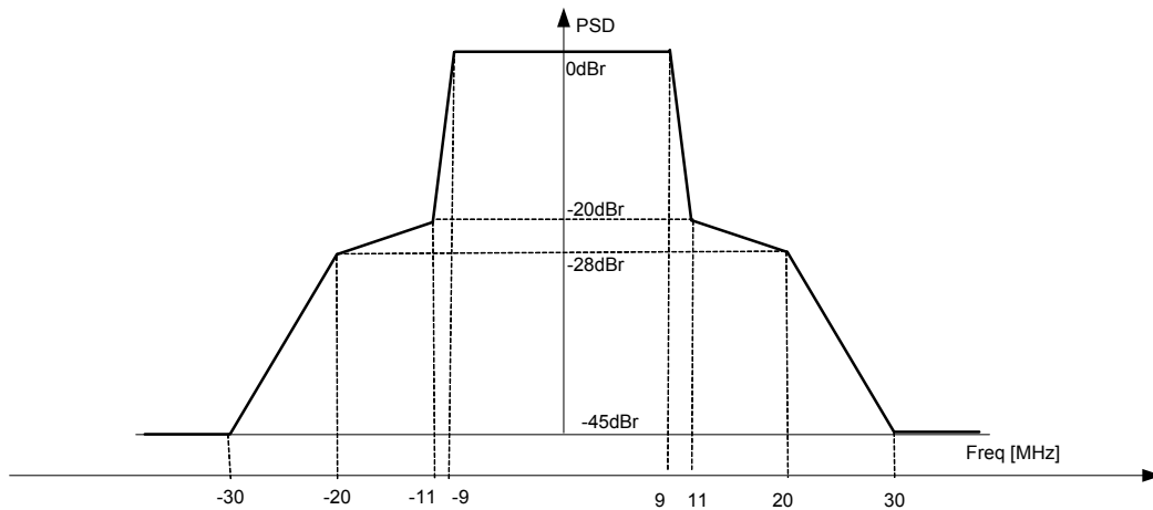
Figure 20-17—Transmit spectral mask for 20 MHz transmission
