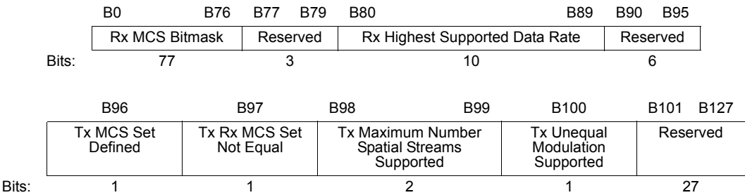
Figure 7-95o20—Supported MCS Set field
