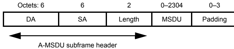
Figure 7-17b—A-MSDU subframe structure
