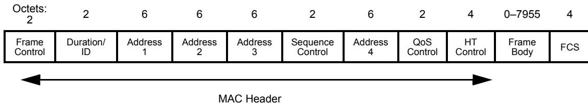
Figure 7-17—Data frame
