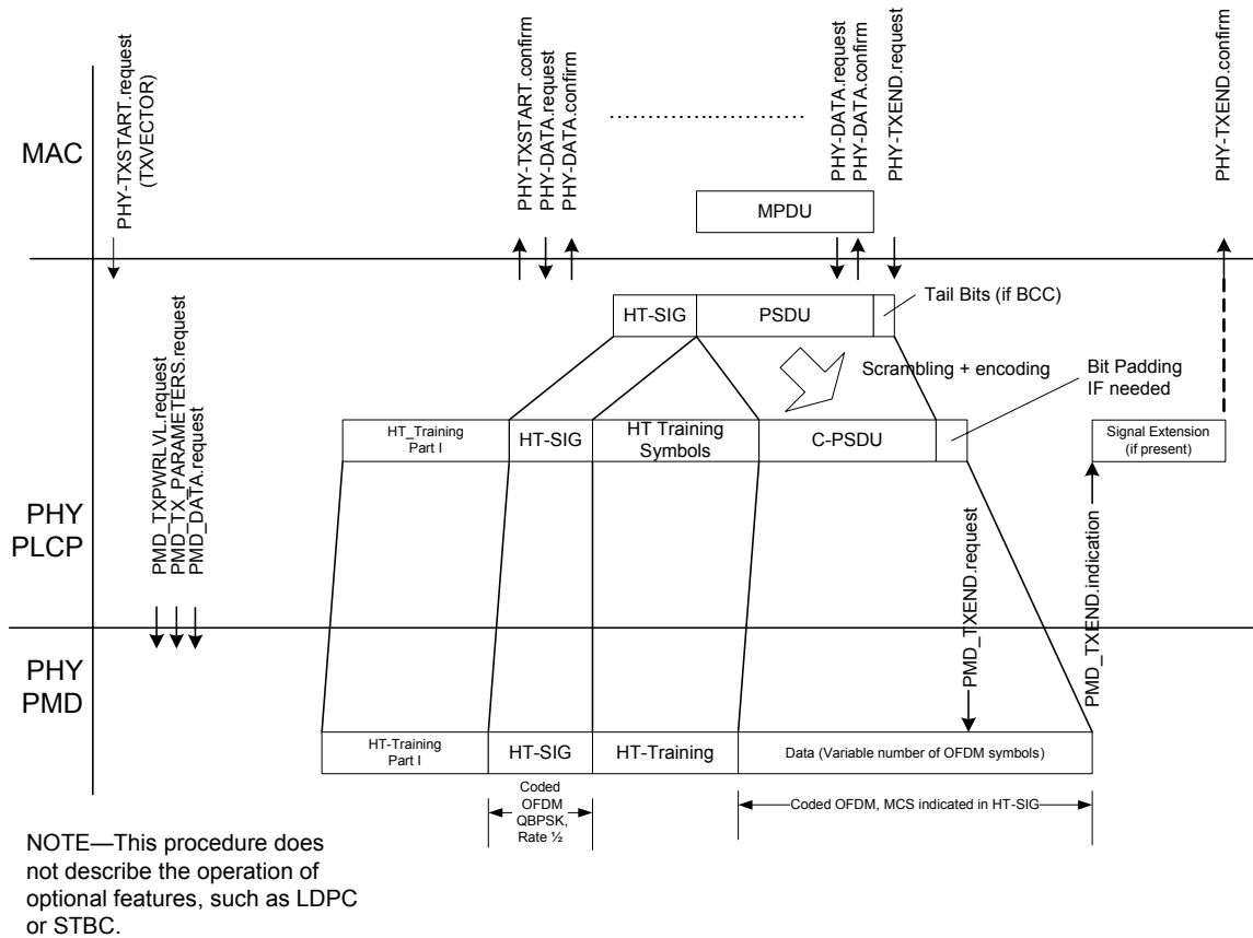
Figure 20-21—PLCP transmit procedure (HT-greenfield format PPDU)
