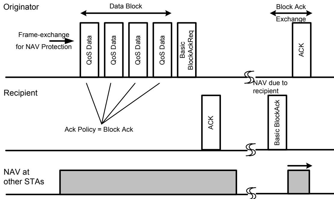
Figure 9-23—A typical BlockAck sequence when delayed policy is used
