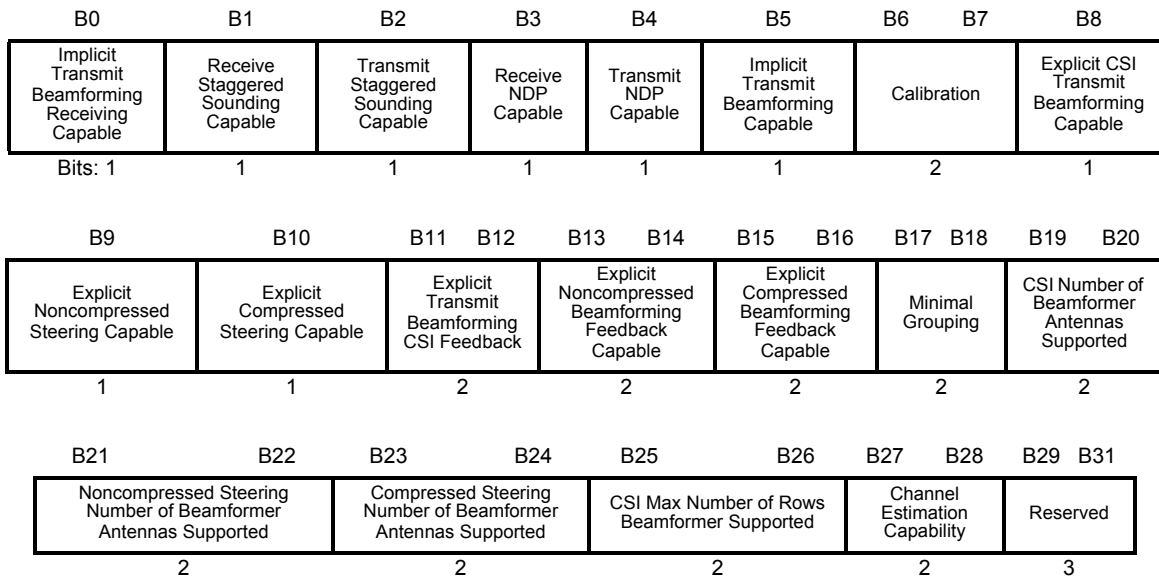
Figure 7-95o22—Transmit Beamforming Capabilities field
