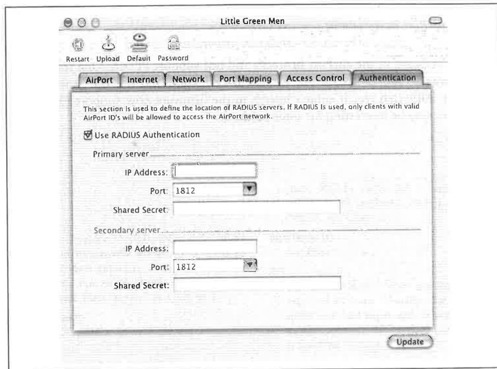
Figure B-15. RADIUS authentication tab
