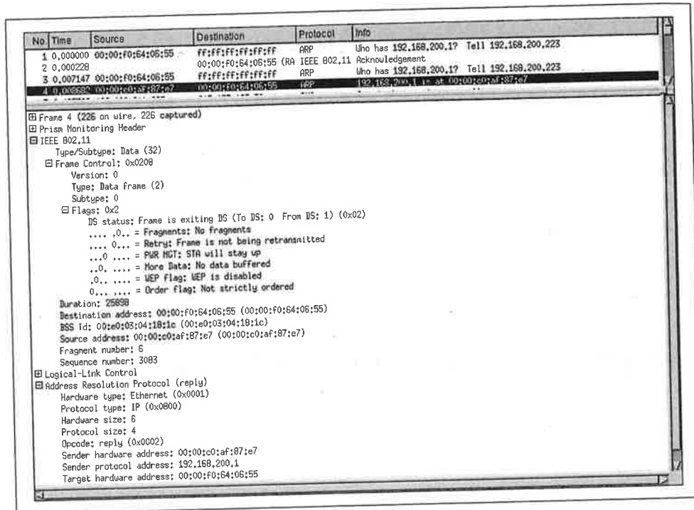
Figure 16-21. ARP reply
