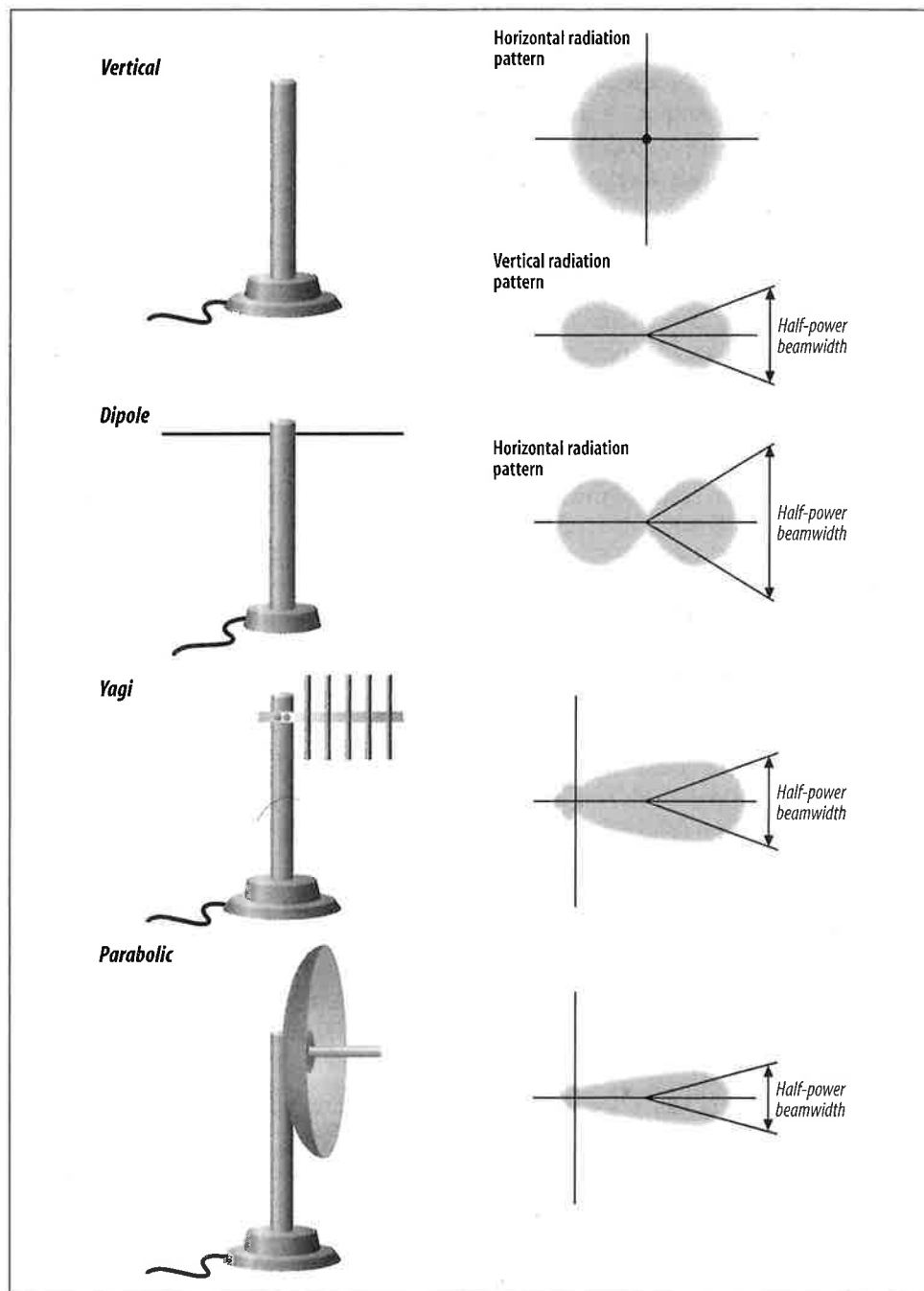
Figure 15-5. Antenna types
