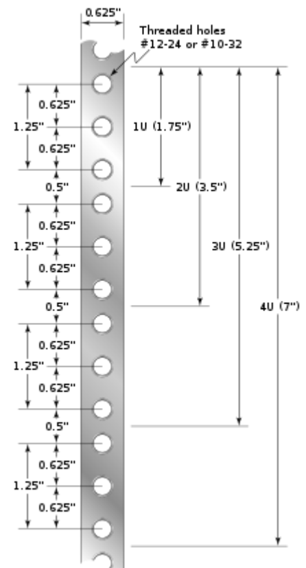
A typical section of rack rail, showing rack unit distribution
