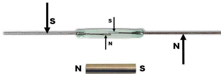
Figure 1 – Magnetic Induction
