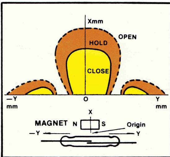
Figure 5 – Magnet Parallel to Reed Sw.
