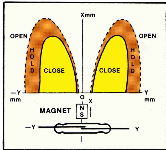
Figure 4 – Magnet Perpendicular to Reed Sw.
