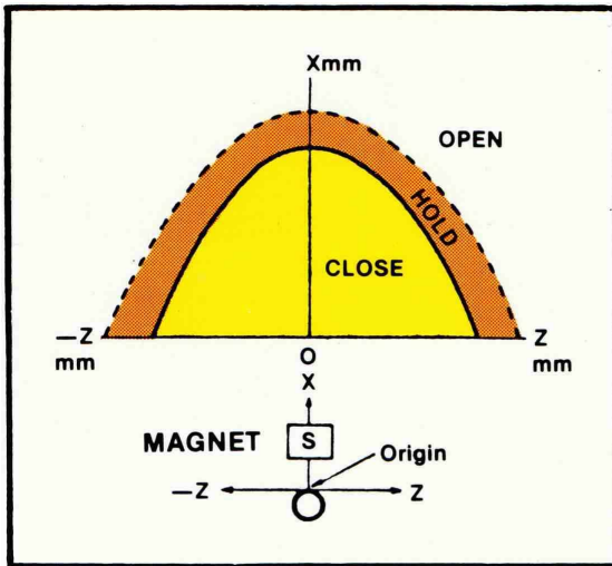
Figure 3 – Magnet Parallel to Reed Sw.
