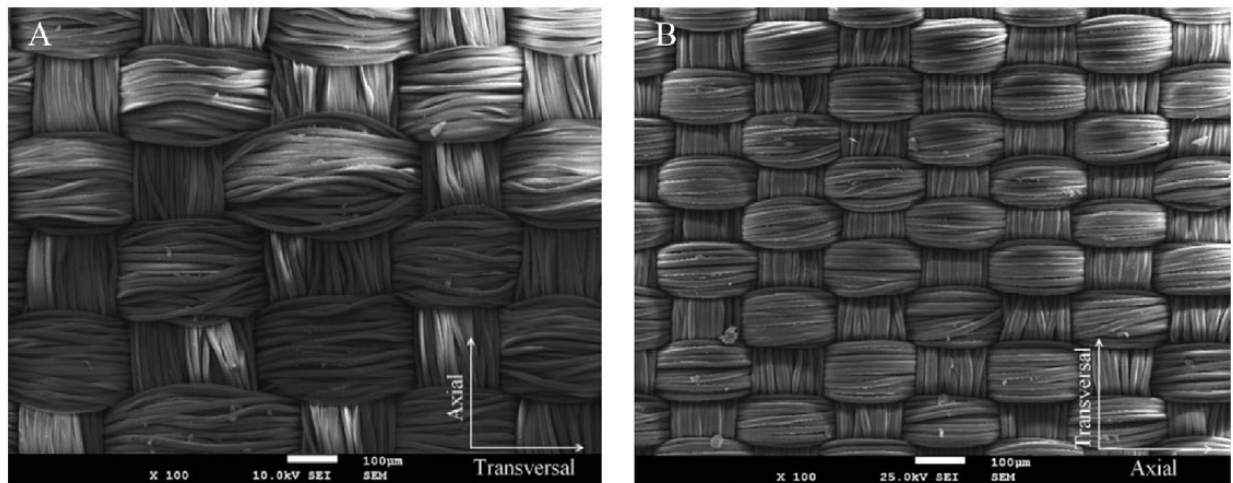
Fig. 8. Woven structures observed by SEM. (A) PET fabric; (B) PET-LP fabric.
