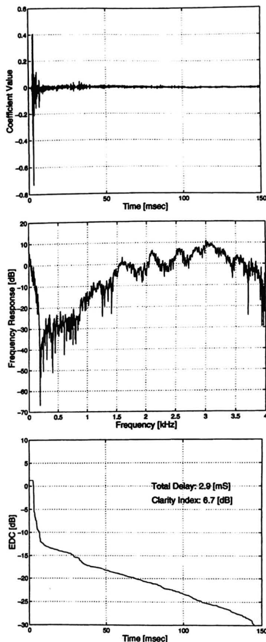
Fig. 6. (Top) Impulse response, (middle) frequency response, and (bottom) EDC of the TF between the speech loudspeaker and the first microphone.
