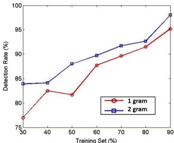
Fig. 7.7 Detection rate for permission based detection vs. Training set ratio (FNN with 10 nodes)
