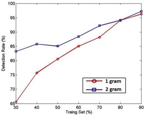
Fig. 7.9 Detection rate for permission based detection vs. Training set ratio (RNN with 10 nodes)
