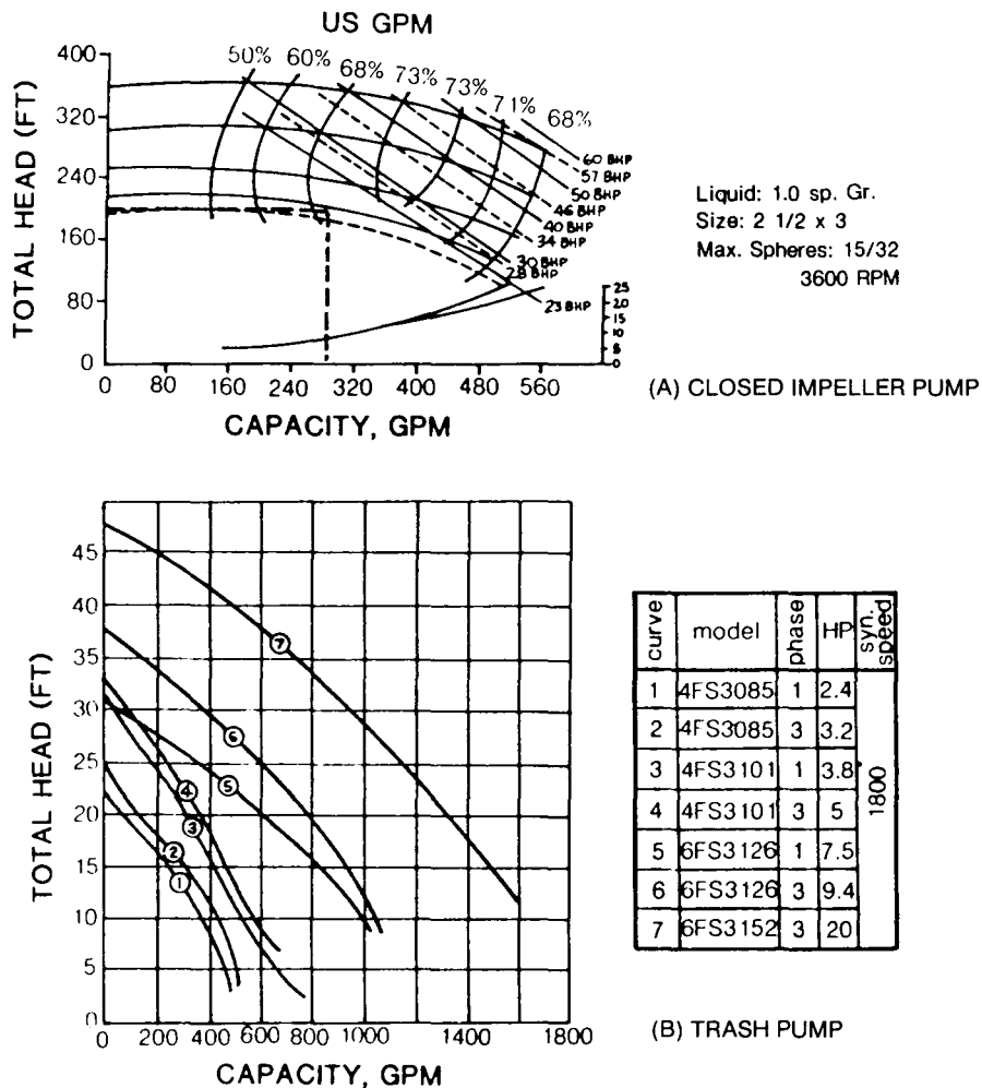
Figure 2. Example of typical performance curve for a closed impeller pump (A) and trash-type pump (B).
