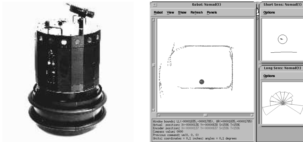
Figure 1: Left : The Manchester mobile robot Forty Two . The robot's sonar and infrared sensors are mounted on the turret. In all experiments the turret was kept fixed to provide a "compass sense". Exploration was carried out using the separate translational and rotational motors located in the base of the robot right : The Nomad simulator.
