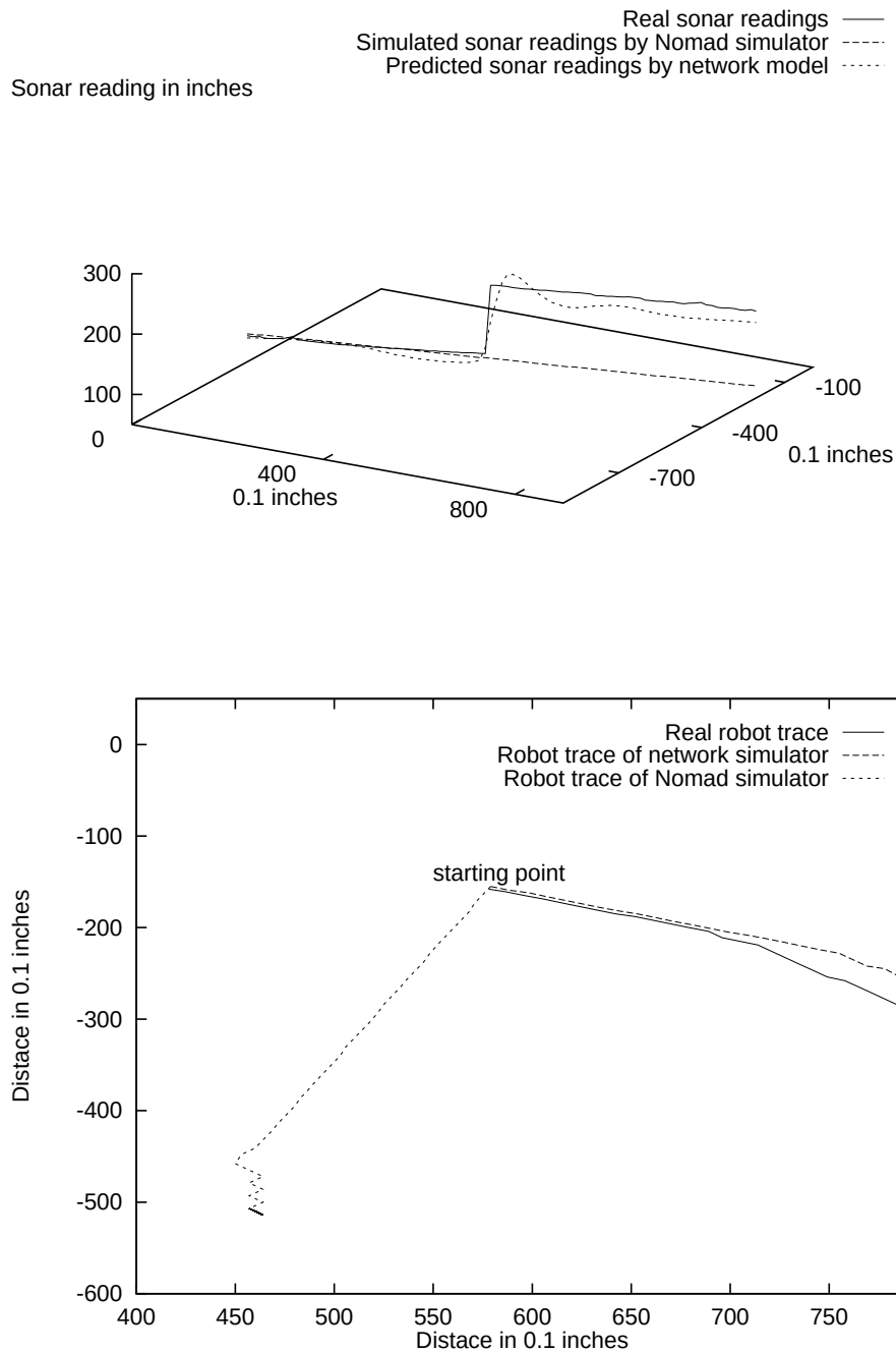
Figure 3: Top : Sonar reading predictions. The Nomad simulator is unable to predict the sudden increase in sonar reading due to specular reflection, while the network simulator predicts this correctly. Bottom : Simulated and real robot trajectories in response to the “find free-est space” program. The real and network-simulated robot bump into a smooth wall while the Nomad-simulated robot goes to the geometrical centre of the robot’s environment at (450,-450).
