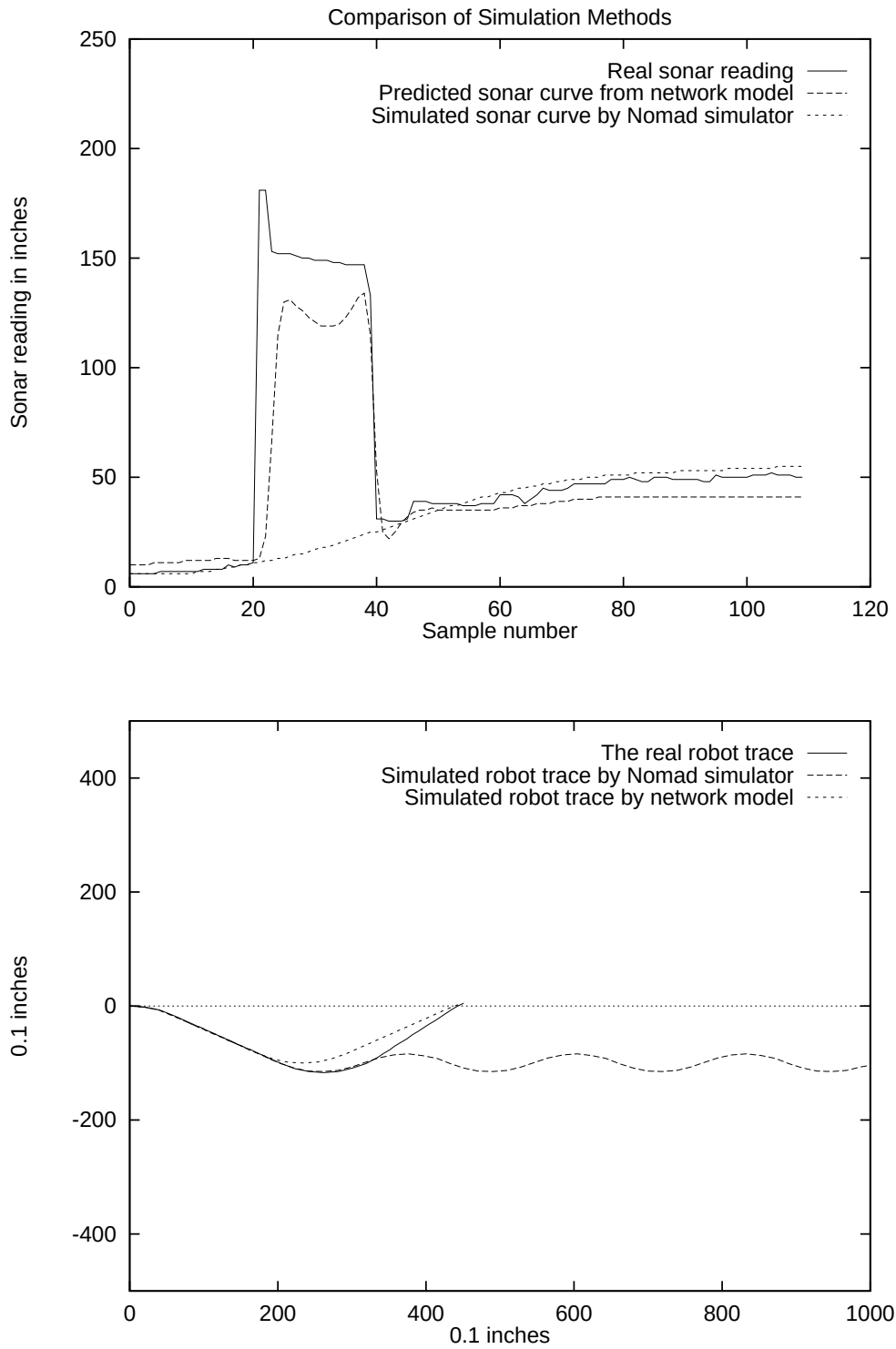
Figure 2: top : The network model successfully predicts the sudden changes in sonar readings between sample 20 and 40, which the Nomad model fails to do. Bottom : By assuming a homogeneous wall surface, the Nomad simulator fails to predict the collision of the real robot, caused by specular reflections. The network simulator correctly predicts the collision.
