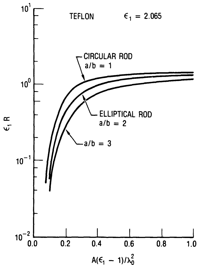
Fig. 1. Configuration Loss Factor \epsilon_1 R as a Function of Normalized Frequency for an Elliptical Teflon Rod Supporting the Dominant {}^e\text{HE}_{11} Mode. A is the cross-sectional area, \lambda_0 is the free-space wavelength, a is the semi-major axis of the elliptical rod, and b is the semi-minor axis. Note that flatter rod yields smaller configuration loss factor for the same cross-sectional area.
