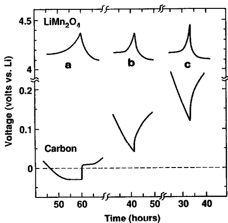
Fig. 6. Voltage profiles vs. Li (as measured from a three electrode cell) of \text{LiMn}_2\text{O}_4 and carbon electrodes at the end of the first charge and the beginning of the first discharge with different ratios r = 3.1 (a), r = 2.1 (b) and r = 1.7 (c). For these experiments the mass of the carbon electrode was maintained constant (30 mg), the electrolyte used was \text{EC} + \text{DEE} (50:50) + 1 \text{ M LiClO}_4 and the current rate was 0.4 \text{ mA cm}^{-2} .
