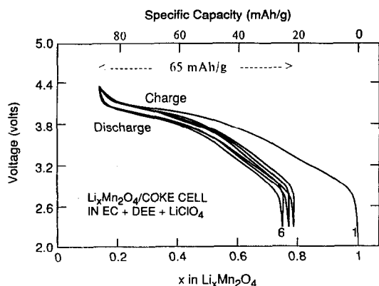
Fig. 8. Cycling behavior at room temperature of a \text{LiMn}_2\text{O}_4/\text{EC} + \text{DEE}(50:50) + 1\text{ M LiClO}_4/\text{C} rocking-chair cell at a rate of C/10 with the mass of the positive electrode being 2.1 times that of the negative electrode.
