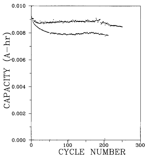
Fig. 7. Capacity vs. cycle number for \text{LiNiO}_2/\text{coke} 1225 coin cells discharged through 1 and 3\text{ k}\Omega resistors. The lower capacity data are for the 3\text{ k}\Omega load. The cell voltage remains below 0.1\text{ V} for 10\text{ h} before each recharge (see text).
