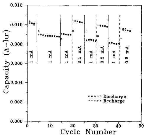
Fig. 10. Capacity vs. cycle number for LiNiO 2 /coke 1225 coin cells with 30 day storage periods after every 10 cycles. The storage periods occurred after each vertical bar in the graph. The cycling currents are indicated in the figure. The cells were cycled between 3.9 and 2.5 V.
