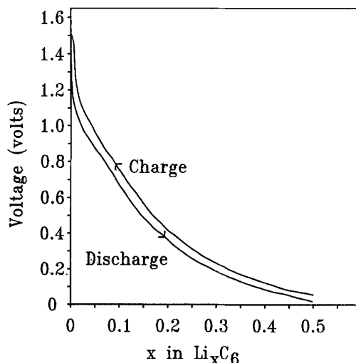
Fig. 3. Voltage of \text{Li}/\text{Li}_x\text{C}_6 cells vs. x for the second discharge and charge of the cell. The carbon in the positive electrode is petroleum coke. The current was chosen so that a change \Delta x = 1 occurred in 80 h.
