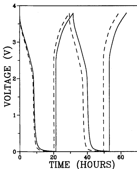
Fig. 6. Voltage vs. time for a \text{LiNiO}_2/\text{coke} 1225 coin cell discharged through a 3\text{ k}\Omega load and then charged to 3.8\text{ V} . The 10th, 11th (solid), and 110th, and 111th (dashed) cycles are shown. The cell was at 21^\circ\text{C} .
