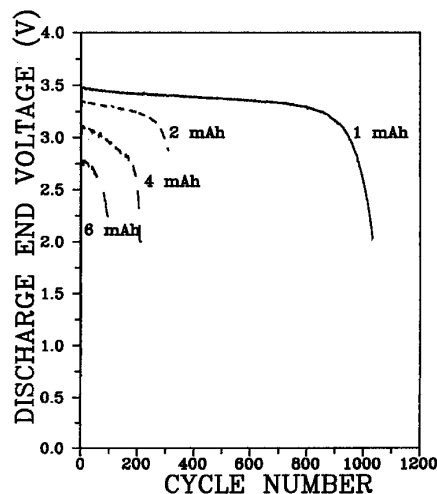
Fig. 9. End of discharge voltage vs. cycle number for constant capacity discharges ( 1.0\text{ mA} ) at 85^\circ\text{C} . The \text{LiNiO}_2/\text{coke} cells were charged to 3.7\text{ V} at 1.0\text{ mA} following each discharge. Four cells were tested using discharge capacities of 1, 2, 4, and 6 mAh.
