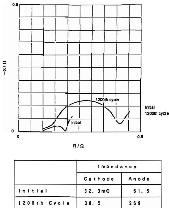
Fig. 18. Impedance spectra of electrodes at initial and after 1200 cycles.
