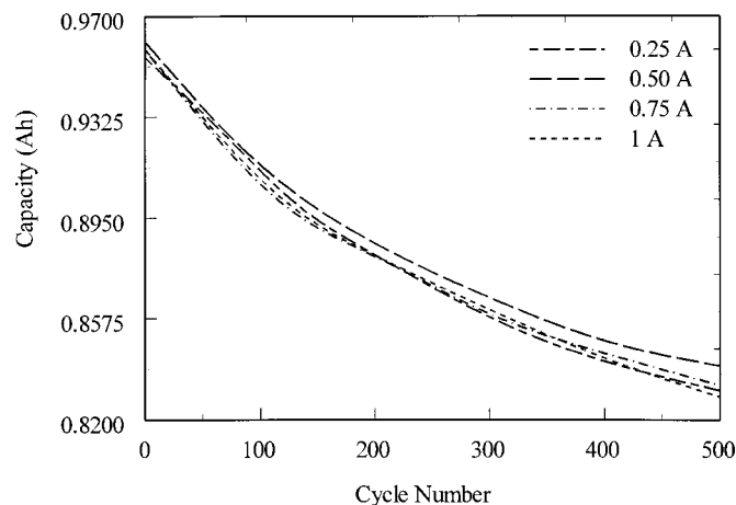
Figure 5. Capacity fade of Li-ion cells charged at different currents.
