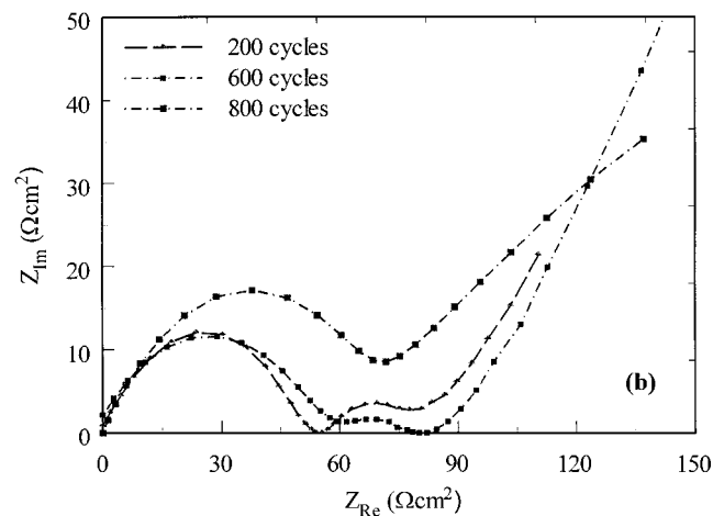
Figure 9. Nyquist plots obtained using a T-cell at discharged state for carbon (a, top) and spinel (b, bottom).
