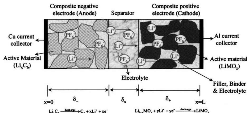
Fig. 1. Schematic diagram of a lithium-ion cell on discharge.
