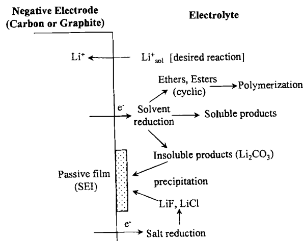
Fig. 5. The complexity of the intercalation process in the negative electrode.
