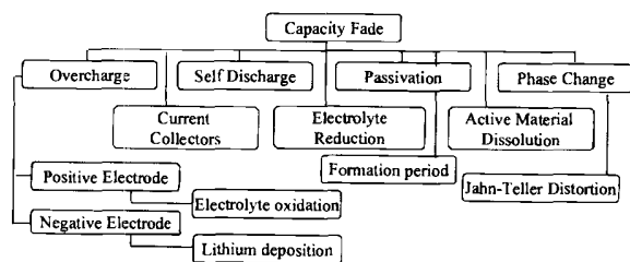
Fig. 2. Flow chart describing various capacity fade phenomena in lithium-ion batteries.
