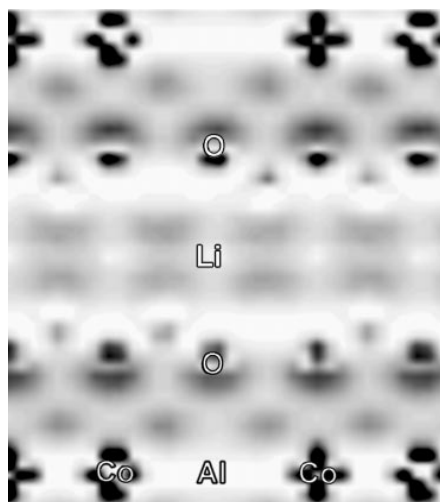
Figure 1 Positive part of the electron density difference between Li(Al 0.33 Co 0.67 )O 2 and (Al 0.33 Co 0.67 )O 2 in a plane perpendicular to the direction of layering in the structure. Darker indicates larger electron density.
