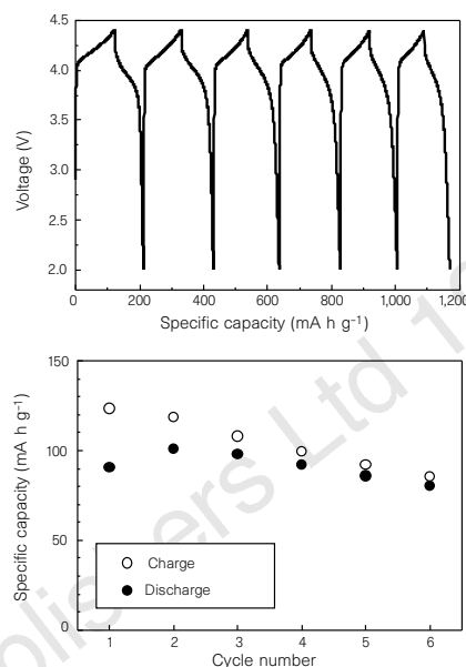
Figure 3 Cycling behaviour of \text{Li}(\text{Al}_{0.25}\text{Co}_{0.75})\text{O}_2/\text{Li} and specific capacity between 2.0 and 4.4 V. The current density was 0.4\text{ mA cm}^{-2} .
