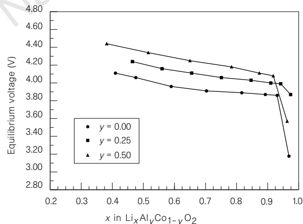
Figure 2 Open-circuit potential as a function of lithium content in pure \text{LiCoO}_2 and in Al-doped materials.
