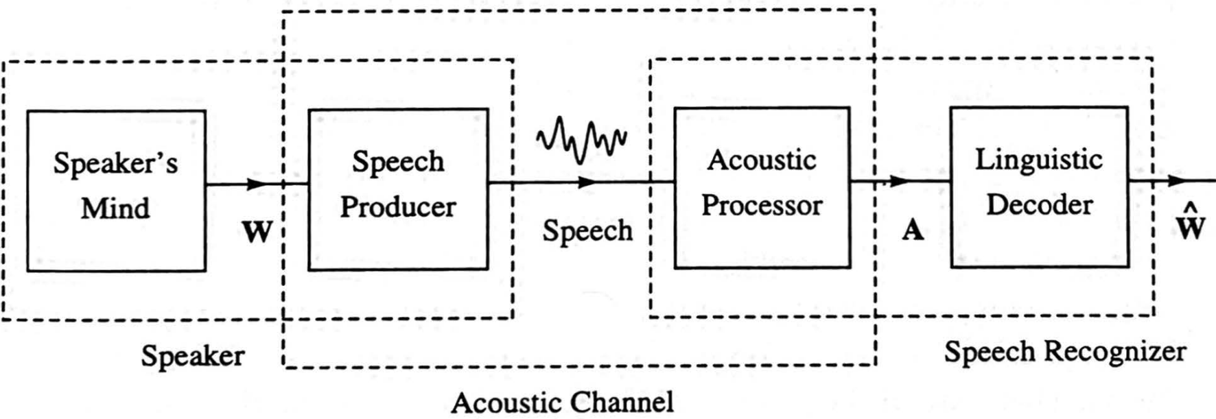
Figure 1.3 Source-channel model of speech recognition
