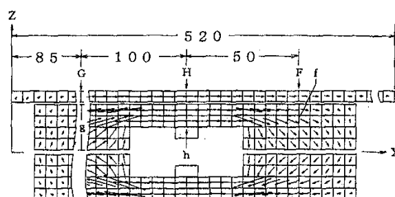
Fig. 7 Flux density plot of the coupler.
