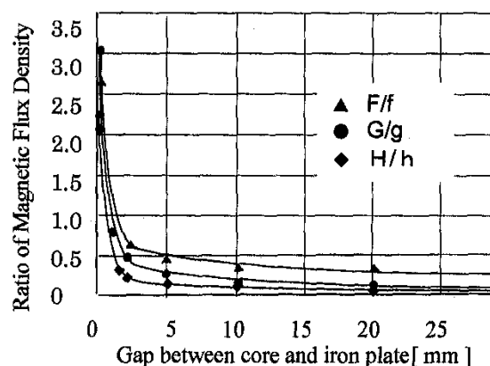
Fig. 8 Magnetic flux densities ratio.
