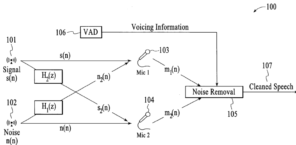
Figure 1 is a block diagram of the noise removal system. Ex. 1001, 2:23–25. Microphones Mic 1 and Mic 2 receive acoustic information from speech signal source 101 and noise source 102, and the acoustic information received at each microphone is provided to Noise Removal system 105. Id.
