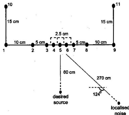
FIG. 5. Experimental configuration.
