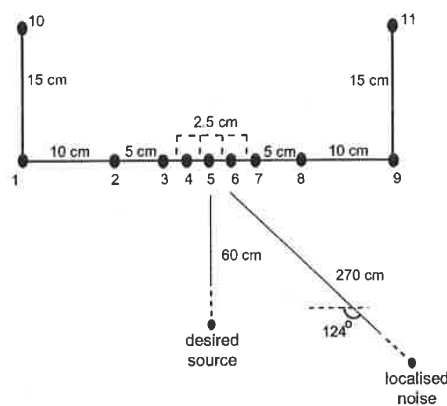
FIG. 5. Experimental configuration.
