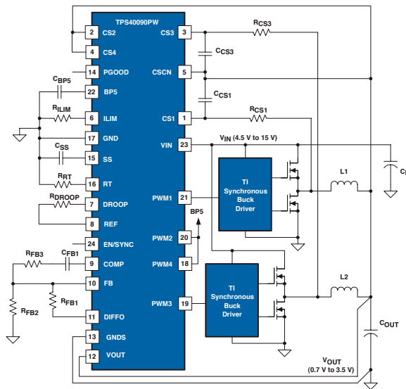
Simplified two-phase application diagram.
