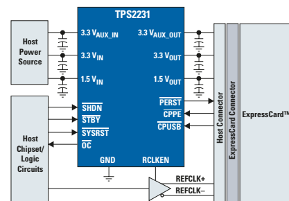
Typical ExpressCard™ power-distribution application.
