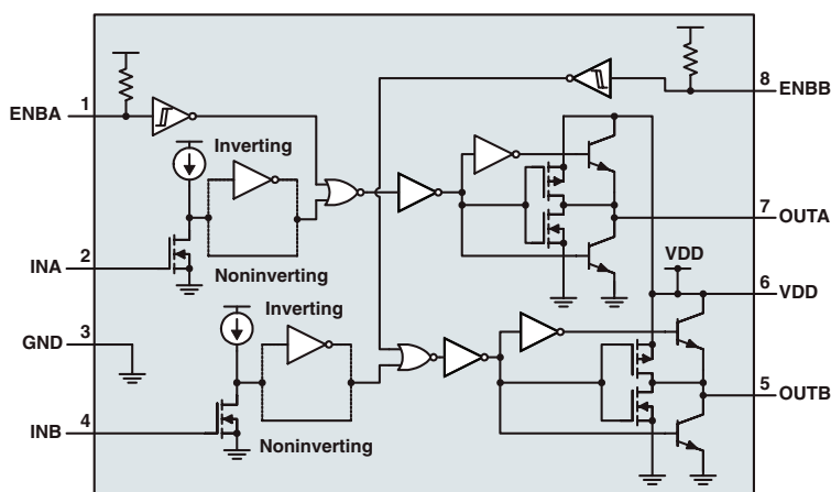
UCC27423/24/25 block diagram.
