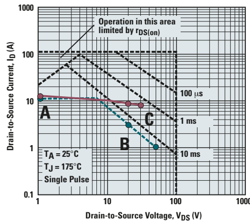
Safe operating area of a power FET.
