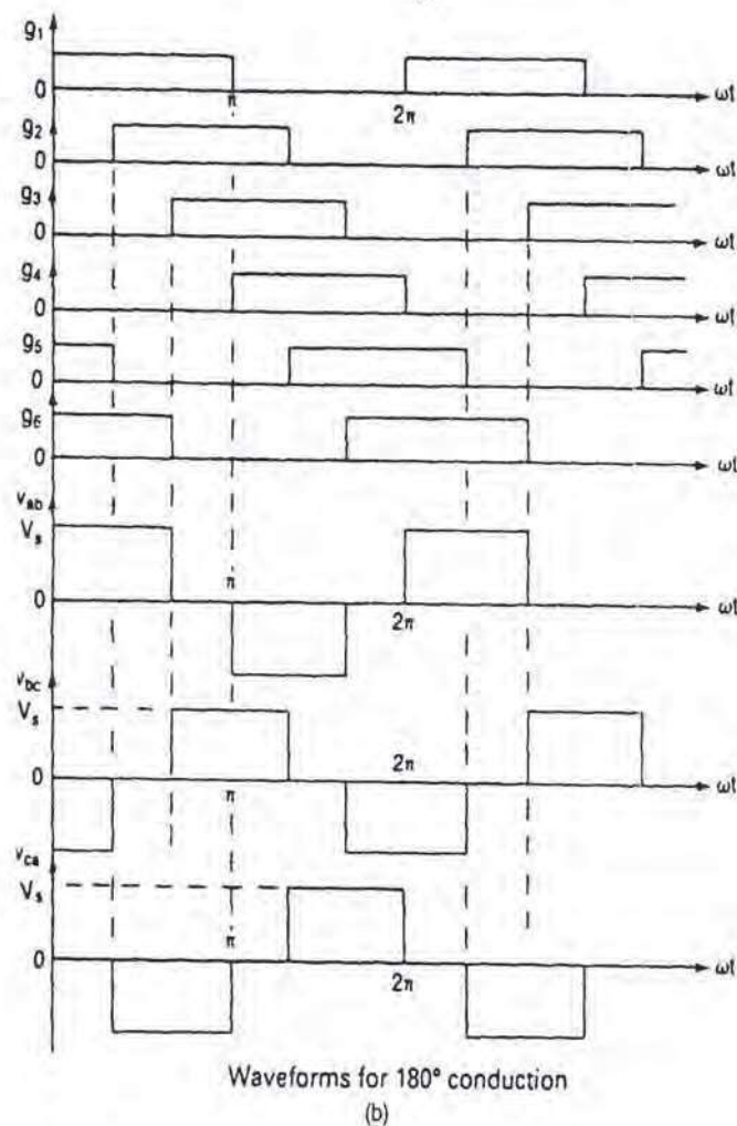
FIGURE 30.8 Three-phase voltage-controlled inverter operation.
