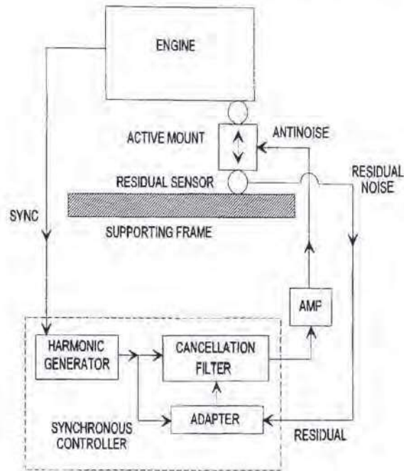
FIGURE 31.6 An active engine mount.
