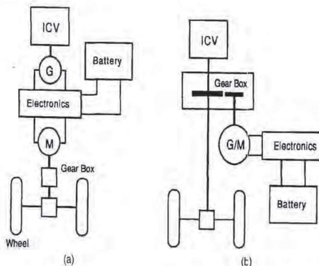
FIGURE 30.13 Two conceptual arrangements for hybrid vehicles: (a) series hybrid drive; (b) parallel hybrid drive.
