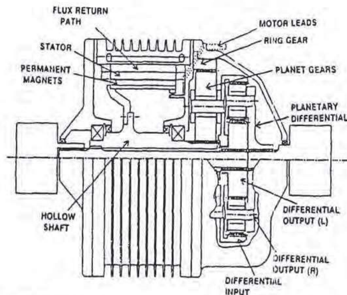
FIGURE 30.9 Integrated transaxle motor, gear, and differential arrangement. 8
