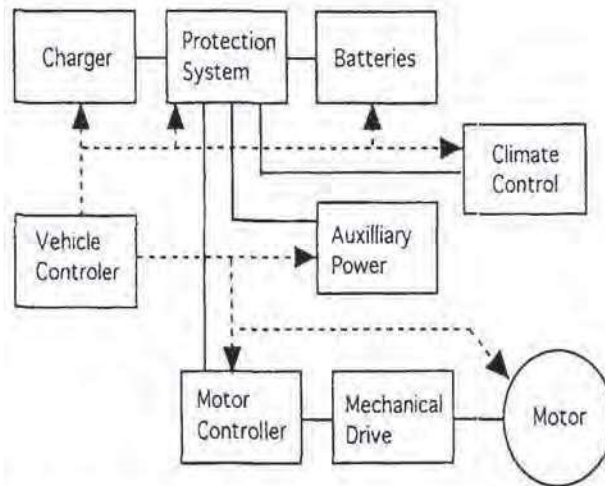
FIGURE 30.1 System-block diagram of a typical electric vehicle (EV).
