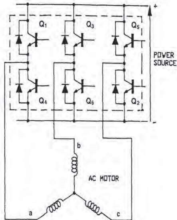
FIGURE 30.7 Concept of ac motor regulation.
