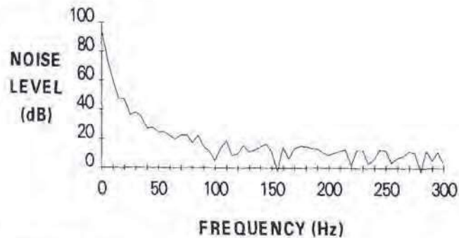
FIGURE 31.1 A typical broadband noise spectrum.
