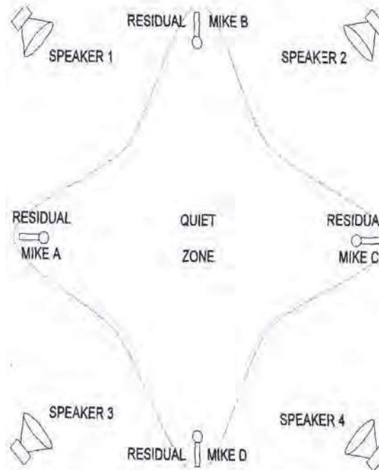
FIGURE 31.7 Zonal noise control for an automobile.
