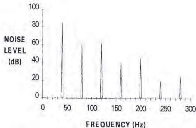
FIGURE 31.2 A typical narrowband noise spectrum.
