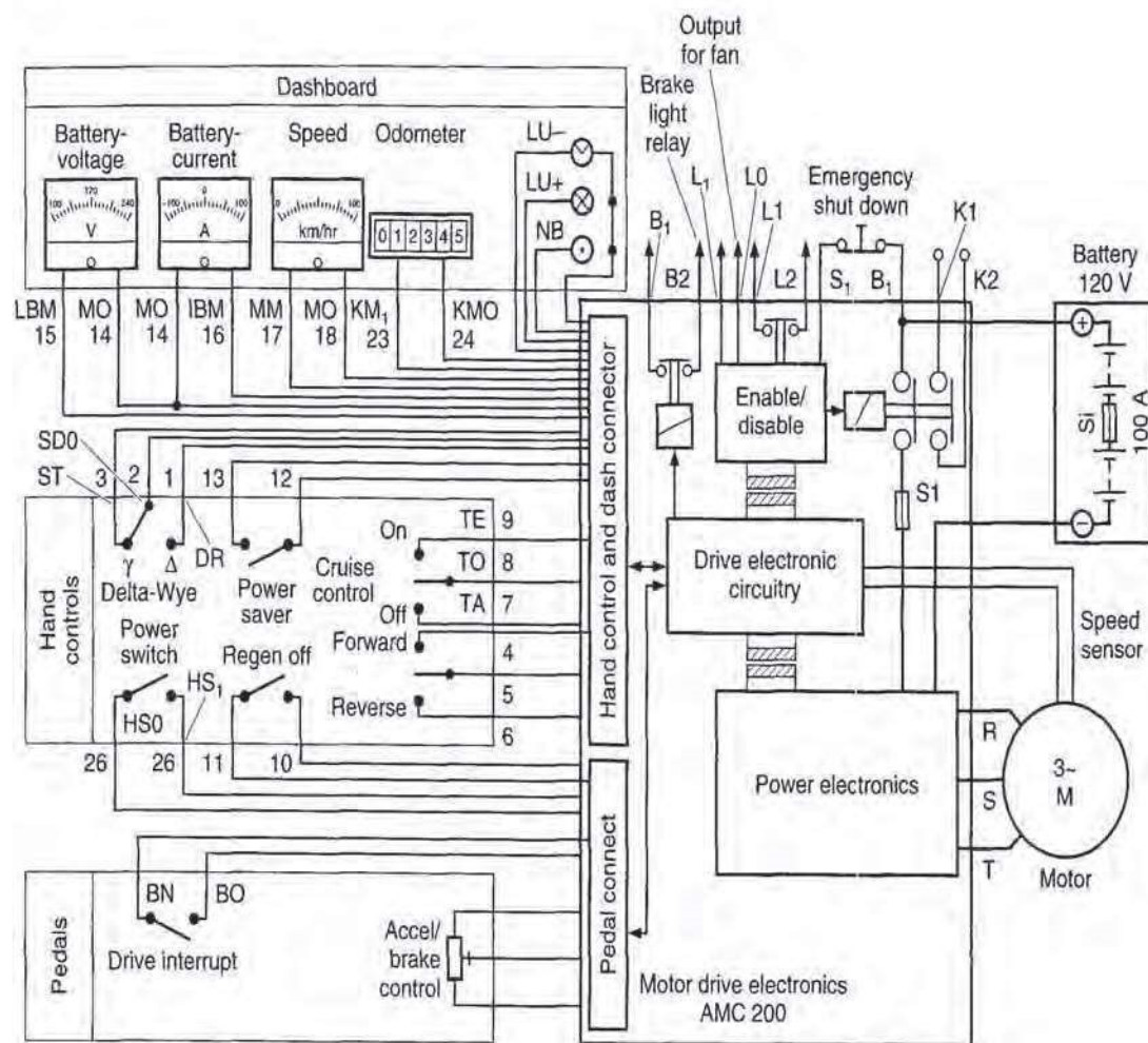
FIGURE 30.10 An electric vehicle control system.
