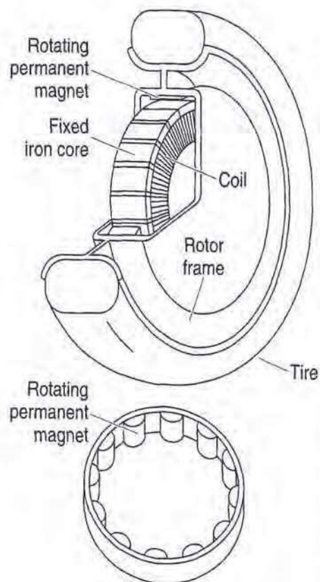
FIGURE 30.4 In-wheel brushless dc electric motor. (Courtesy of Tokyo Electric Power Co.)
