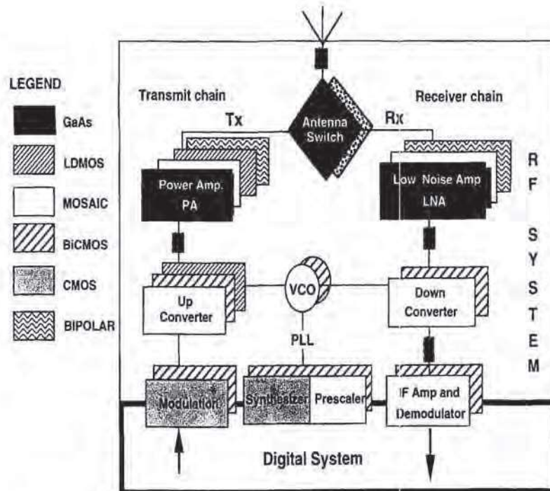
FIGURE 32.6 RF semiconductor technologies.
