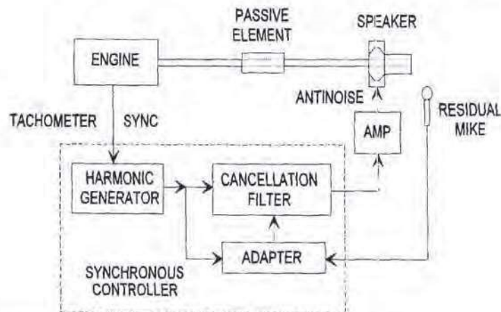
FIGURE 31.5 Narrowband noise cancellation (an active muffler).
