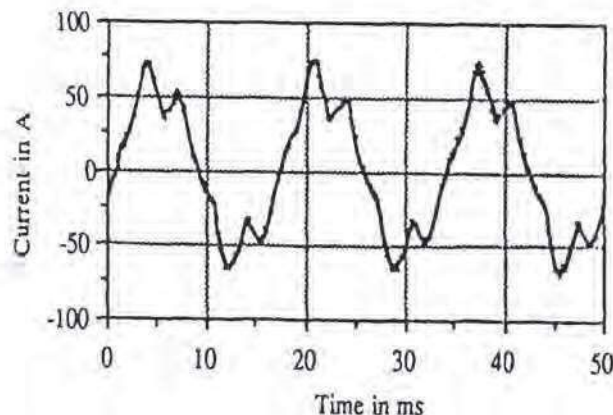
FIGURE 30.12 Charging current waveform at a slow-charging station. 11
