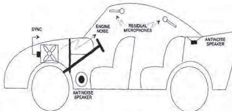
FIGURE 31.8 An automobile cabin-quieting system.
