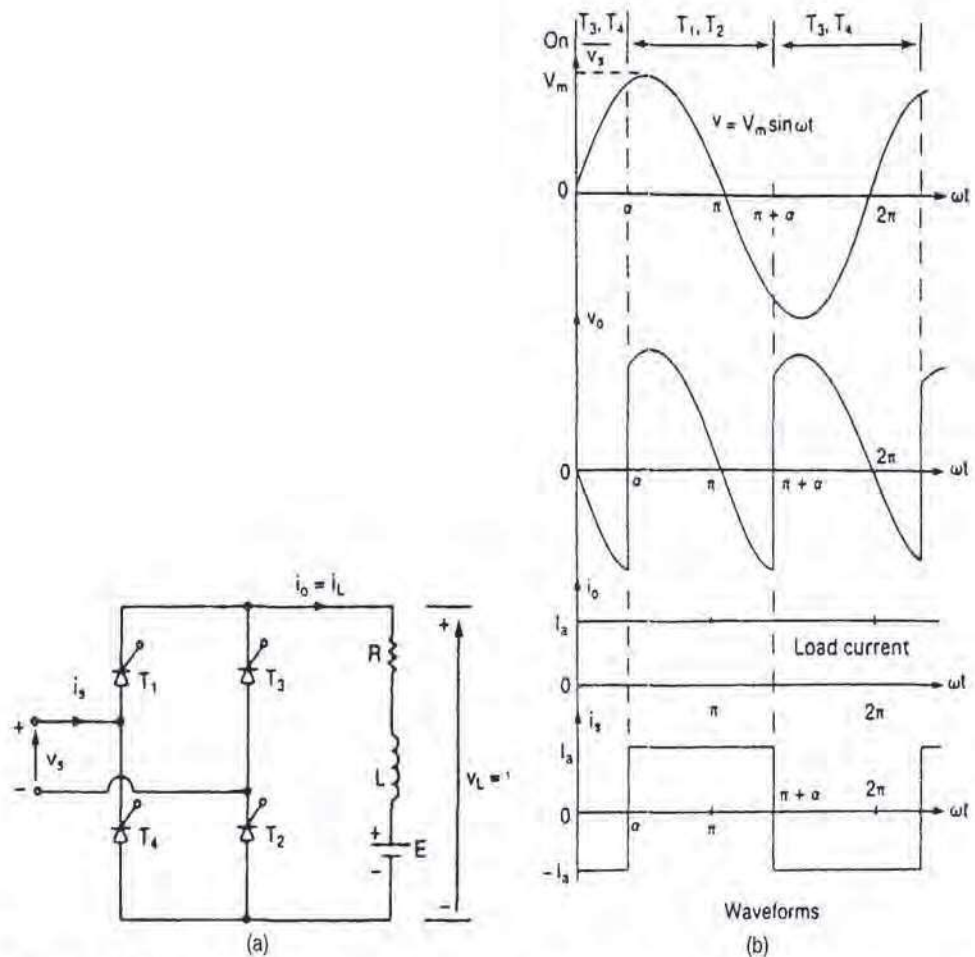
FIGURE 30.2 Thyristor-controlled battery charger: (a) connection diagram; (b) current and voltage waveforms.
