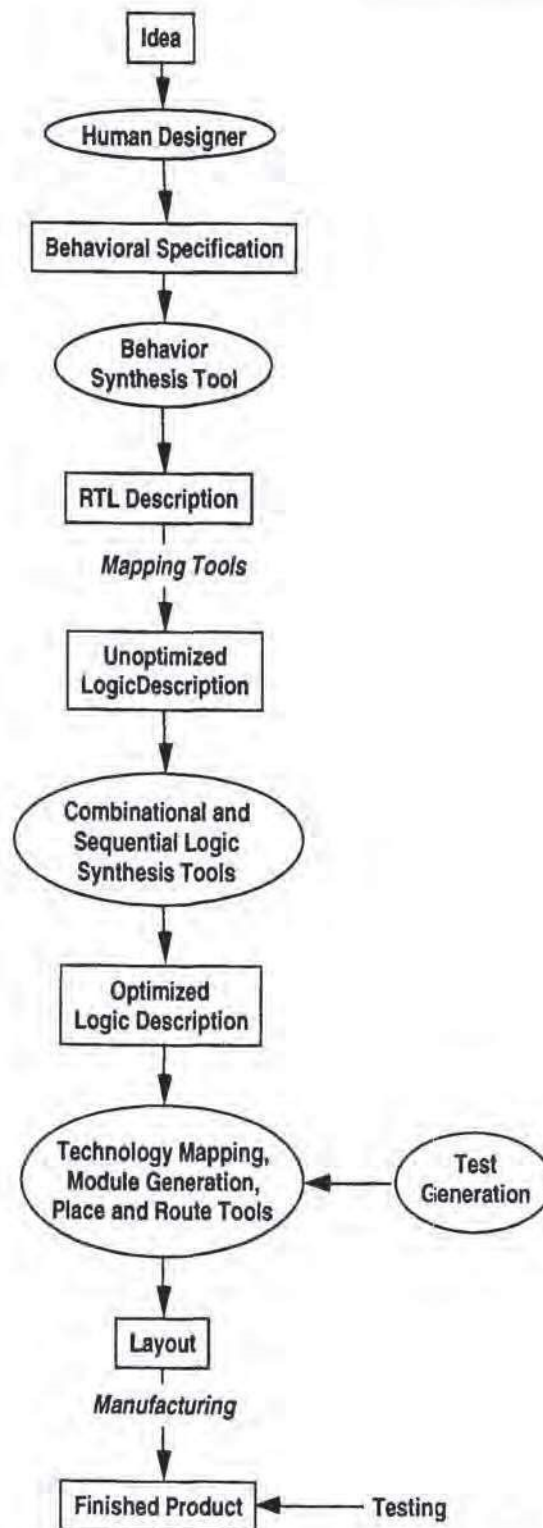
FIGURE 32.10 Typical synthesis pipeline of today's design of VLSI silicon chip.
