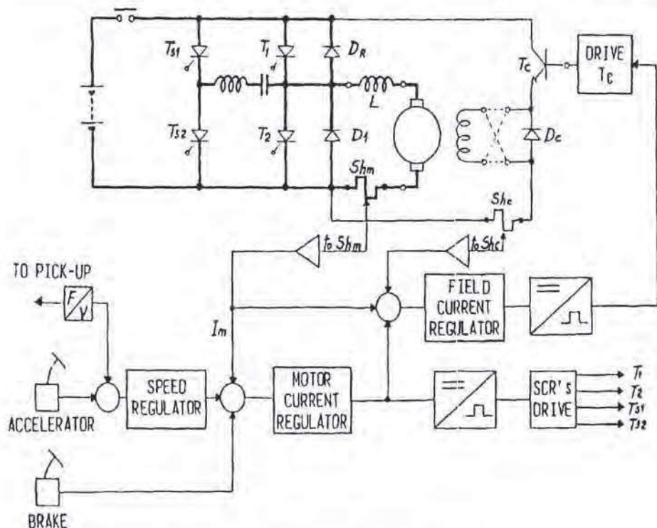
FIGURE 30.6 Double chopper for separately excited dc commutator motor.
