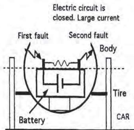
FIGURE 30.3 Effect of insulation faults in an EV.
