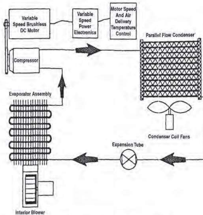
FIGURE 30.11 An EV advanced air conditioning system. 10
