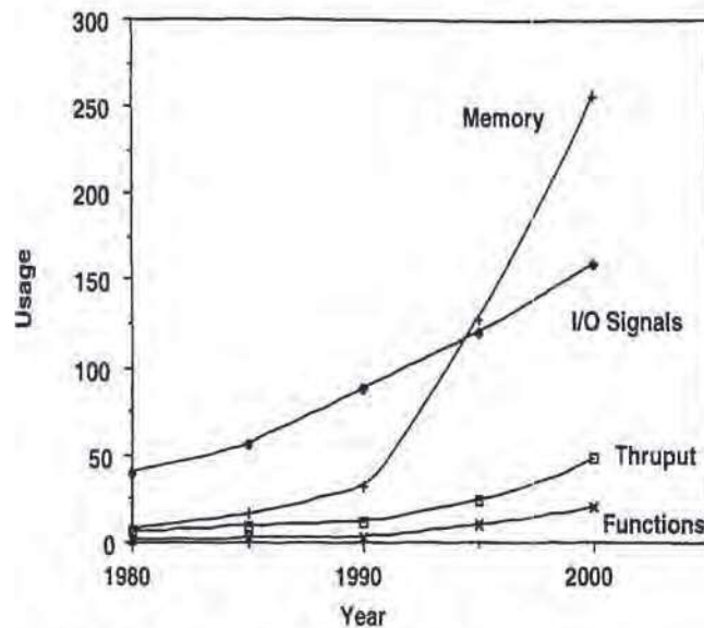
FIGURE 32.2 Automotive usage of microcontroller technology.
