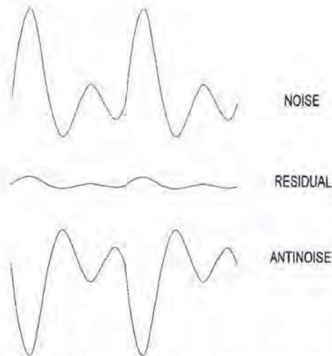
FIGURE 31.3 Relationships in time among noise, antinnoise, and residual noise.
