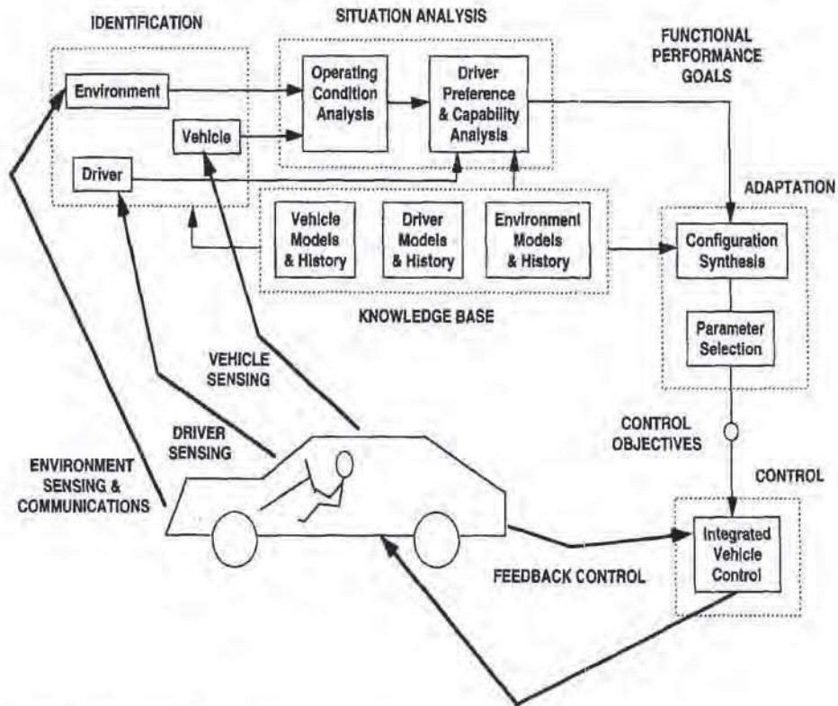
FIGURE 32.8 Vehicle, driver, and environment interrelationships.
