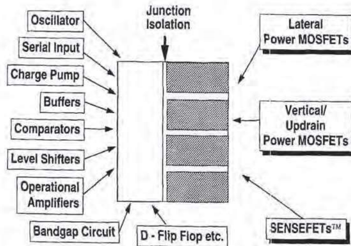
FIGURE 32.5 SMARTMOS™ technology cells.
