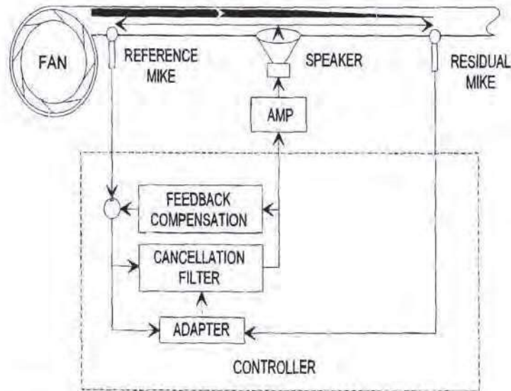
FIGURE 31.4 Feed forward cancellation system.
