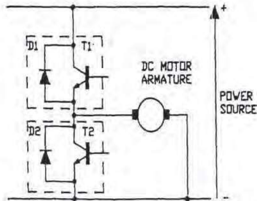
FIGURE 30.5 Concept of a commutator-type series dc motor drive.
