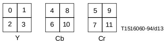
Figure 6-12 – 4:4:4 Macroblock structure
