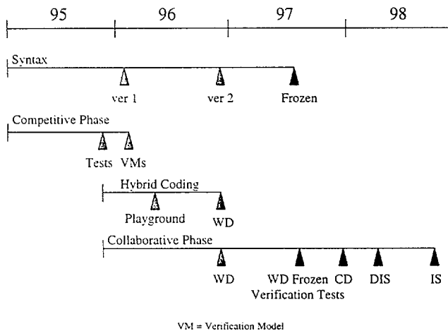
Fig. 6 MPEG4 workplan.
