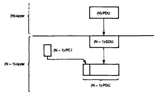
Fig. 7. Interrelationship between data units.
