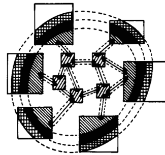
Fig. 2. Network layering.
