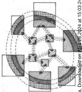
Fig. 2. Network layering.
