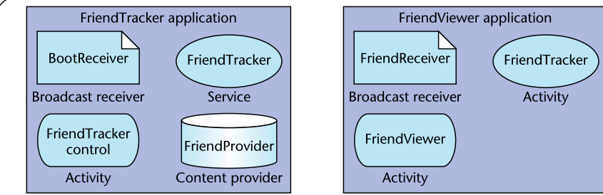
Figure 1. Example Android application. The FriendTracker and FriendViewer applications consist of multiple components of different types, each of which provides a different set of functionalities. Activities provide a user interface, services execute background processing, content providers are data storage facilities, and broadcast receivers act as mailboxes for messages from other applications.
