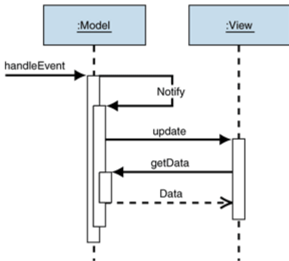
Figure 4: Behavior of the active model
