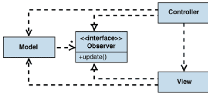
Figure 3: Using Observer to decouple the model from the view in the active model
