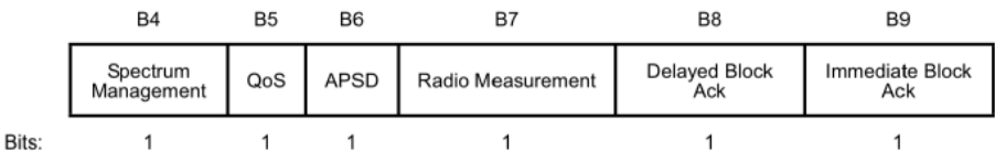
Figure 9-297—Capabilities subfield
