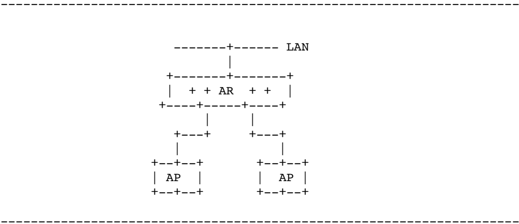
Figure 2: Directly Connected
