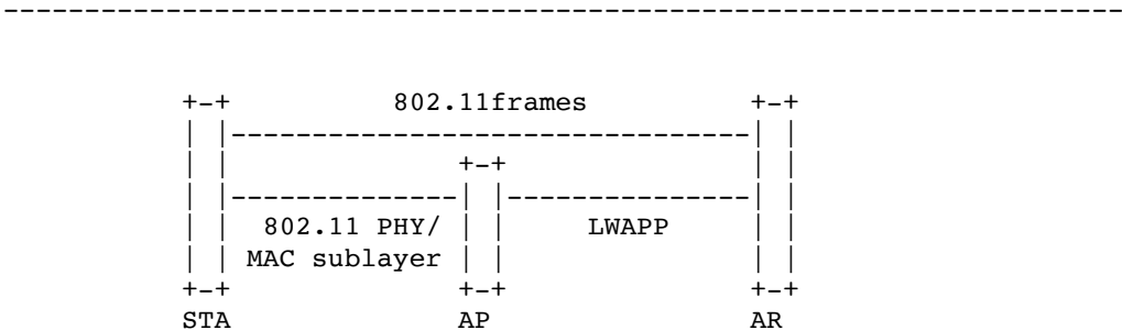
Figure 1: LWAPP Architecture
