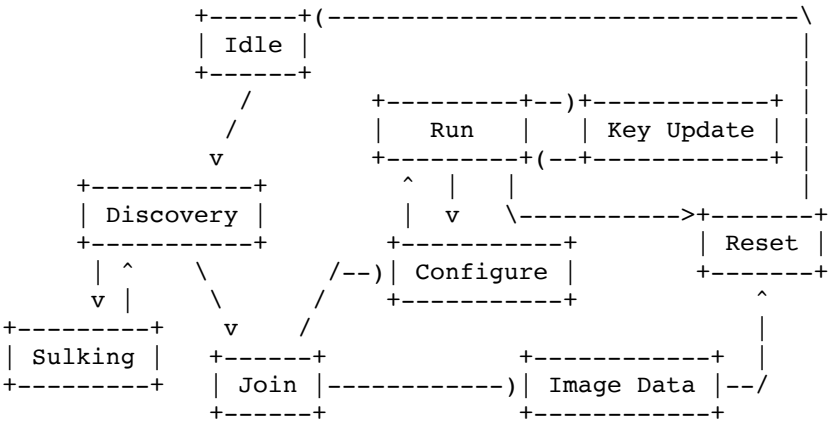
Figure 3: LWAPP State Machine
