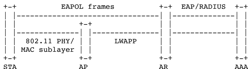
Figure 2: 802.1X Authentication in the AR
