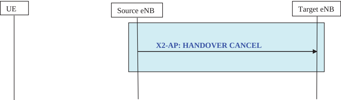
Figure 20.2.2-1: Handover Cancellation procedure
