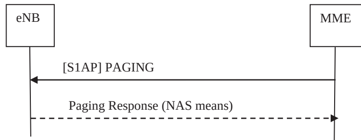
Figure 19.2.2.1-1: Paging procedure
