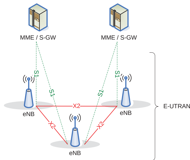
Figure 4-1: Overall Architecture
