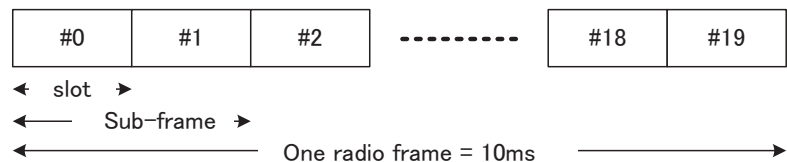
Figure 5-1: Frame structure type 1
