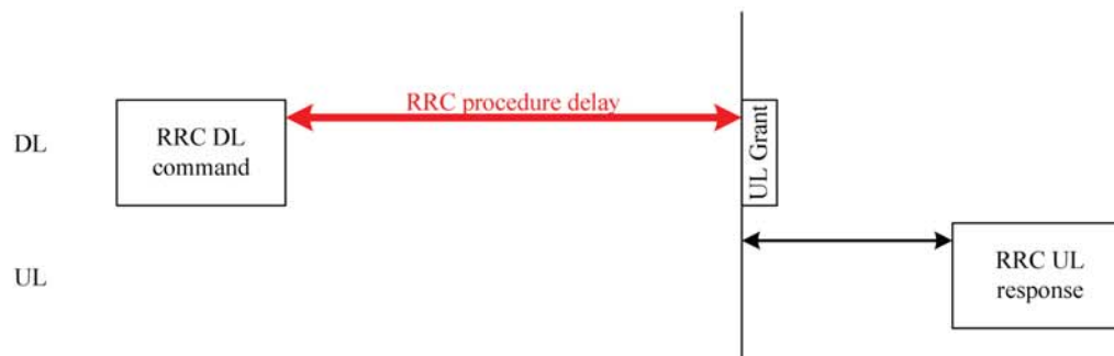
Figure 11.2-1: Illustration of RRC procedure delay
