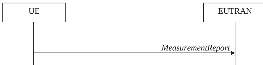
Figure 5.5.5-1: Measurement reporting
